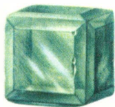
crystal
