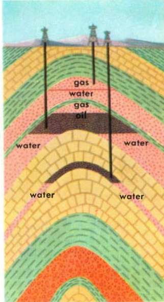
WELL FIELD producing gas from the upper zone, oil and gas from the middle zone, and oil below.
