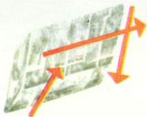
Rhombohedral cleavage: calcite
