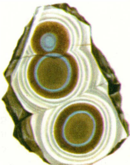
EYE AGATE—Brazil
