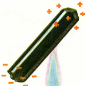
Heated tourmaline develops electric charges
