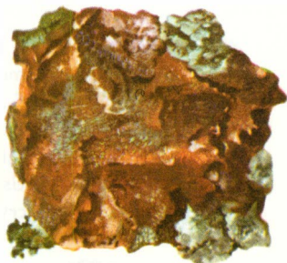
NATIVE COPPER—Michigan
