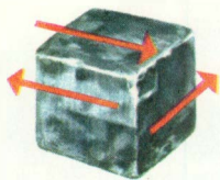
Cubic cleavage: galena
