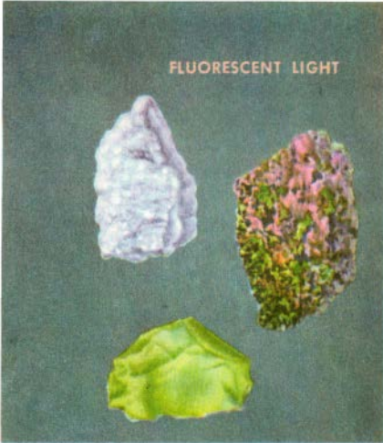
SCHEELITE
