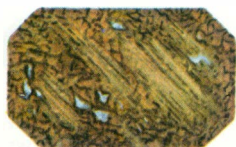
JASPER—Montana
