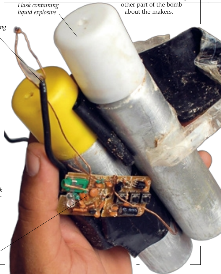
Circuit board triggers bomb when cell phone signal is received
