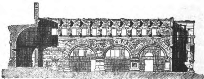
FIG. 84. — Longitudinal section of basilica in Ruweha, Syria.
