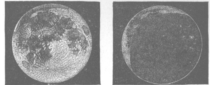
Fig 158. The Full moon.
