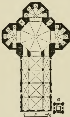
FIG. 147.—DUOMO AT FLORENCE. PLAN.
