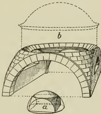
FIG. 71.—DIAGRAM OF PENDENTIVES.
