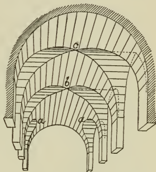
FIG. 109.—PENETRATIONS AND INTERSECTIONS OF VAULTS.
