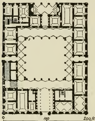
FIG. 167.—PLAN OF FARNESE PALACE.
