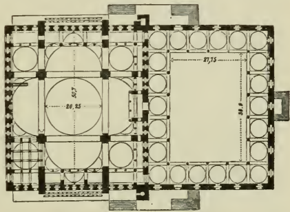
FIG. 87.—MOSQUE OF MEHMET II., CONSTANTINOPLE. PLAN.
