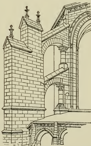
FIG. 107.—EARLY GOTHIC FLYING BUTTRESS.
