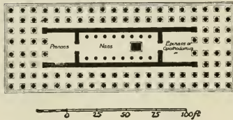
FIG. 39.—TEMPLE OF OLYMPIAN ZEUS, ATHENS.
