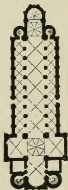
FIG. 99.—PLAN OF MINSTER AT WORMS.
