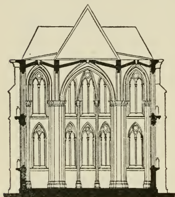
FIG. 140.—SECTION OF ST. ELIZABETH, MARBURG.
