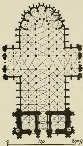
FIG. 141.—COLOGNE CATHEDRAL. PLAN.
