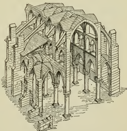
FIG. 105.—CONSTRUCTIVE SYSTEM OF GOTHIC CHURCH. ILLUSTRATING PRINCIPLES OF ISOLATED SUPPORTS AND BUTTRESSING.
