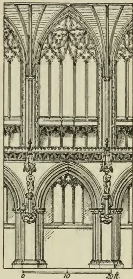
FIG. 135.—ONE BAY OF CHOIR, LICHFIELD CATHEDRAL.
