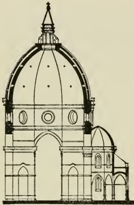
FIG. 159.—SECTION OF DOME OF DUOMO, FLORENCE.
