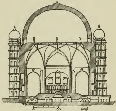
FIG. 85.—TOMB OF MAHMUD, BIJAPUR. SECTION.
