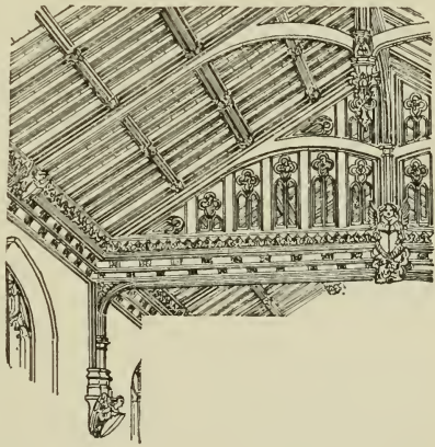
FIG. 138.—ROOF OF NAVE, ST. MARY'S, WESTONZOYLAND.
