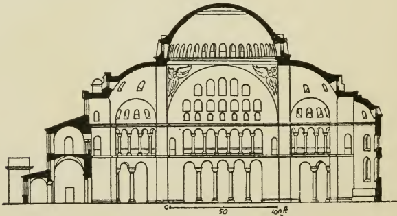
FIG. 76.—SECTION OF HAGIA SOPHIA.
