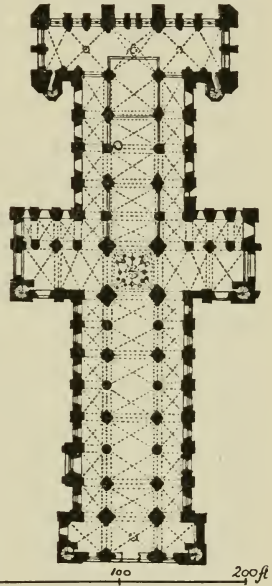
FIG. 102.—PLAN OF DURHAM CATHEDRAL.
