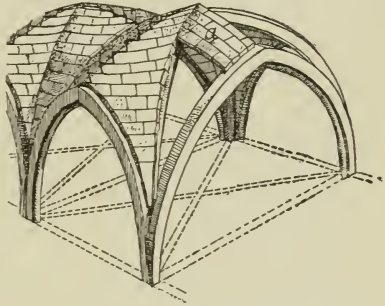
FIG. 119.—GROINED VAULT WITH ZIG-ZAG RIDGE-JOINTS.
