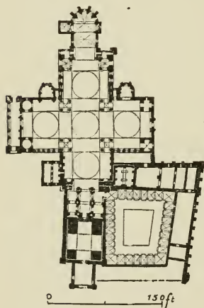
FIG. 94.—PLAN OF ST. FRONT.
