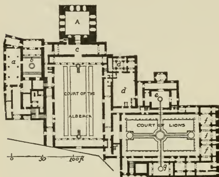
FIG. 84.—PLAN OF THE ALHAMBRA.
