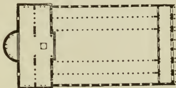
FIG. 67.—PLAN OF THE BASILICA OF ST. PAUL.
