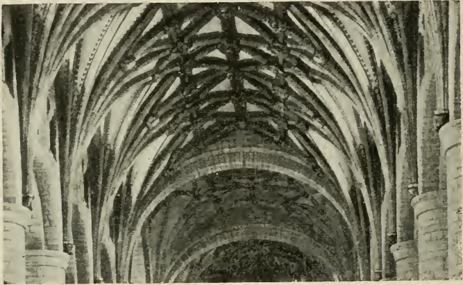
FIG. 130. —NET OR LIERNE VAULTING, TEWKESBURY ABBEY.
