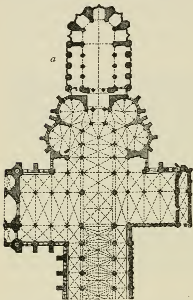
FIG. 137.—EASTERN HALF OF WESTMINSTER ABBEY.
