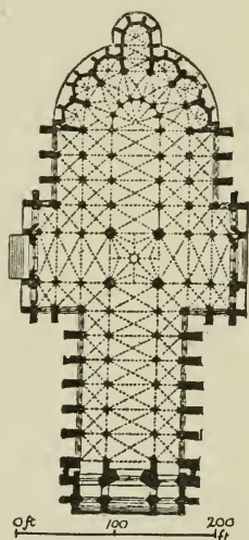
FIG. 122.—PLAN OF AMIENS CATHEDRAL.
