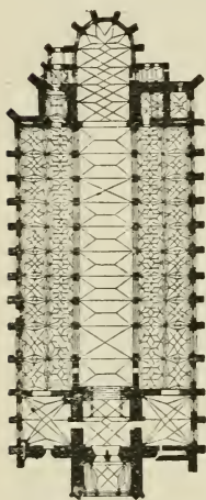
FIG. 143.—PLAN OF ULM CATHEDRAL.
