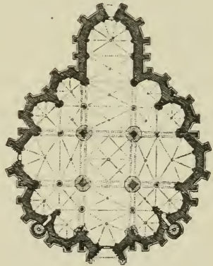
FIG. 142.—CHURCH OF OUR LADY, TREVES.
