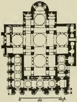
FIG. 78.—PLAN OF ST. MARK'S, VENICE.
