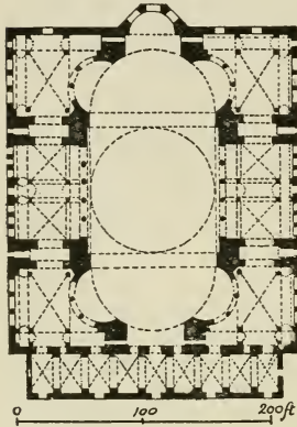
FIG. 75.—PLAN OF HAGIA SOPHIA.
