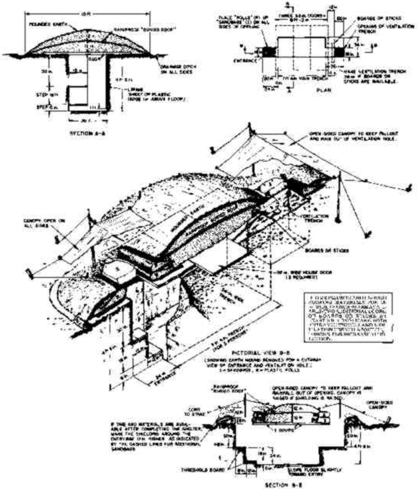
Fig. A.1. Door-Covered Trench Shelter.
