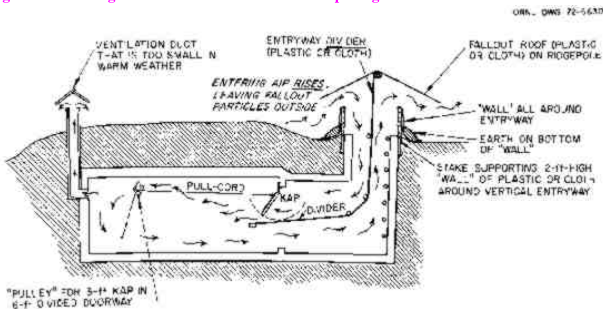
Fig. 15. Ventilating a shelter when the air-exhaust opening is too small. ORNL DWG 72-6630
