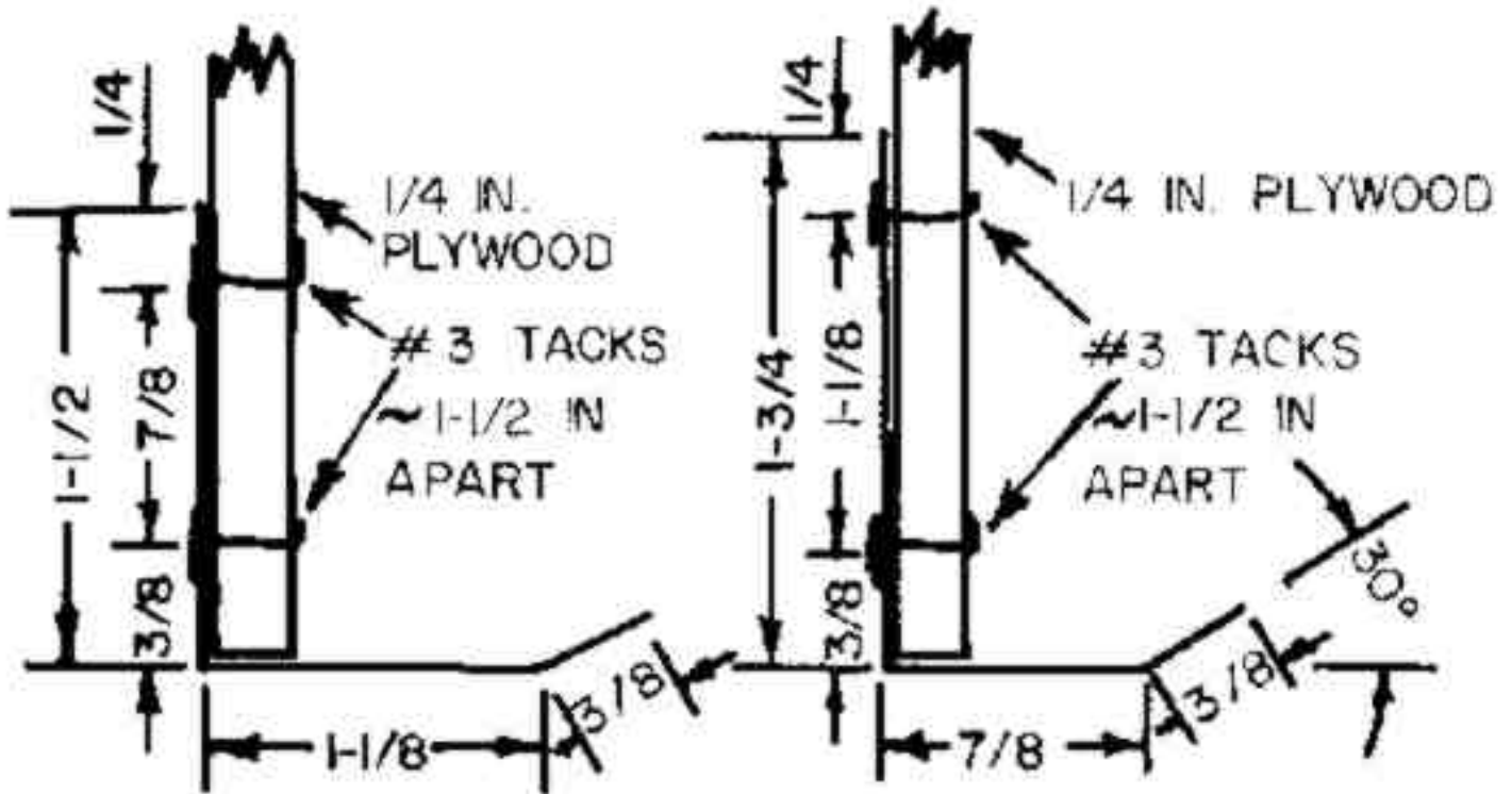
A TOP OR BOTTOM SHEETMETAL STRIP (11-13/16 IN. LONG)
