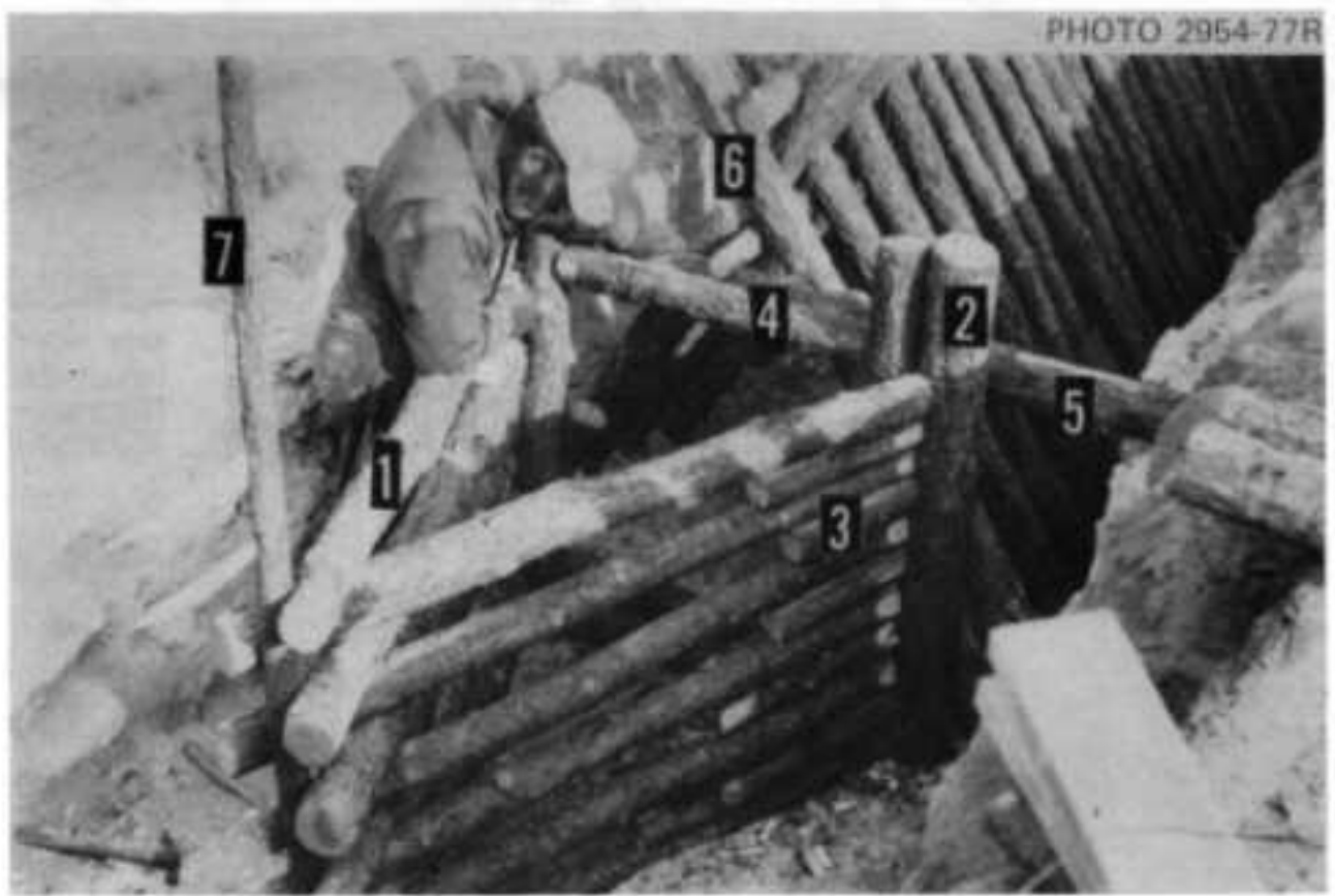
Fig. D. 10. Uncompleted lower section of a vertical triangular entry. (Photo 2954-77R)
