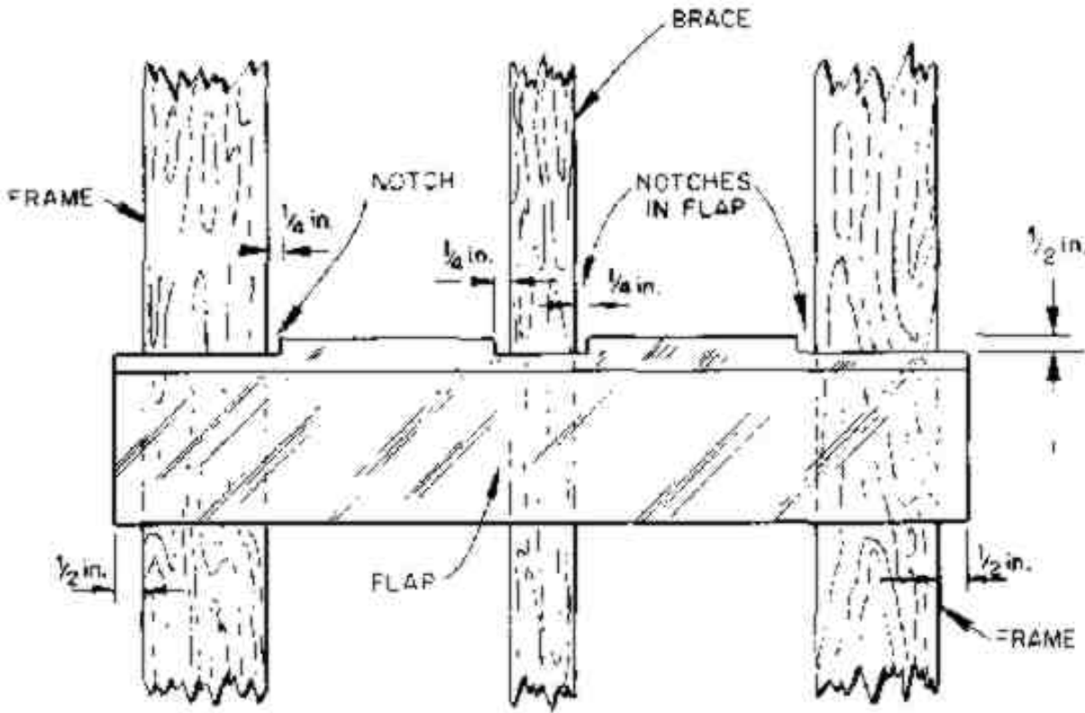
Fig. 6. Sizes of notches in flaps.
