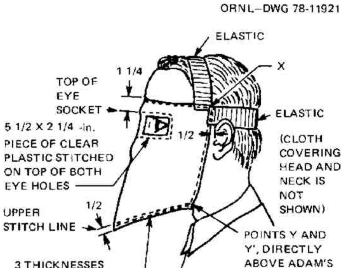
Fig. 15.9. A Russian-type homemade fallout mask. For most Americans this will continue to be a low-priority item as long as Russian warheads are large. ORNL-DWG 78-11921
