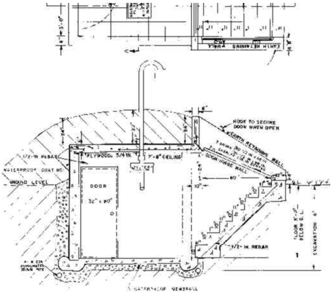
Fig. 17.1. Permanent Family Fallout Shelter for Dual Use.
