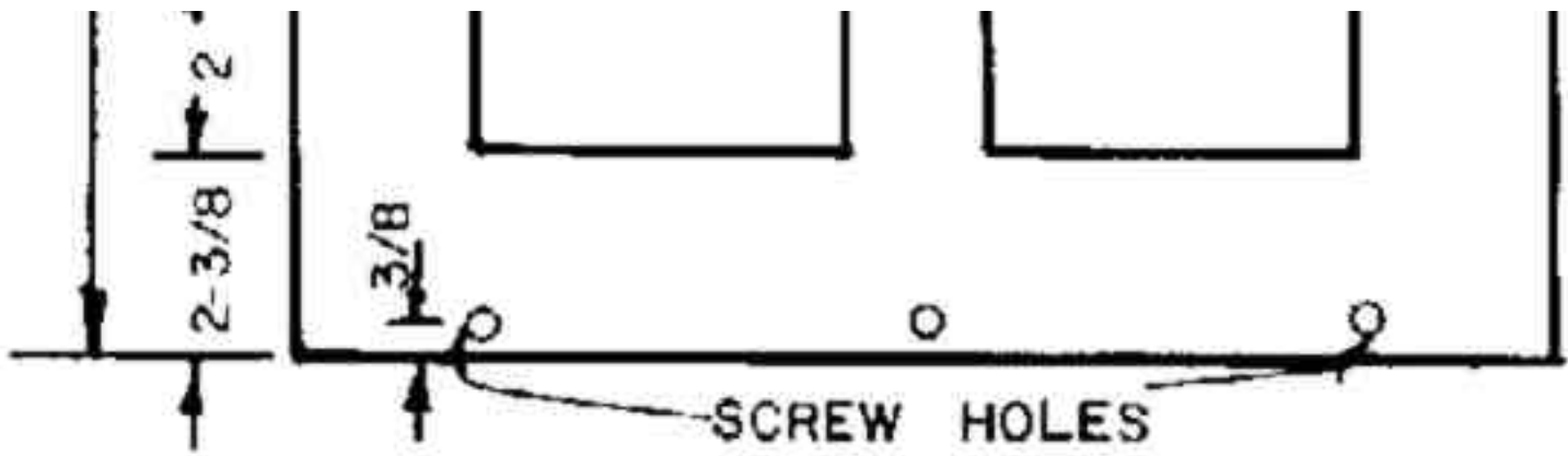
Fig. 8. Back End. Only the plywood is shown.
