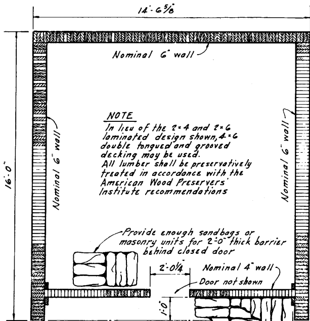
FLOOR PLAN
