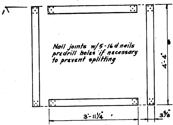
FRAME DETAIL
