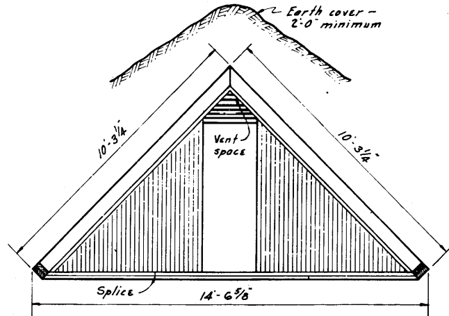
Sandbag or masonry barrier 2'-0" thick FRONT ELEVATION
