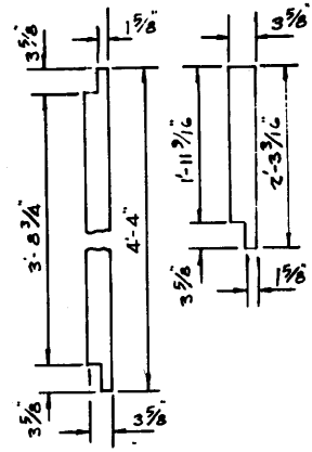
STIFFENER DETAILS
