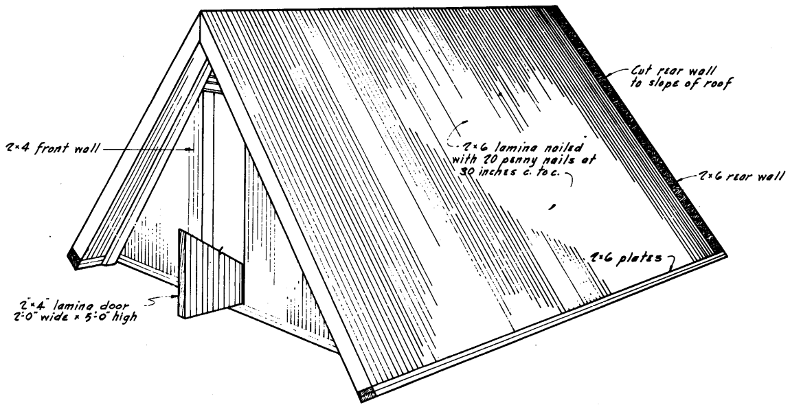
PERSPECTIVE VIEW
