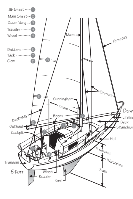
Figure A-1: The parts of a keelboat.
