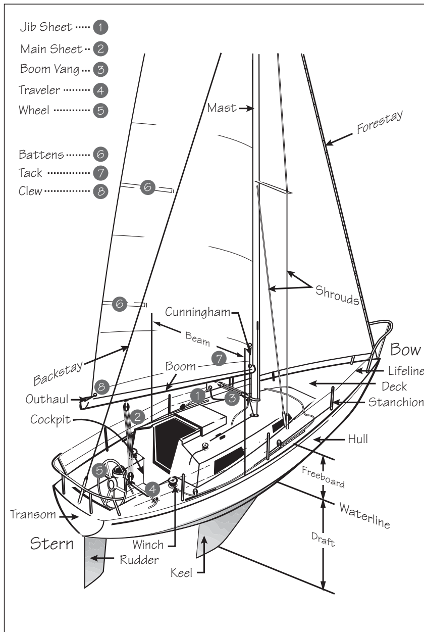
Figure 4-1: The parts of a keelboat.
