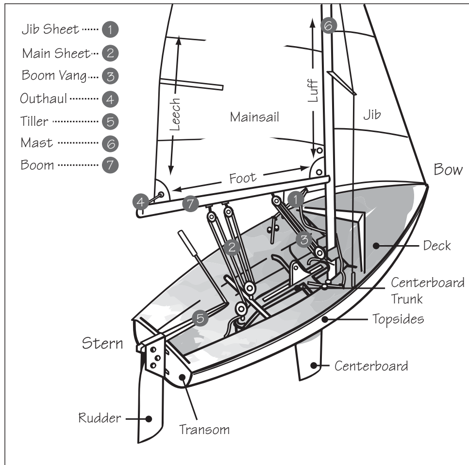
Figure 4-2: The parts of a dinghy.
