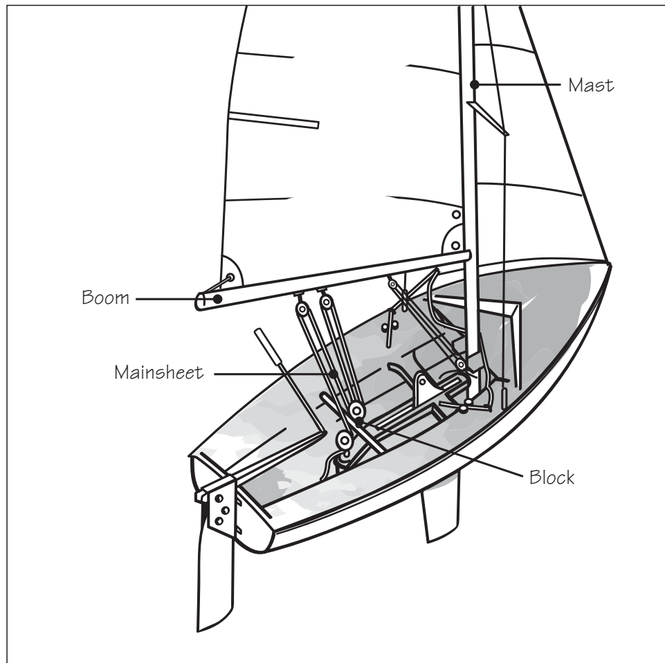
Figure 1-6: Mainsheet system on a dinghy.
