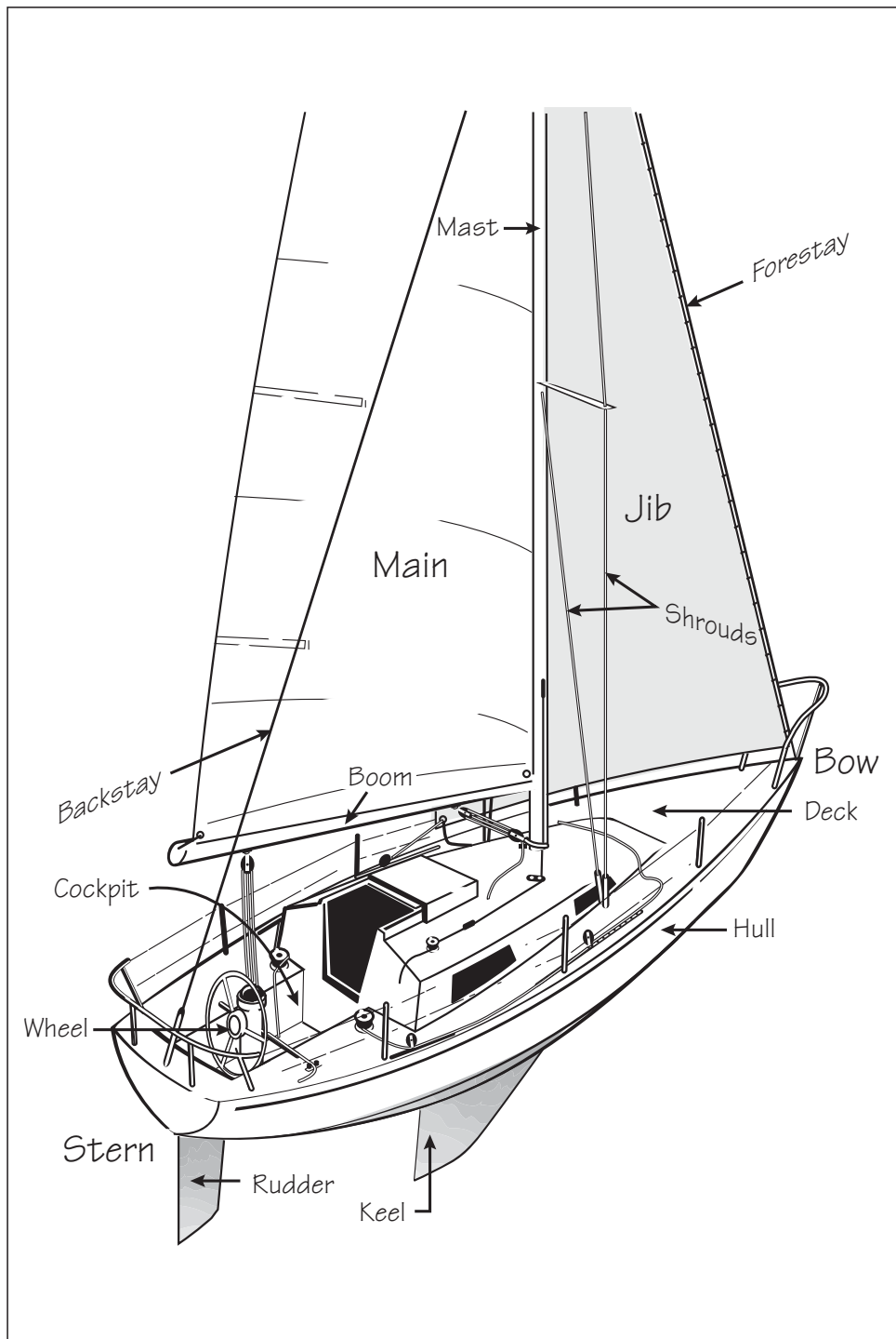
Figure 1-5: The basic parts of a keelboat.
