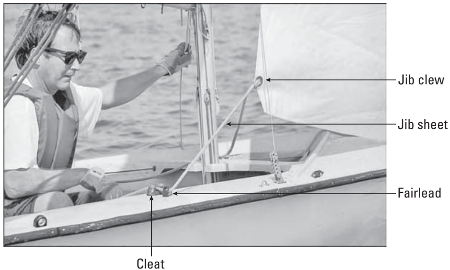
Figure 4-11: Jib sheet system on a 420-class dinghy.
