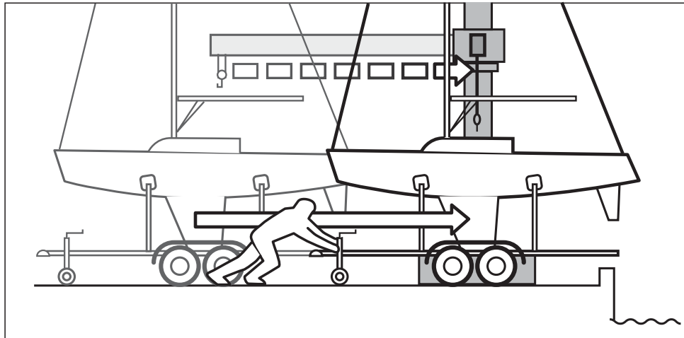
Figure 6-7: As the trailer is pushed under the crane, swing the crane's arm past the backstay.
