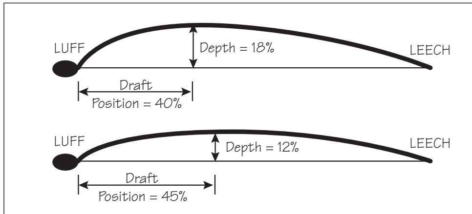
Figure 12-6: A fuller, draft-forward sail shape (top) gives you more power for lighter winds.
