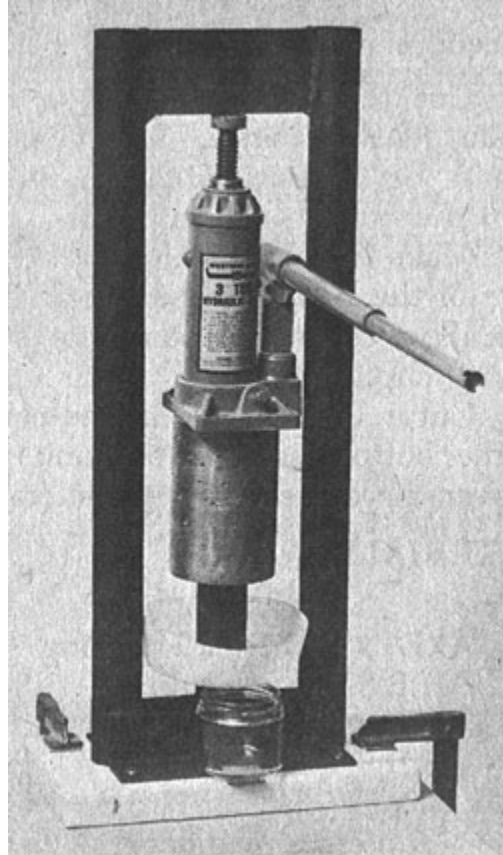
A welded frame offers the necessary support for pressing with a 3-ton hydraulic jack.
