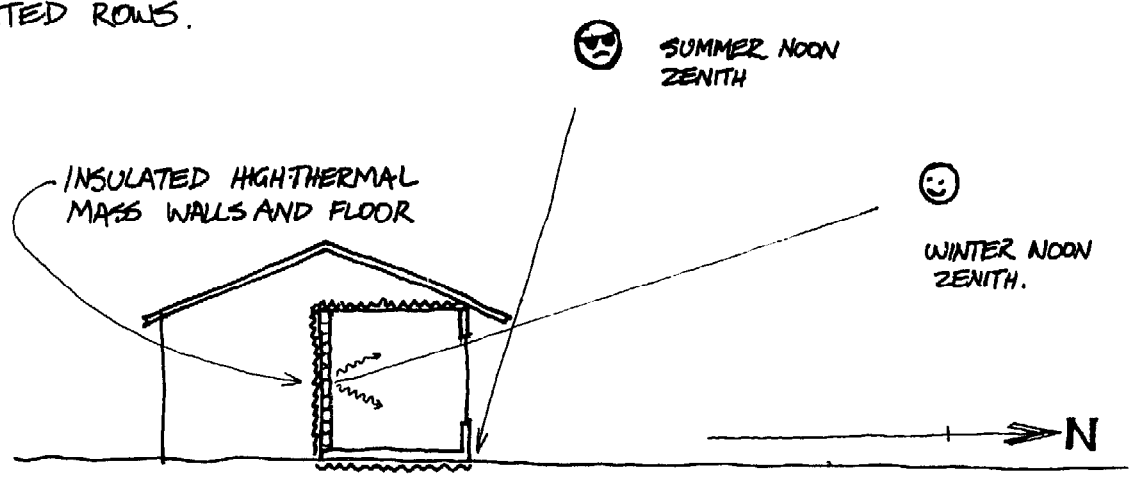
FIG 6:21: SUN/WINDOW/EAVE RELATIONSHIP.
