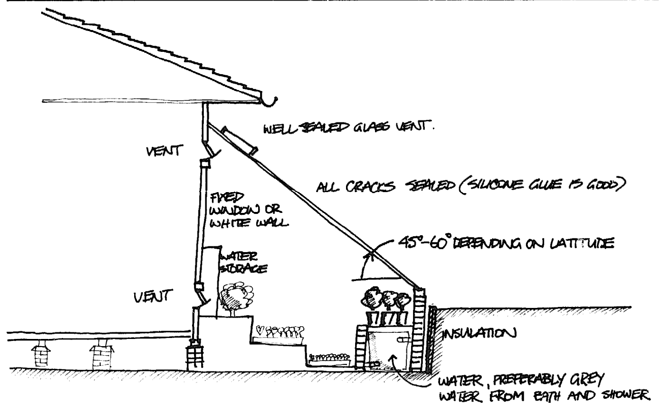
ESSENTIALS OF THE ATTACHED GLASSHOUSE. FIG. 6.3
