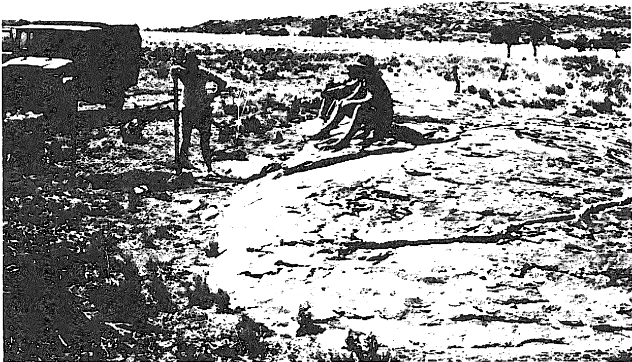
WEMIKUTTA. SMALL DOME FITTED WITH A CONCRETE GUTTER BY ANDREW AND KIM LEADS TO A NETTED TREE ENCLOSURE WITH PISTACHIO. (SEE FIG. 55). GUTTER IS SNAKE-LIKE LINE ON STONE. PLATE 5-7
