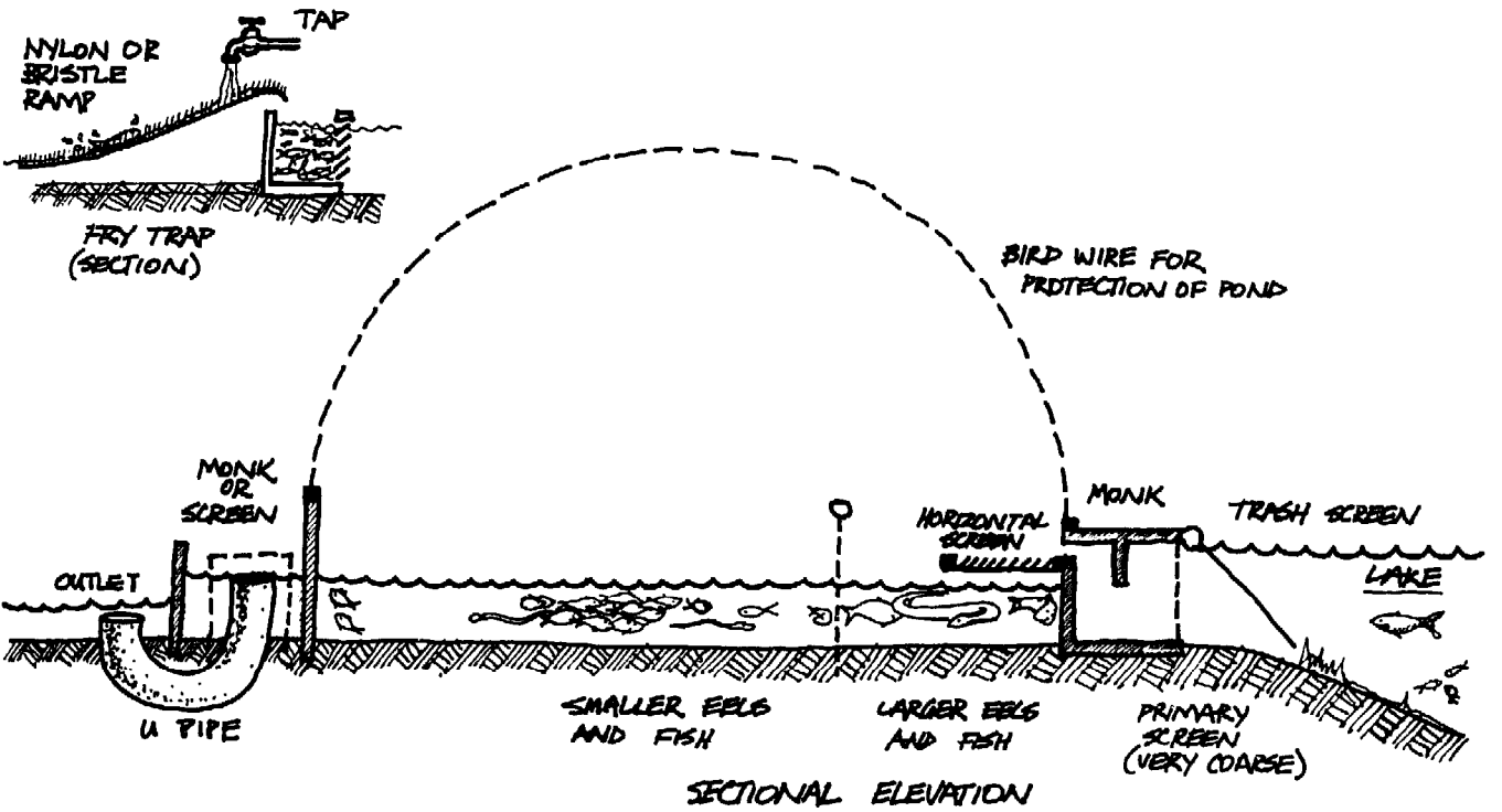
FIG. 7.23: COMPLEX OUTLET DEALING WITH CAPTURE OF UPSTREAM FRY, ELVERS, DOWNSTREAM ADULTS (EEL POND PLUS SOME FISH). POND HOLDS ADULTS MOVING TO SEA.
