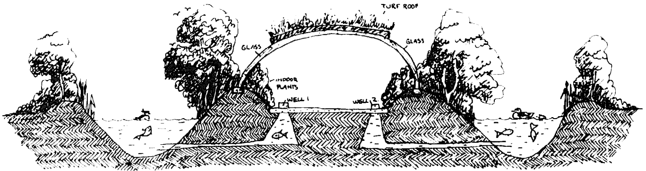
FIG. 6.6 SECTION OF EARTH HOUSE - LIGHT INDOOR DIVISIONS CAN BE MADE. END WALLS OF GLASS TO NORTH, SOLID TO SOUTH.
