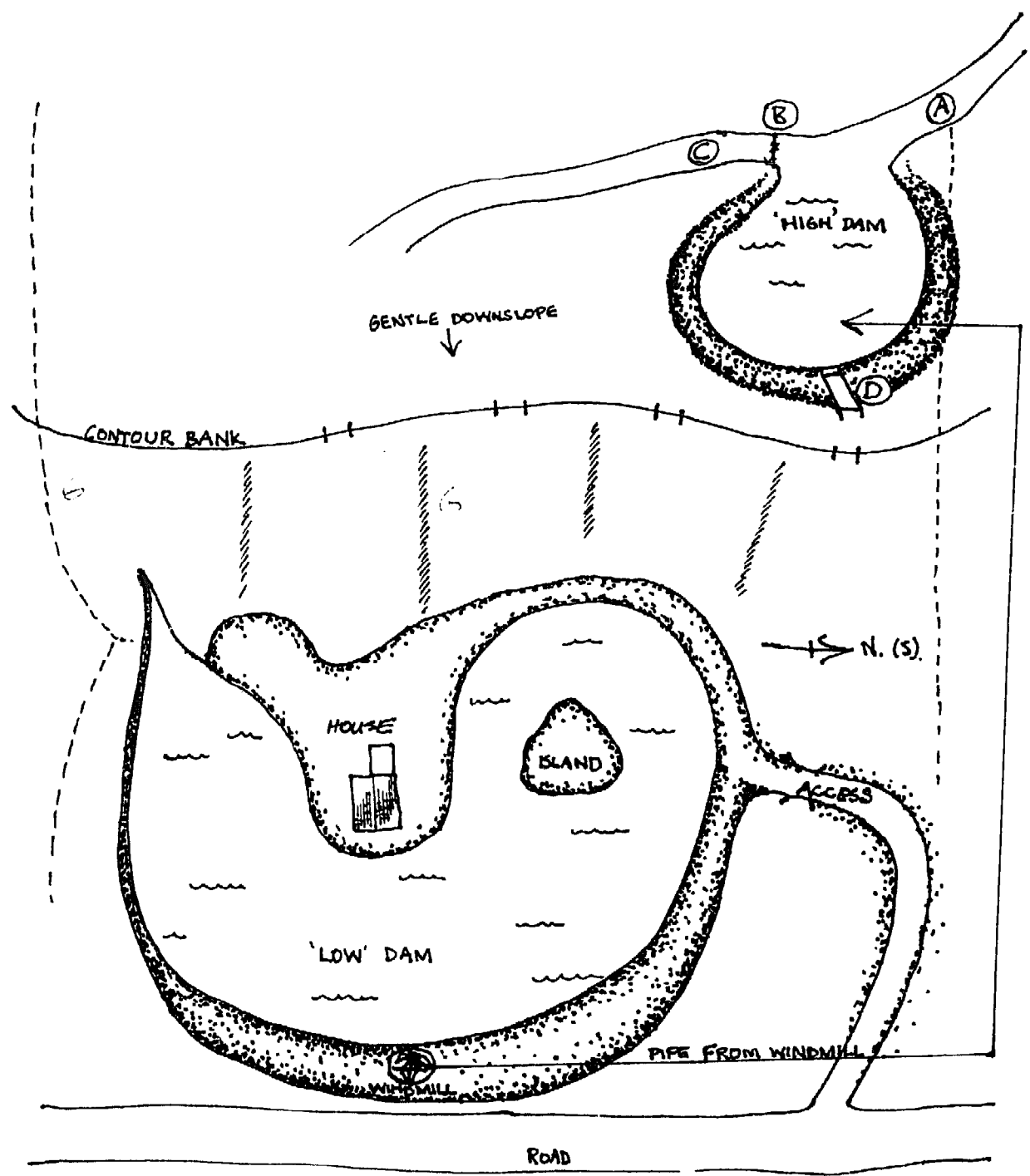
LAYOUT OF 5 ACRES AT DICGER'S REST, VICTORIA. HOUSE PROTECTED FROM FIRE, WHOLE AREA WATER CONTROLLED. DESIGNED BY YEOMANS, GALL AND MOLLISON. (SEE DETAIL FIG. 7.14.)
