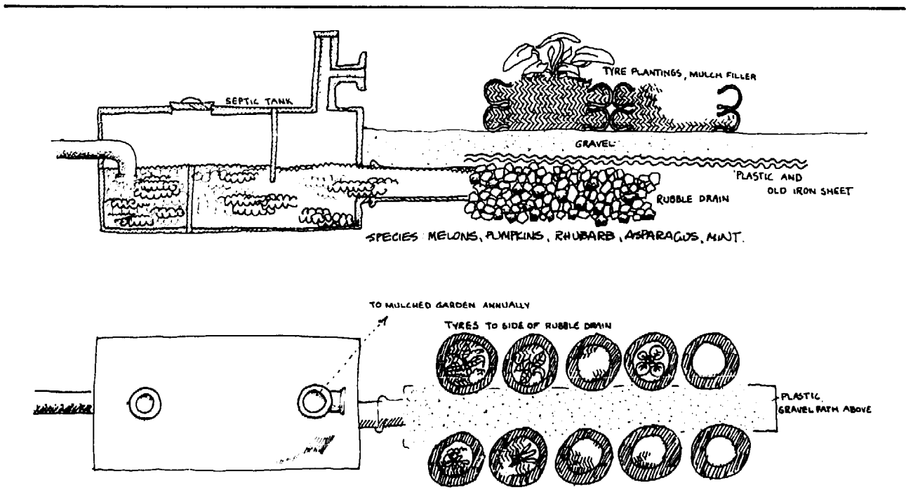
FIG. 6:20: DISPOSAL OF SEPTIC TANK EFFLUENT OR SULLAGE VIA TYRE-PLANTED ROWS.
