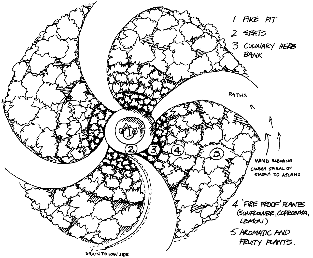
FIG. 6-17: FIRE MANDALA (PLAN).
