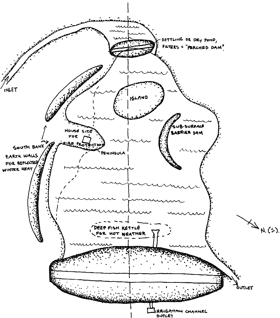
POSSIBLE "COMPLICATIONS" ON CLASSICAL DAM, FOR PERMACULTURE PURPOSES. FIG. 7.3:
