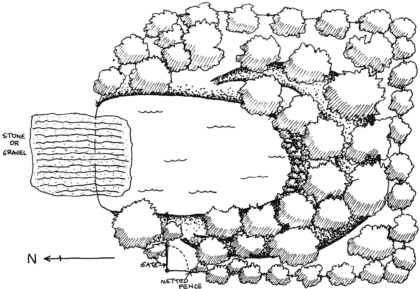
PLAN OF 'REFORMED' EARTH TANKS. IF ORIENTED TO NORTH POND BECOMES HEAT AND LIGHT REFLECTOR TO FORM A HOT MICROCLIMATE WHERE SPECIES, NOT NORMALLY GROWABLE IN THE AREA, WILL GROW. FOR EXAMPLE AVOCADO IN A COOL TEMPERATE ZONE. FIG. 7.6
