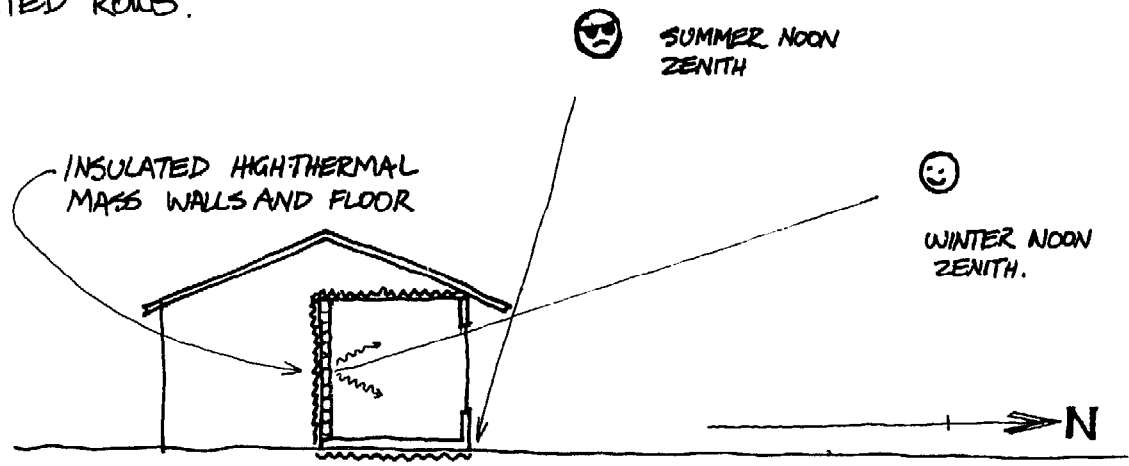
FIG 6:21: SUN/WINDOW/EAVE RELATIONSHIP.
