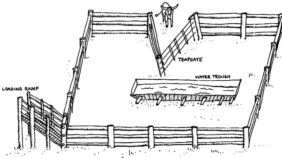
FIG. 5.22: TRAPYARD - WATER TROUGH ATTRACTS FERAL HERBIVORES IN DROUGHT.
