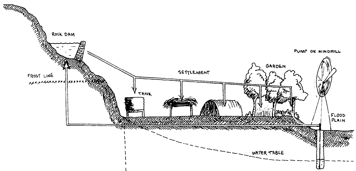
FIG. 5.2: IDEAL RELATIONSHIPS — WATER, SETTLEMENT, GARDENS FOR ARID LANDS
