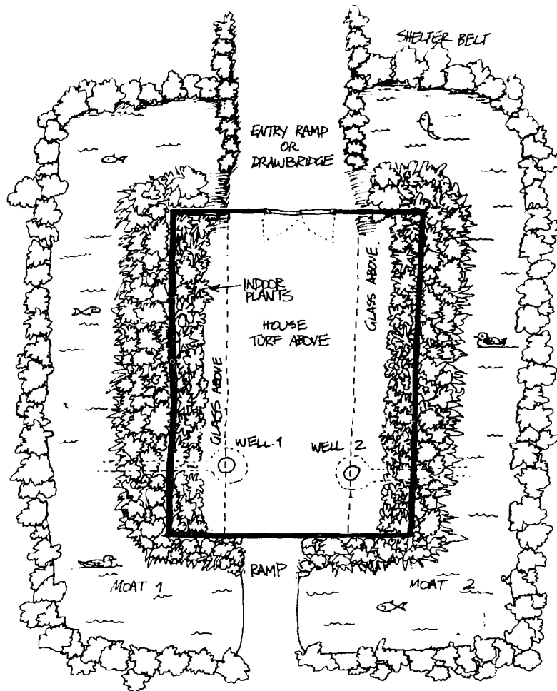
FIG. 6.7: PLAN OF EARTH HOUSE DESIGNED FOR TUNDRA OR WINDY FLAT PLAINS.
