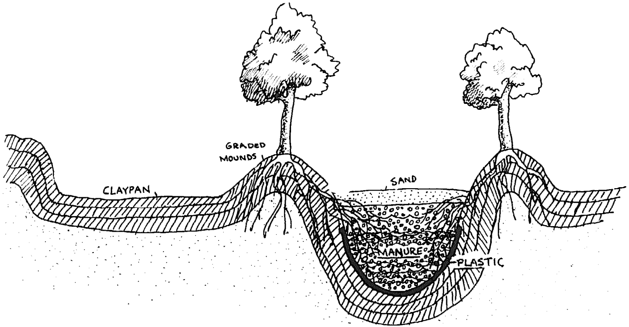
FIG. 5.16: CLAYPANS - MANURE 'WELLS' IN CLAY PANS STORE FLOOD WATER FOR MOUNDED PLANTS.
