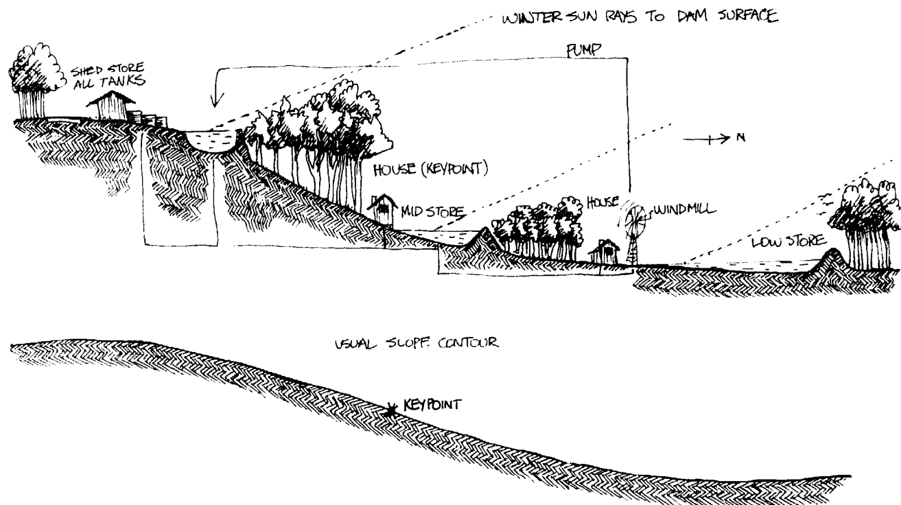
IDEAL PLACEMENT OF ELEMENTS IN RELATION TO SLOPE: FIG.27
