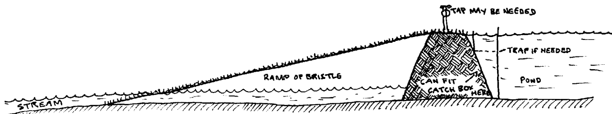
A SLOPE OF NYLON BRUSH BRISTLE, OR TURF, OR ROUGH STONE FOR WRIGGLING AND CREEPING SPECIES SUCH AS ELMERS, YABBIES, SHRIMPS, ETC (AFTER MODEL AT LIMERICK, IRELAND).
