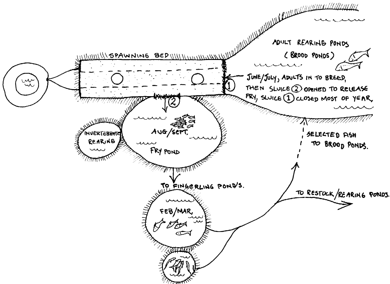
SCHEMATIC POND SYSTEM (TROUT)
