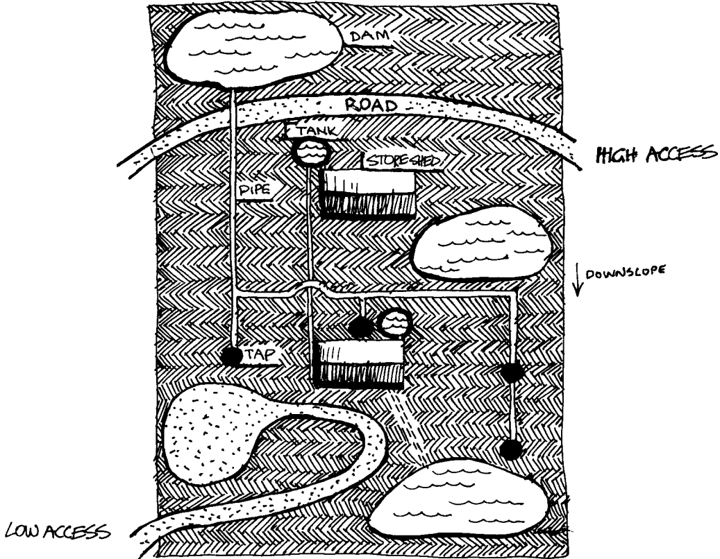
IDEALIZED. DOWNSLOPE LAYOUT OF WATER, BUILDINGS, ACCESS. FIG. 2:10:
