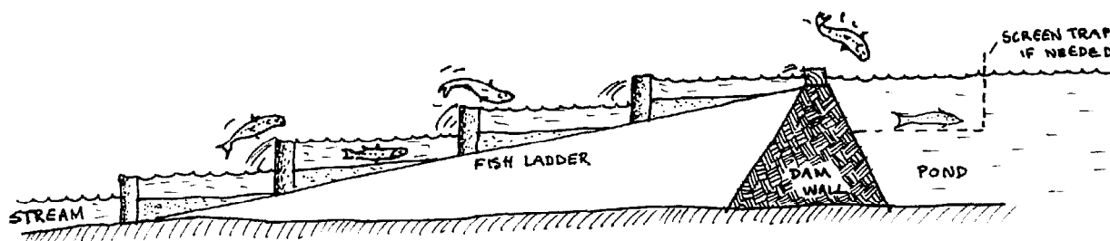
A FISH LADDER FOR LEAPING FISH SPECIES SUCH AS TROUT.
