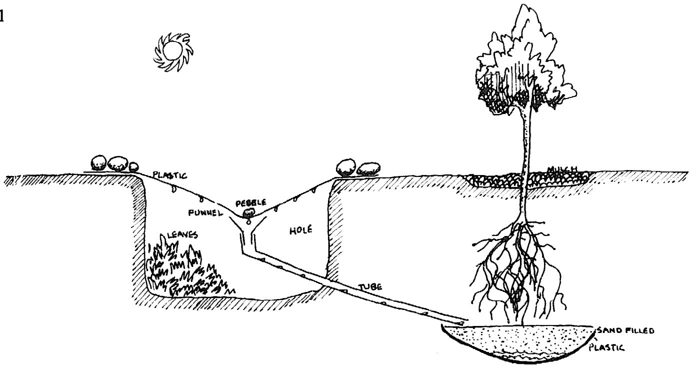
FIG.5:20: PLASTIC STILL USES LEAVES OR SOIL TO DISTILL WATER FOR PLANT RESEVOIR.
