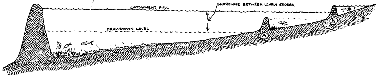
FIG. 7.8: MAJOR CATCHMENT MODIFICATIONS (SECTION). MODIFIERS ARE A SUBSURFACE DAM TO PRESERVE AND PROTECT SHORELINE; AND B PERCHED DAM TO BREED SMALL FORAGE FISH SPECIES.
