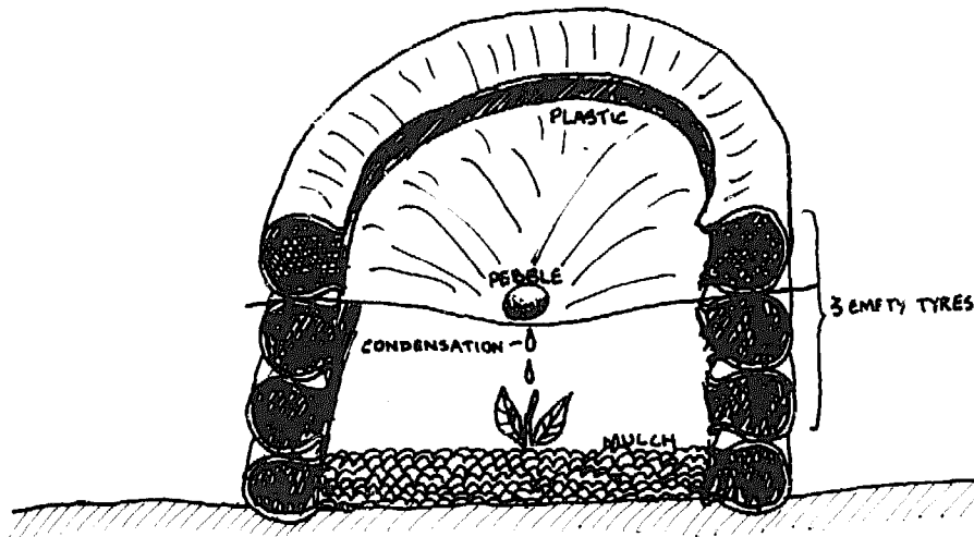
FIG.5:21: TYRE GLASSHOUSE - PLASTIC CONDENSES NIGHT MOISTURE. PLASTIC COVER REMOVED LATE SPRING. SELF WATERING AND FROST FREE.
