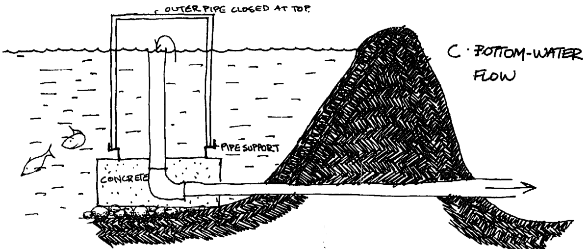
POND OUTLET STRUCTURES (AFTER CHAKROFF 16 ). FIG. 7:18
