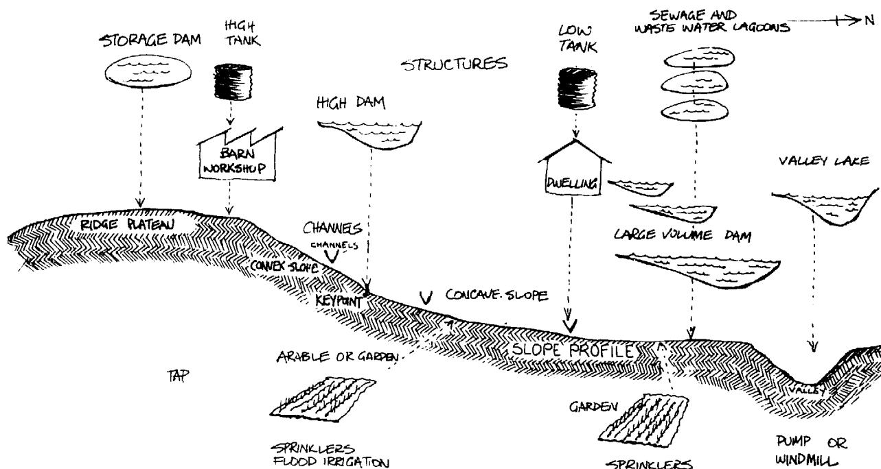
FIG. 2.8: IDEAL RELATIONSHIPS OF STRUCTURES AND WATER STORAGES ON SLOPES (FUNCTIONS AND USES).
