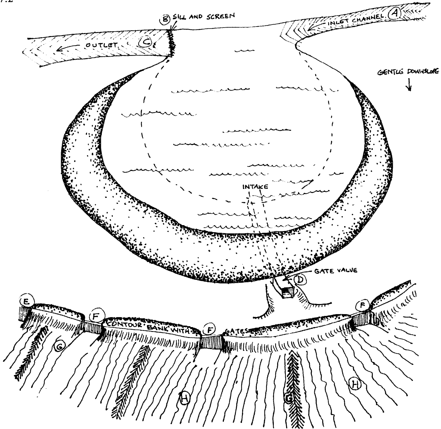
FIG. 7.14: HIGH HOLDING DAM GATHERS WATER AT (A) FROM A 1:150 LEAD IN (DIVERSION) DRAIN ACROSS SLOPE. IN FLOOD, THIS LEAD IN WATER SPILLS ACROSS SILL (B) TO OUTLET CHANNEL (C) OR CAN BE RELEASED THROUGH GATE VALVE (D) AT ANY TIME. CONTOUR BANK (E) HOLDS RELEASED WATER FOR CONTROLLED LIBERATION INTO FIELDS (H) VIA GATES (F). WATER IS THEN CONTROLLED BY VERY LOW STEERING BANKS (G), AND SOAKS INTO CHISEL PLOUGHED FIELDS. DIRECTION OF CHISELING INDICATED BY WIDE-SPACED LINES. (AFTER DAM AT DIGGER'S REST DESIGNED BY KEN YEOMANS).
