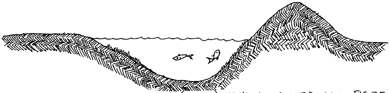
TYPICAL EARBANKS OF FLATLANDS (SECTION). USUALLY UNPLANTED, OPEN TO WIND AND EVAPORATION. OFTEN WASTE SUBSOIL IS HEAPED ON THE SUN SIDE AND STOCK CAN APPROACH FROM ANY QUARTER MUDDING WATER. FIG. 7.5
