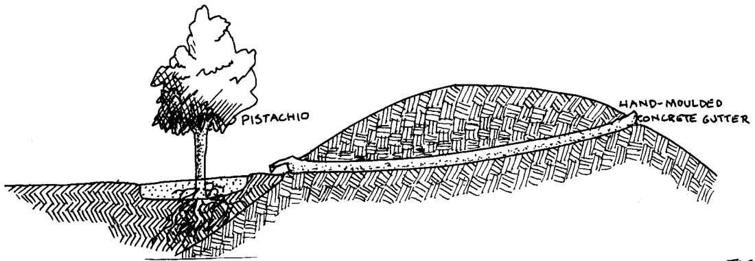
AT WOMIKUTTA : SMALLER ROCK DOME SUFFICES FOR A TREE OR TWO. FIG. 5.5
