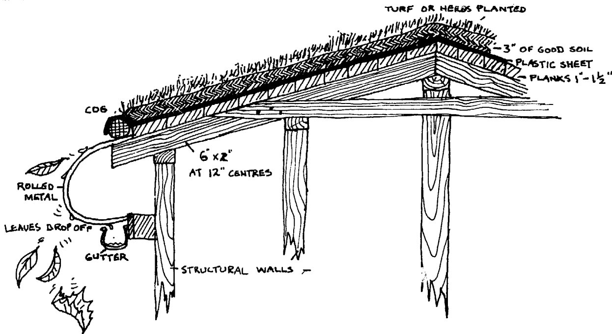
TURF ROOF CONSTRUCTION. FIG 6-16
