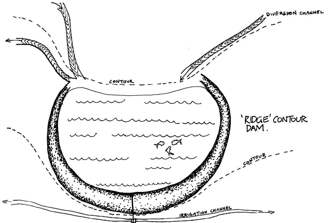
FIG. 7-4: CONTOUR DAMS .
