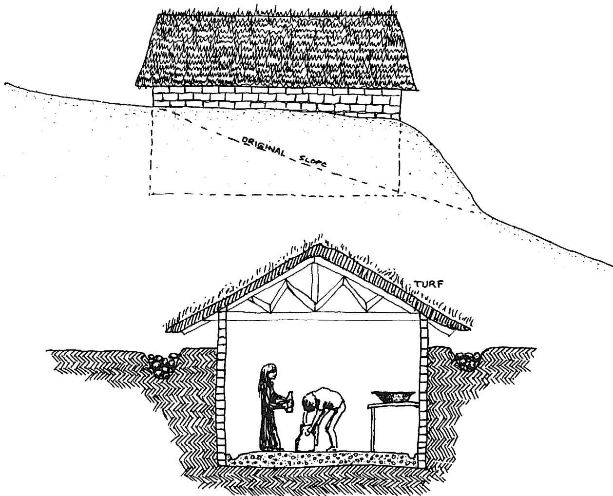
EARTH HOUSE TRADITIONAL BUSH DAIRY CUT INTO BANK, WALLS OF MASONRY, TURF ROOF, TAMPED EARTH OR CONCRETE FLOOR. EAVES PROJECT TO RUBBLE DRAIN. COOL IN ANY WEATHER. FIG. 6.8
