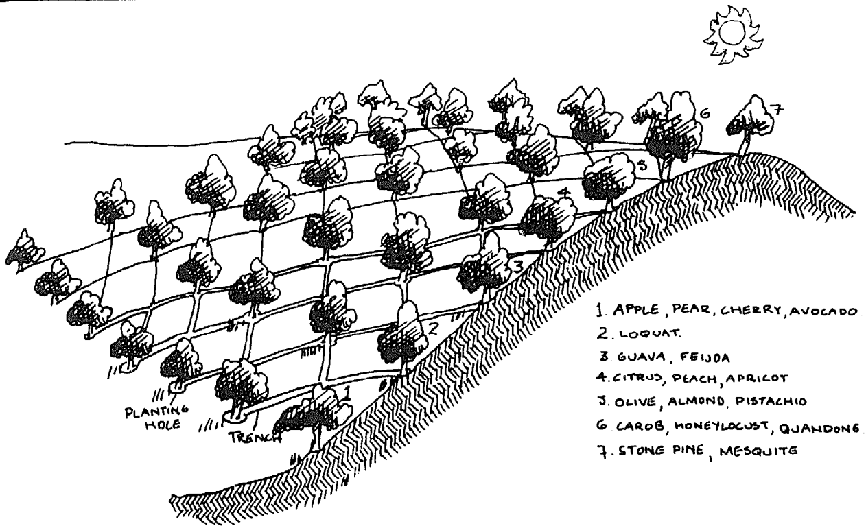
FIG. 5.3: NET AND PAN FOR DRY, STONY HILLSIDE.
