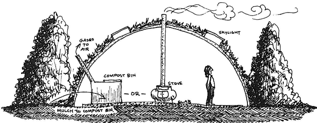
PLANT HOUSE 3 (SECTION). METAL, CONCRETE, PLASTIC OR WOODEN DOME WITH IVY OR TURF COVER, PLANT WALL SHELTERS.
