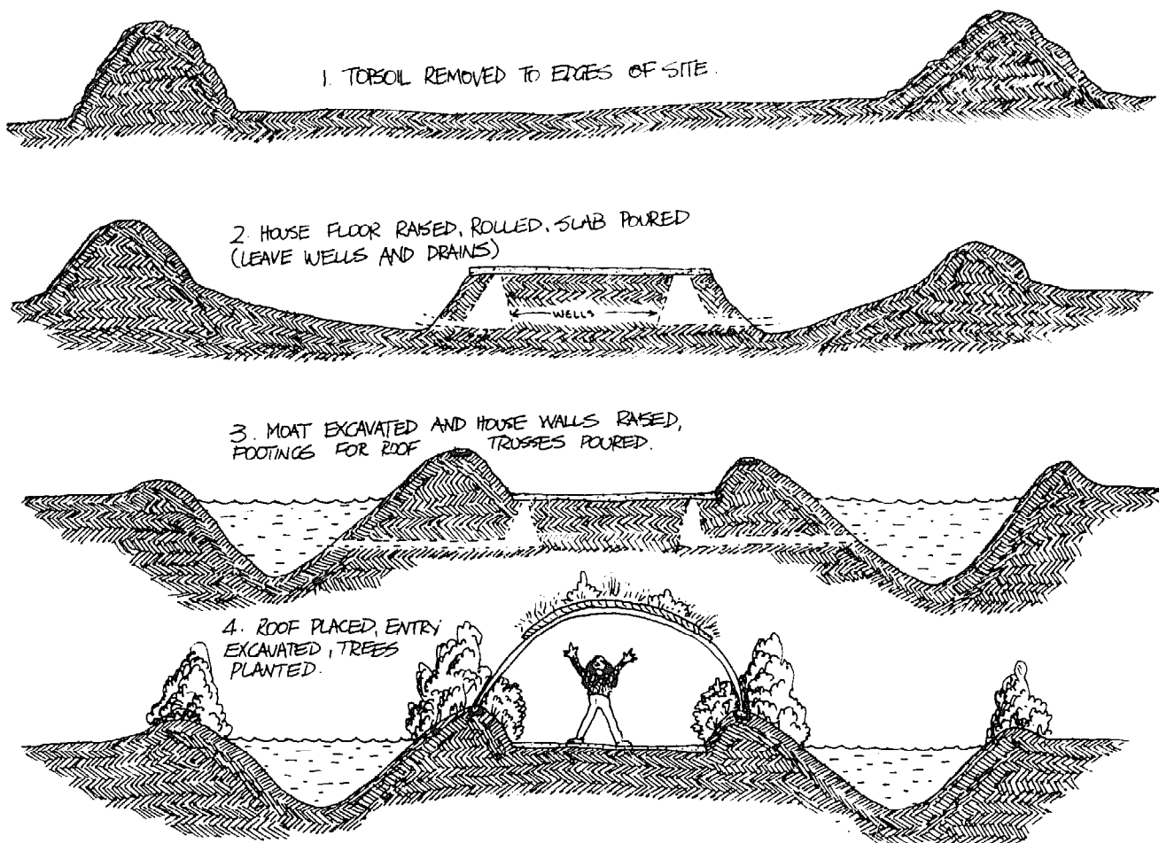
CONSTRUCTION STAGES OF EARTH HOUSE. FIG. 6.5
