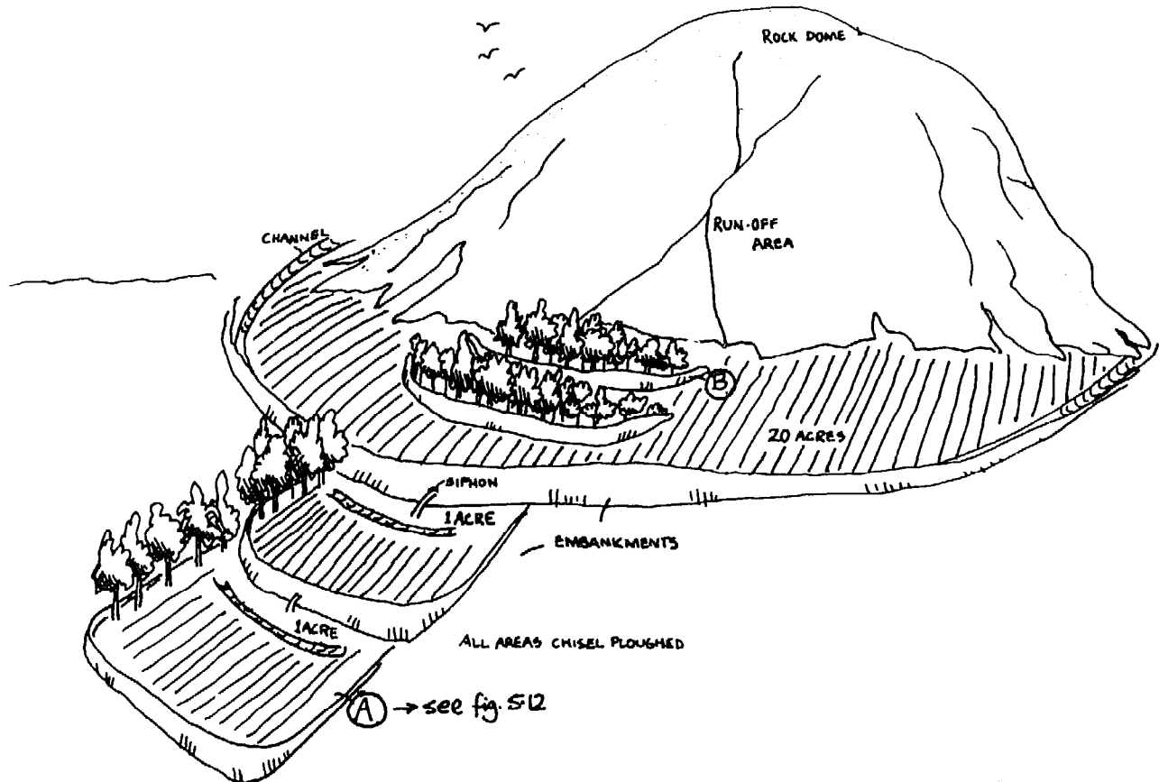
FIG. 5.13: RUN-OFF LED BY SIPHON TO SMALL CHISEL PLOUGHED FIELDS
