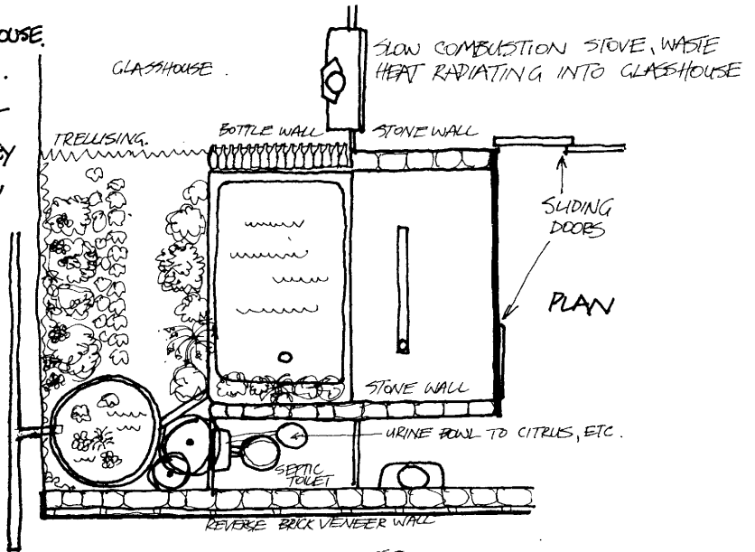
FIG. 6-13: BATHROOM GLASSHOUSE. SHOWER OVER PEBBLE BED KEEPS PLANTS MOIST. CAN BE ATTACHED TO EXISTING BATHROOM AS 'HOT' OR 'COLD' GLASSHOUSE.
