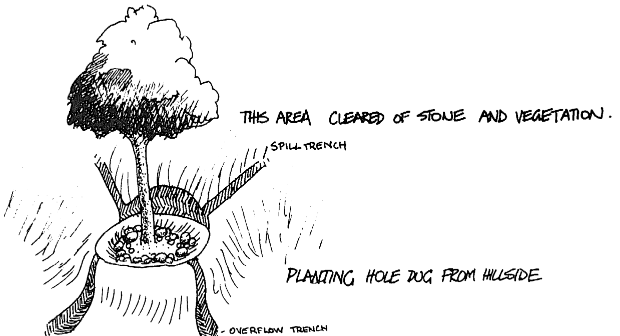
FIG. 5.4: DETAIL OF PAN.
