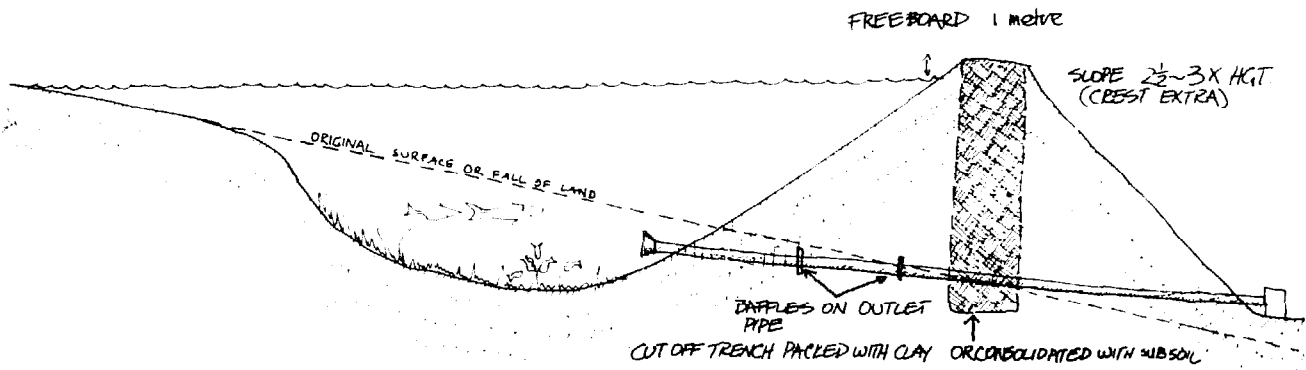
A CLASSICAL BARRAGE DAM (AFTER YEOMANS 2 ). SECTION. FIG. 7.2:
