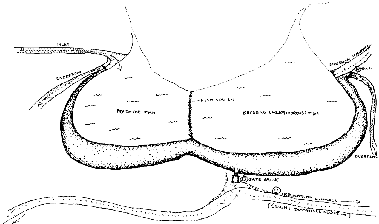
FIG. 7.12: "DOUBLE" DAM IN DEPRESSION CONNECTED VIA FISH SCREEN. PREDATORS (TROUT) KEEP HERBIVORES (PERCH) CULLED VIA FISH SCREEN (YANDOIT, VICTORIA)
