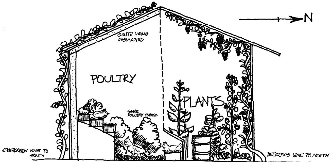
CHICKEN HEATED GLASSHOUSE. FIG. 8.3.
