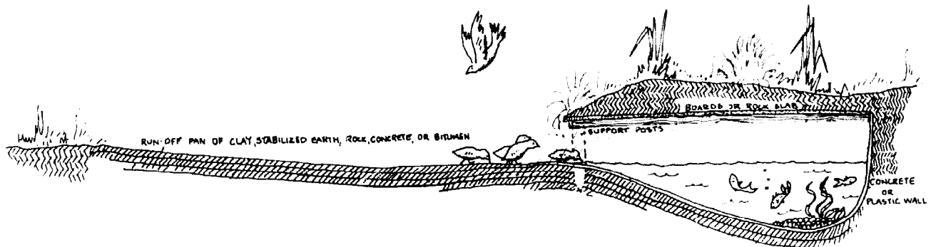
FIG. 5.14: SMALL WELL IN CLAYPAN OR ON ROCK BASE HOLDS WATER FOR QUAIL, PIGEON, LIZARD SPECIES, BEES. FISH AND MUSSELS KEEP WATER CLEAR. CATTLE CANNOT FOUL SUCH WELLS.
