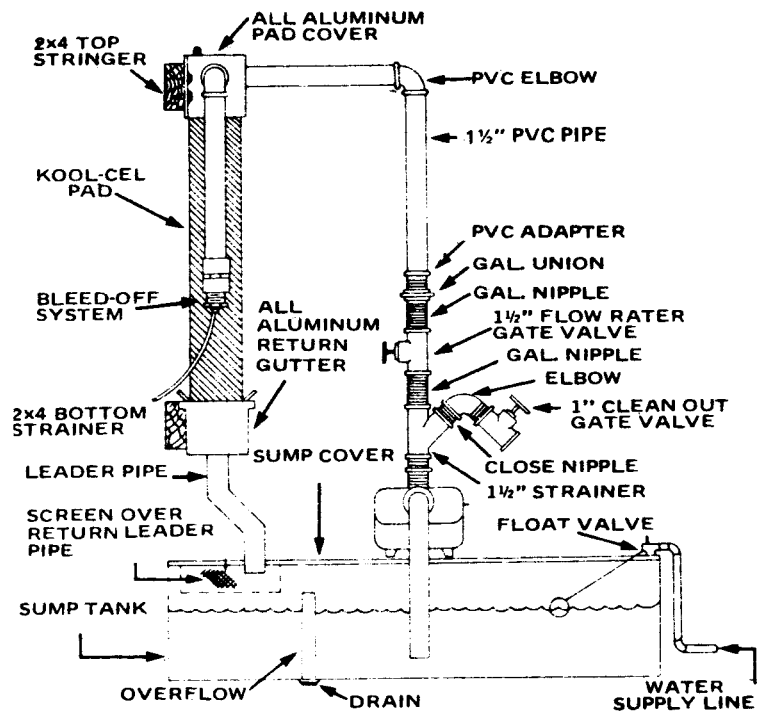
Figure 25. Evaporative cooling pad installation diagram.
