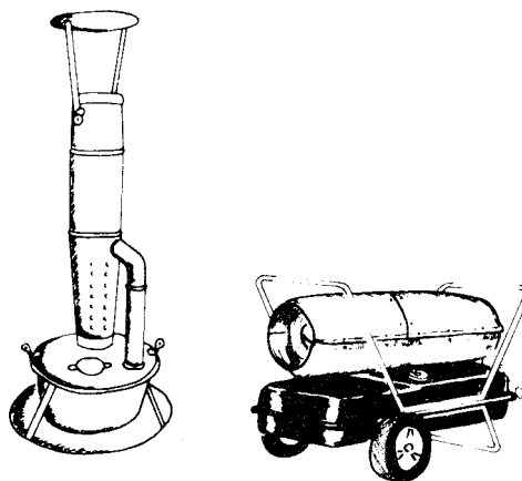
Figure 22. (a) Radiant heater, (b) hot-air heater.
