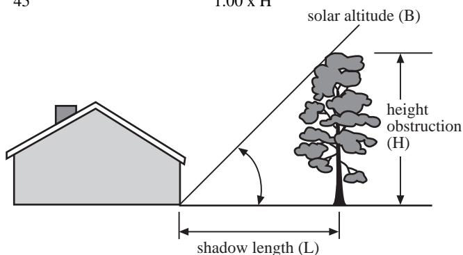
Figure 14. Ratio of shadow length and obstruction height for selected solar altitudes.
