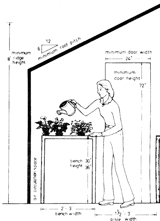
Figure 1. Lean-to greenhouse. A greenhouse may be from 6 to 12 feet wide and suggested minimum area of 100 square feet.
