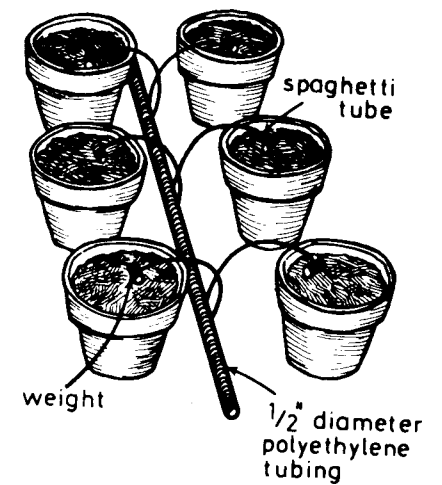
Figure 28c. Spaghetti Tube watering system.
