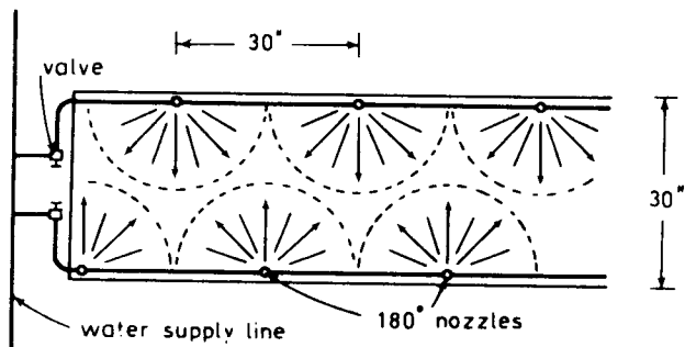
Figure 28a. 180° spray watering system.
