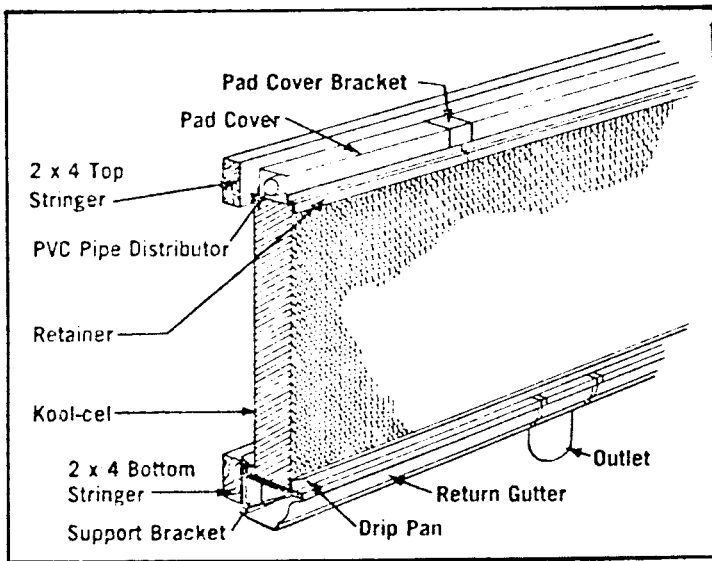
Figure 25. Evaporative cooling pad installation diagram.
