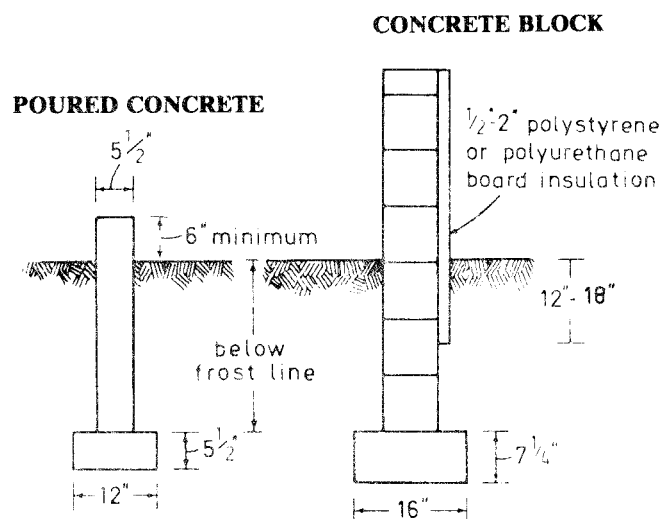
Figure 13. Typical masonry foundations
