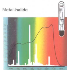
Above: High-pressure metal-halide lamps produce very bright light for their size and power input. Ideal for plants needing high light intensity.
