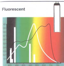
Above: Fluorescent tubes are ideal for plant growth. This output shows mercury discharge as bars, light from the fluorescent layer as a curve.
