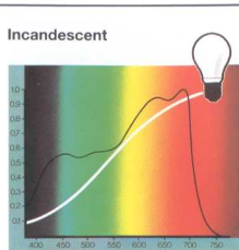
Above: Although inexpensive and easy to install, incandescent lamps produce a spectral output weighted towards the red part of the spectrum.
