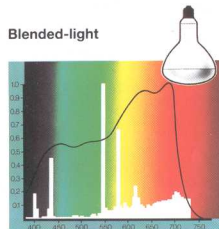
Above: The combination of tungsten and mercury elements in these lamps ensures a balanced light output for plant growth. Easy to use.
