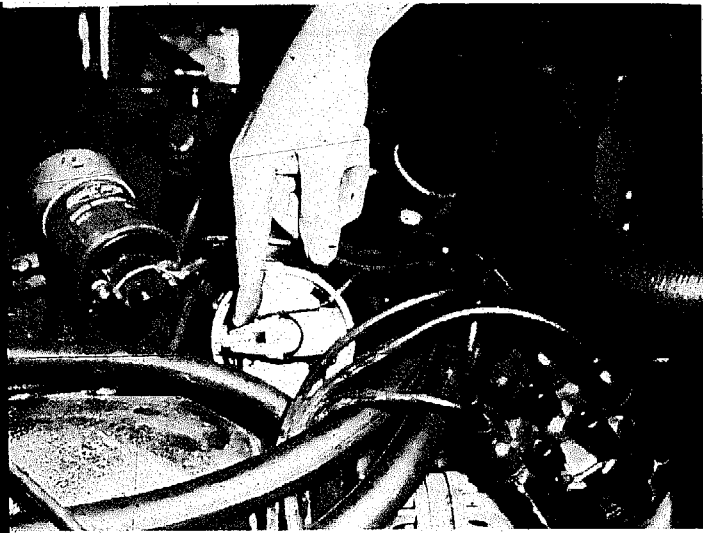
left: With distributor cap removed, the first thing you see is the rotor. Rotor contact end can become pitted with extended use, and contact spring piece on top may lose tension. Rotor is a slip fit on distributor shaft and will have an internal projection to match a slot on distributor drive shaft to insure correct orientation. right: Distributor cap should be checked occasionally for cracks and contact wear. A bad distributor drive shaft can wobble and allow the rotor to impact the metal contact points imbedded in the cap. The center graphite contact button may lose its spring-loading and not make sufficient contact with the rotor to insure complete ignition.
