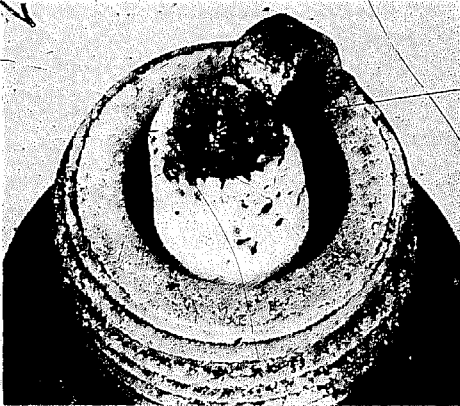
Preignition is a no-no. It's caused by combustion chamber deposits which become incandescent and ignite fuel before the plug does. Other causes include piston scuffing, detonation, cross firing, or plug heat range too high.
