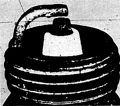
Overheated plugs have a blistered, white insulator and very few deposits. Check for correct plug heat range, overadvanced ignition timing, cooling system malfunction, leaking intake manifold, or sticking valves.
