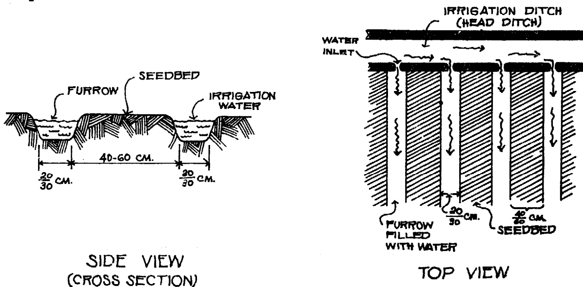
Fig. 7: Furrow irrigation
