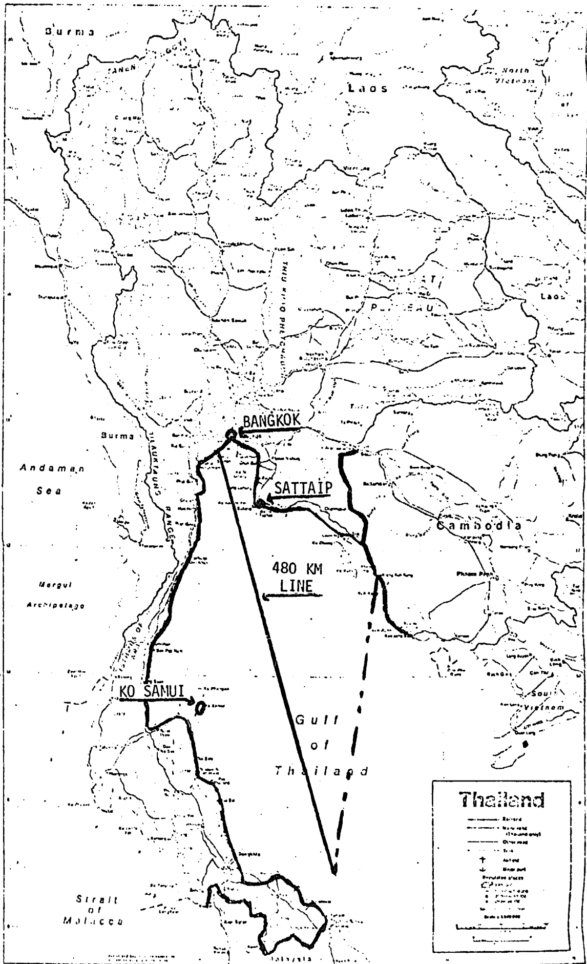
A PROPOSED OFFSHORE WINDPOWER SYSTEM FOR THE GULF OF THAILAND. FIG. (11)
