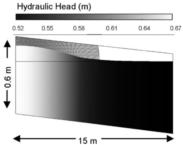
Fig. 8.5 The flow field which corresponds to the modelling parameters specified in Table 8.2 and the hydraulic conductivity profile illustrated in Fig. 8.4. The vertical contours in the upper sub-domain represent vertical infiltration through the surface layer and the shaded profile represents the variation of hydraulic head in the horizontal water table
