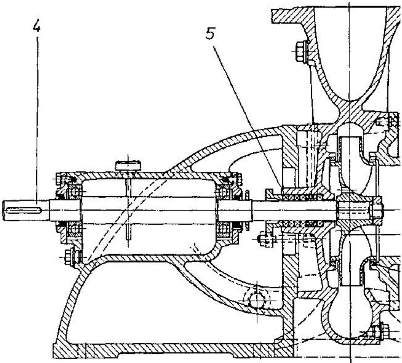
Fig. 7.11: Cross-sectional view of single-stage centrifugal pump (KSB).
