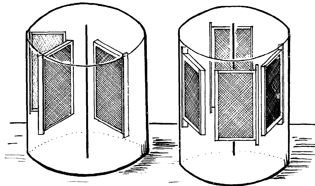
Basket-type extractor
