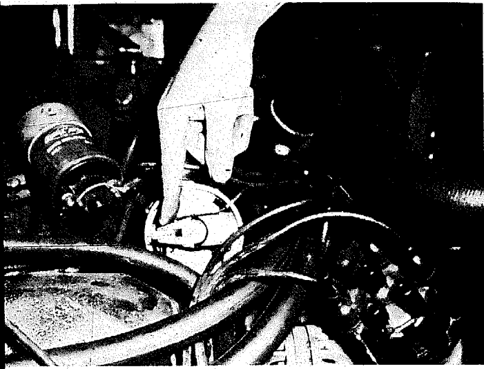
left: With distributor cap removed, the first thing you see is the rotor. Rotor contact end can become pitted with extended use, and contact spring piece on top may lose tension. Rotor is a slip fit on distributor shaft and will have an internal projection to match a slot on distributor drive shaft to insure correct orientation. right: Distributor cap should be checked occasionally for cracks and contact wear. A bad distributor drive shaft can wobble and allow the rotor to impact the metal contact points imbedded in the cap. The center graphite contact button may lose its spring-loading and not make sufficient contact with the rotor to insure complete ignition.
