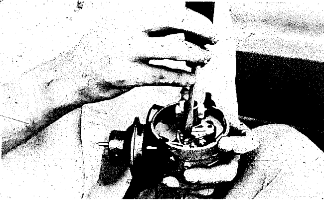
left: This is the easy way to change points! While we don't advise removing the distributor to change points, we do want to use this picture to point out that the screws that secure the points can be easily lost into one of the holes in the breaker plate and you will have to remove the distributor! right: All ignition coil connections should be tight and free of corrosion. Any dirt on terminals can cause some of the high voltage to "run off" and may result in insufficient voltage to the spark plugs.
