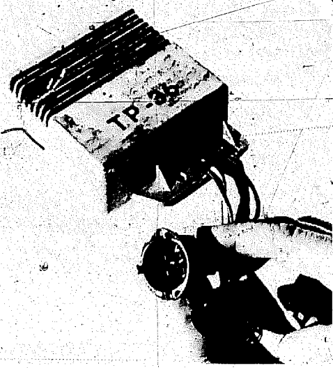
left: One nice thing about the new ignition systems is that it's pretty difficult to hook them up incorrectly after a component change. Ford Dura-Spark control module shows how spade-type male connectors and keyed connector housings are constructed to minimize assembly errors. right: GM HEI distributor cap is much changed from conventional cap. Large well in cap is where ignition coil goes, and projection on left is electrical connector. Pen points to new design of spark plug wire connectors.
