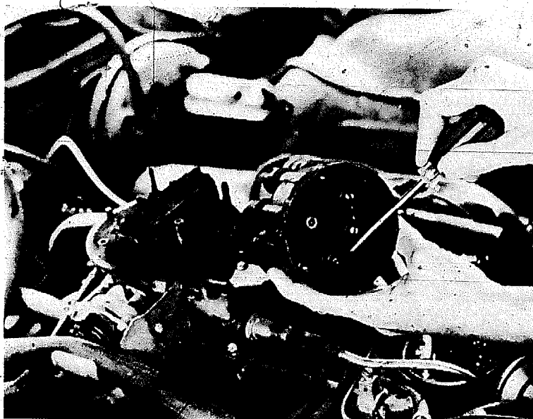
Light carbon deposits should be scraped off the distributor cap contacts. Heavy carbon build-up or cracks in the cap call for a new cap.
