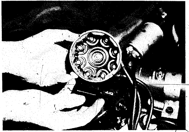
left: With distributor cap removed, the first thing you see is the rotor. Rotor contact end can become pitted with extended use, and contact spring piece on top may lose tension. Rotor is a slip fit on distributor shaft and will have an internal projection to match a slot on distributor drive shaft to insure correct orientation. right: Distributor cap should be checked occasionally for cracks and contact wear. A bad distributor drive shaft can wobble and allow the rotor to impact the metal contact points imbedded in the cap. The center graphite contact button may lose its spring-loading and not make sufficient contact with the rotor to insure complete ignition.
