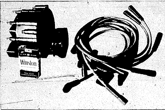
Left: Large size of GM HEI distributor cap is emphasized by cigarette pack. Plug wire size has been increased to 8mm and has female connectors on both ends. Female connectors are used to negate possibility of voltage leaks. right: Would you believe this is a rotor? Several users of this GM HEI rotor report that the upright portion may crack where it joins the main body. If your '77 runs rough, check for cracking of the upright.
