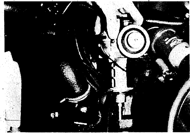
left: If, for some reason, you find it necessary to remove the distributor, first make an illustration like this. It shows the position of the rotor relative to some reference point like the vacuum advance. Since the distributor drive uses helical instead of straight cut gears, the shaft will rotate as it's removed. Unless you know the correct final rotor orientation (by your drawing) you probably won't get the distributor back in correctly. right: This is about the point where the drive gears will begin to mesh. As you go further in, shaft will turn. If you haven't made your drawing, you won't know where the rotor is supposed to be oriented. Also, in some cars, you won't be able to get the distributor all the way in because the drive shaft extension won't mate with the oil pump shaft correctly. Like we said, make that drawing before you pull that distributor!
