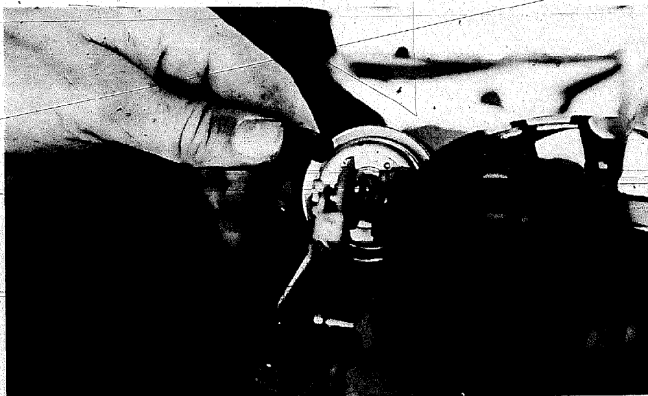
A faulty external vacuum control on a well choke can cause delayed plate openings. If a vacuum control problem is indicated, first check the vacuum hose. If there is vacuum at the hose the unit is faulty and should be replaced.
