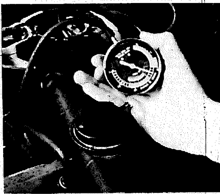
4 If the snorkel of a GM system fails to close when a cold engine is started, check for at least 8 psi of vacuum at the diaphragm unit. Low vacuum means a leaking hose or connection is causing the problem. If the vacuum is sufficient, replace the diaphragm.
