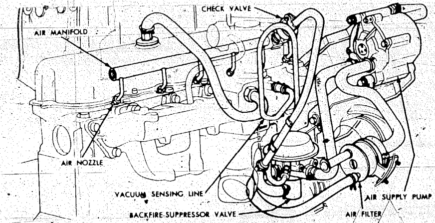
This diagram shows the various units of an AIR system on a six-cylinder engine, using a by-pass type backfire-suppressor valve.
