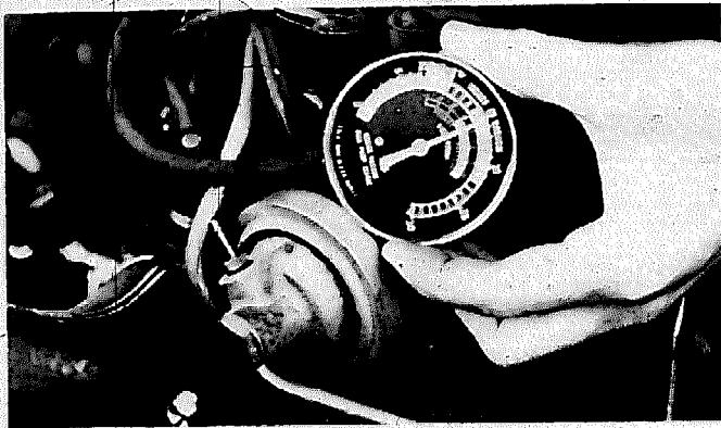
6 Readings at the vacuum advance unit are used to determine if the car's vacuum advance/retard controls are working correctly. Most cars use several of these devices, and a manual should be consulted for the specifics of the devices your car uses.
