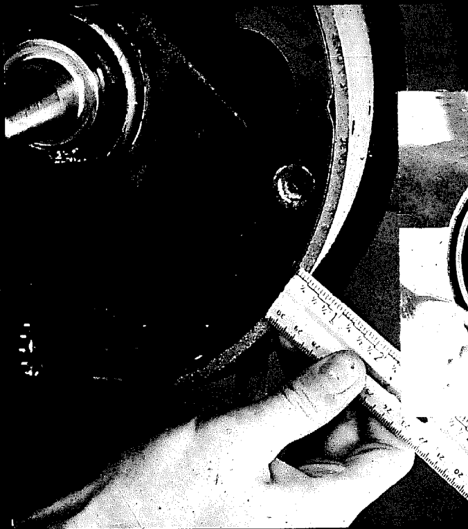
Brakes are one of the most critical areas for inspection. Brake shoes should have at least 1/32-inch of lining above the rivets, or above the shoes on bonded linings. Disc brakes should also be measured for pad thickness—your owner's manual will give the recommended thickness. Brake drums should be evenly worn and free of large scratches or grooves. Worn drums can be machined and reused, but excessively or unevenly worn drums should be replaced.
