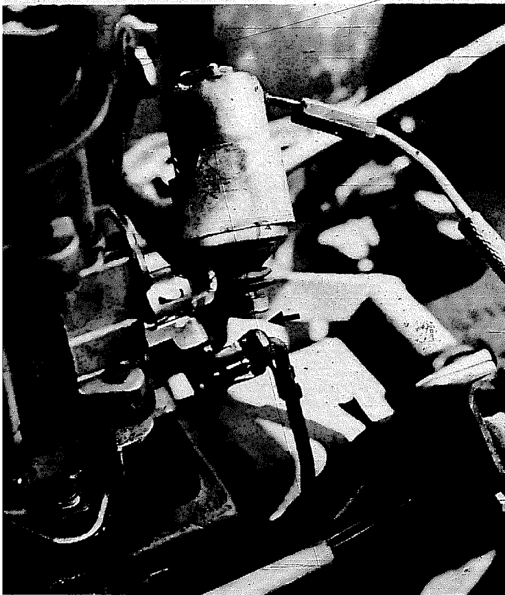
Many 1969 and newer cars use special anti-dieseling devices. The most common is the anti-dieseling solenoid. Solenoids on all cars are essentially the same. With the engine at operating temperature, the solenoid plunger extends against the throttle linkage or throttle-stop screw to maintain engine idle. The plunger should retract when the ignition is shut off. If it doesn't, and the wire to the solenoid is electrically hot, the solenoid must be replaced.
