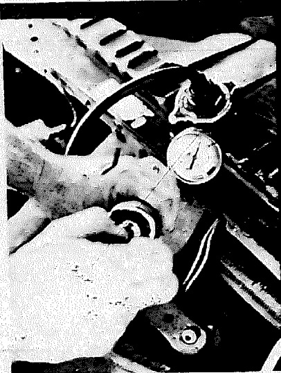
1 The most common type of pressure tester attaches to the radiator filler neck. Pump it until the dial indicates the pressure rating of the system. If the pressure reading drops, there is a leak in the system. Also use the tester to check the radiator cap for a leaking seal.
