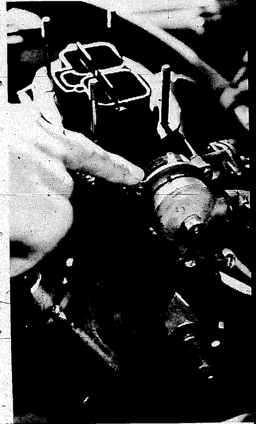
The water-heated choke, used on some late model Ford products, is a very reliable and maintenance-free choke system. Adjustments are made by turning the cover to realign the calibration lines.
