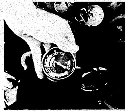
5 The temperature sensor is probably faulty if the snorkel valve doesn't open properly as the engine warms. Lift the air cleaner and check for vacuum at the line which runs from the engine to the sensor. If there is at least 8 psi, replace the sensor.
