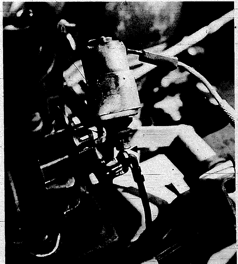
Many 1969 and newer cars use special anti-dieseling devices. The most common is the anti-dieseling solenoid. Solenoids on all cars are essentially the same. With the engine at operating temperature, the solenoid plunger extends against the throttle linkage or throttle-stop screw to maintain engine idle. The plunger should retract when the ignition is shut off. If it doesn't, and the wire to the solenoid is electrically hot, the solenoid must be replaced.
