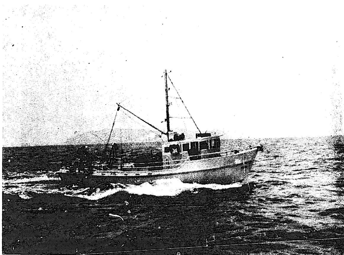
Figure 21. A 48-ft combination trawler at work
