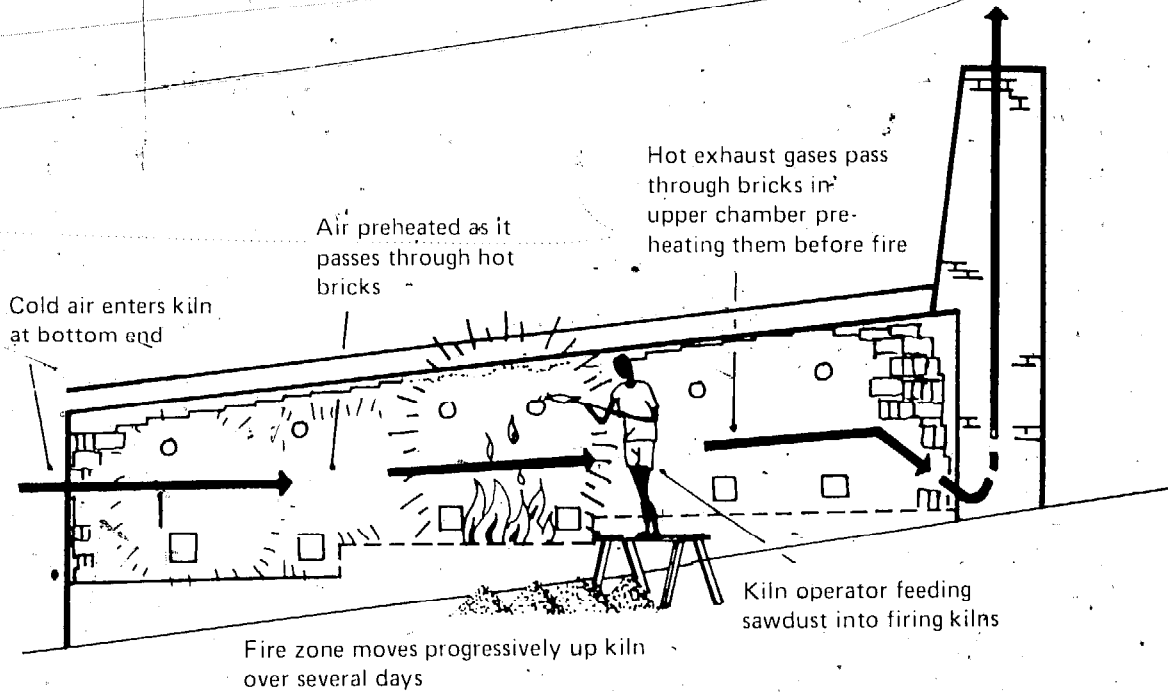
Kiln burner feeding sawdust into Hoffman kiln
