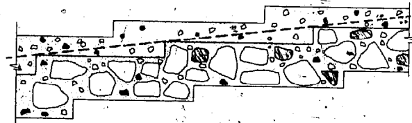
Fig. 47 Stepped foundations.
