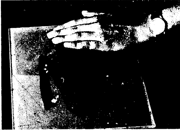
Fig. 8 Testing the plastic limit.
