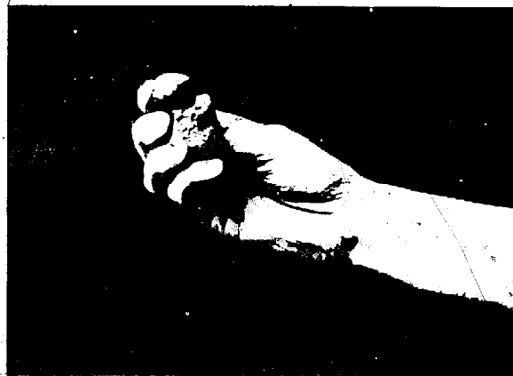
Fig. 14 Dry strength test: pulverizing the ball of soil between the fingers.
