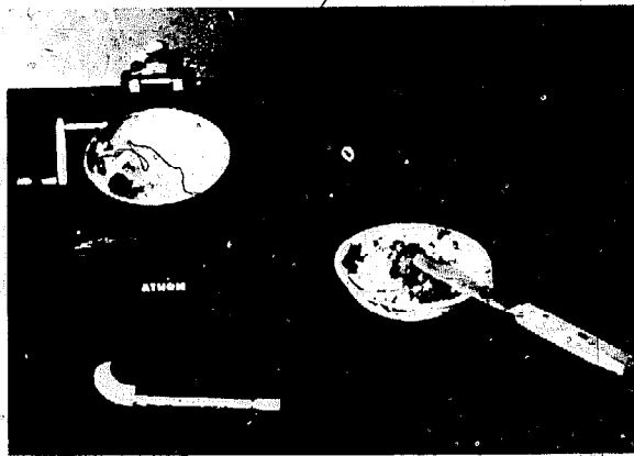
Fig. 7 Testing the liquid limit.
