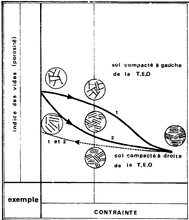
FIGURE 277 : COMPRESSION - DECOMPRESSION
