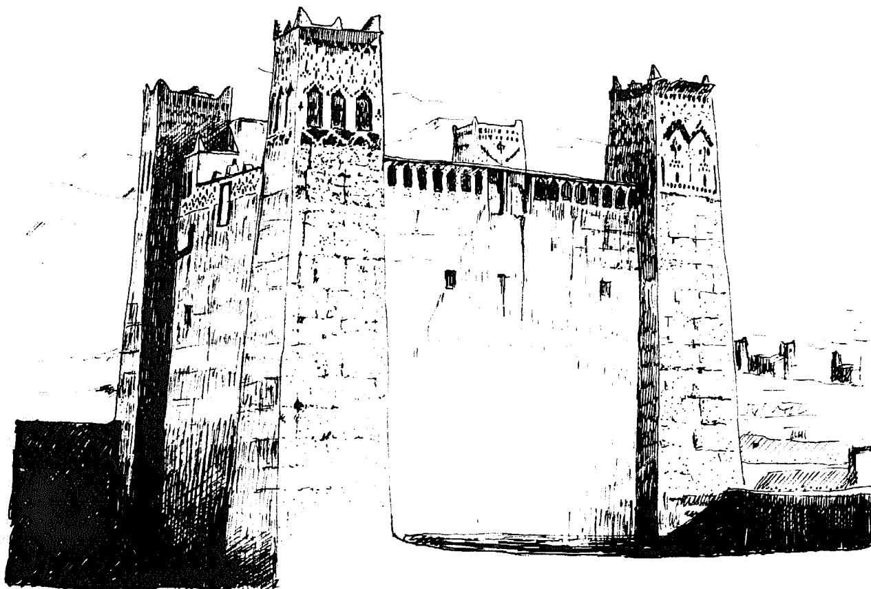
FIGURE 55 : QSAR
