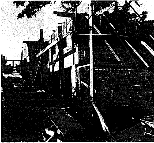
FIGURE 119 : ZERALDA
