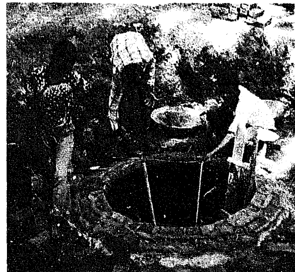
Photo 15: Installing the neck masonry of a fixed-dome (Source: OEKOTOP)
