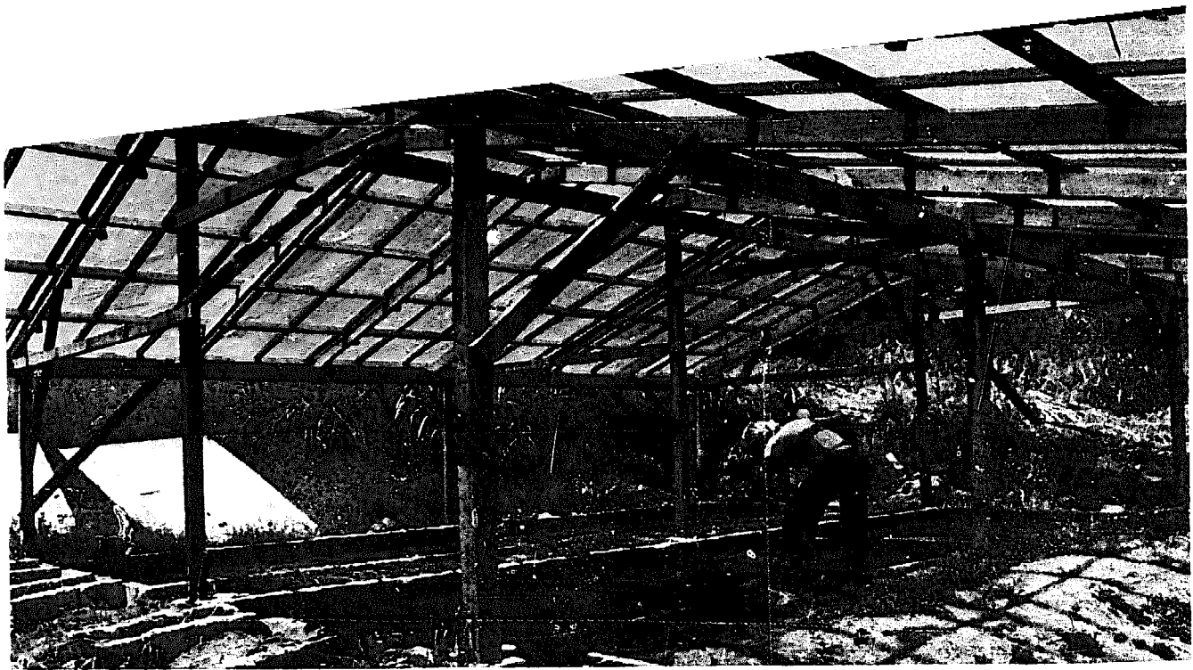
Illustration 2-4: Settling basins.
