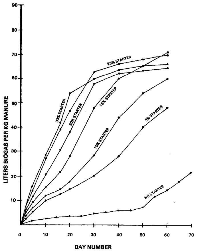
FIG. 3-6 GAS PRODUCTION CURVES FOR VARYING STARTER PERCENTAGE
