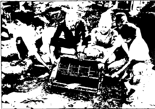
Fig. 10. A cross-flow turbine fabricated by BEW. This 200 mm runner is 560 mm long, the longest runner presently manufactured by BEW. When in use, the turbine's draft tube is connected to the rectangular flange shown.
