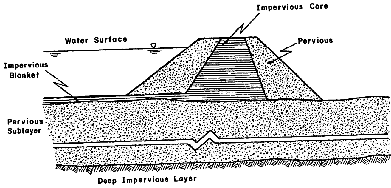
FIGURE II - TREATMENT OF PERVIOUS FOUNDATIONS
