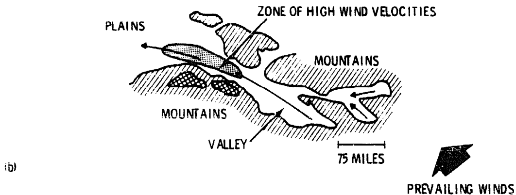
FIGURE 5.14. Possible WECS Sites Where Prevailing Winds are Channeled by Valleys
