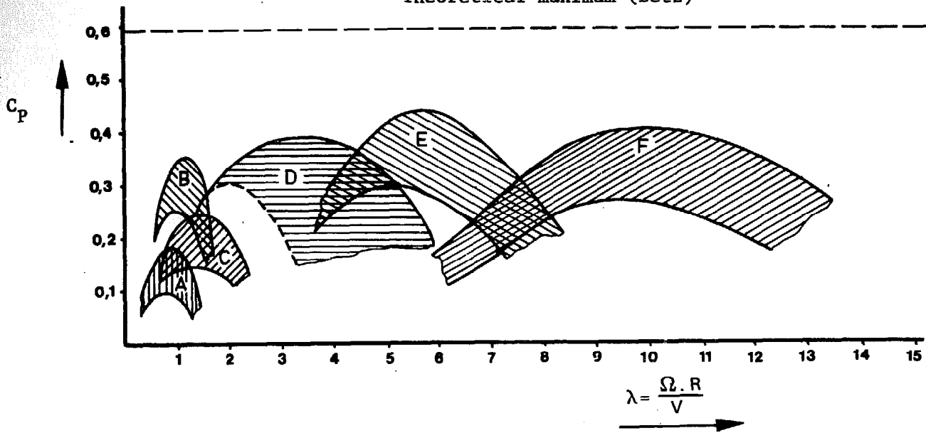
Fig. 4.5. The power coefficient of different types of windrotors as a function of tip speed ratio [8]
