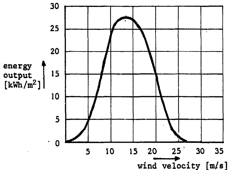
Fig. 3.7. The energy frequency curve of St. Ann's Head (U.K.), derived from fig. 3.6. with P = 0.1 V^3 [W/m 2 ]
