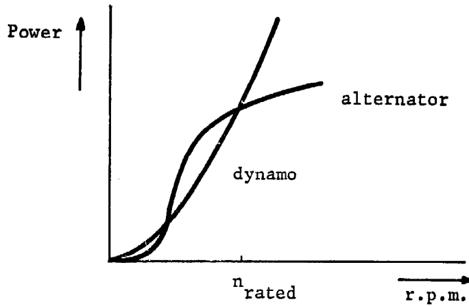
Fig. 4.14. The power output curves of a dynamo and an alternator
