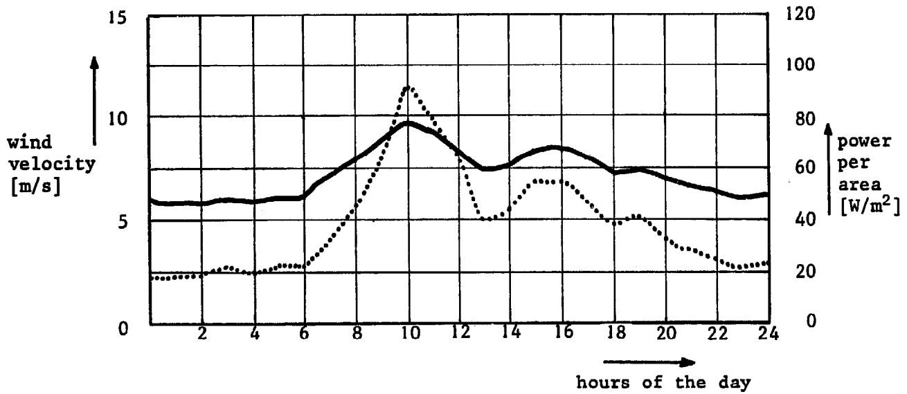
Fig. 3.19. The mean hourly wind speed in Praia (June 1975) during the day. The dotted line indicates the average available power.
