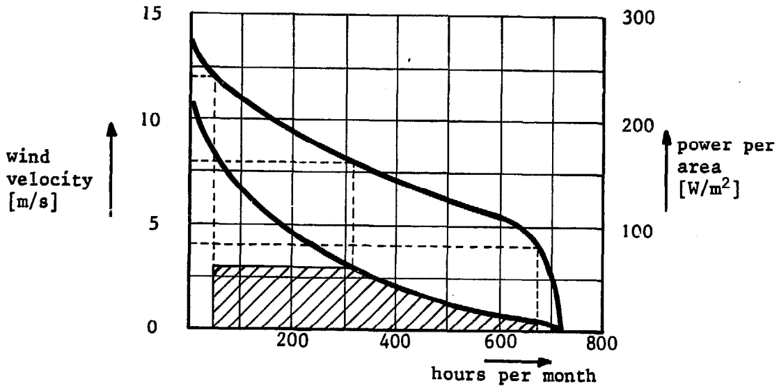
Fig. 3.23. The velocity and power duration curve of Praia (June 1975) with the three design speeds given in case b
