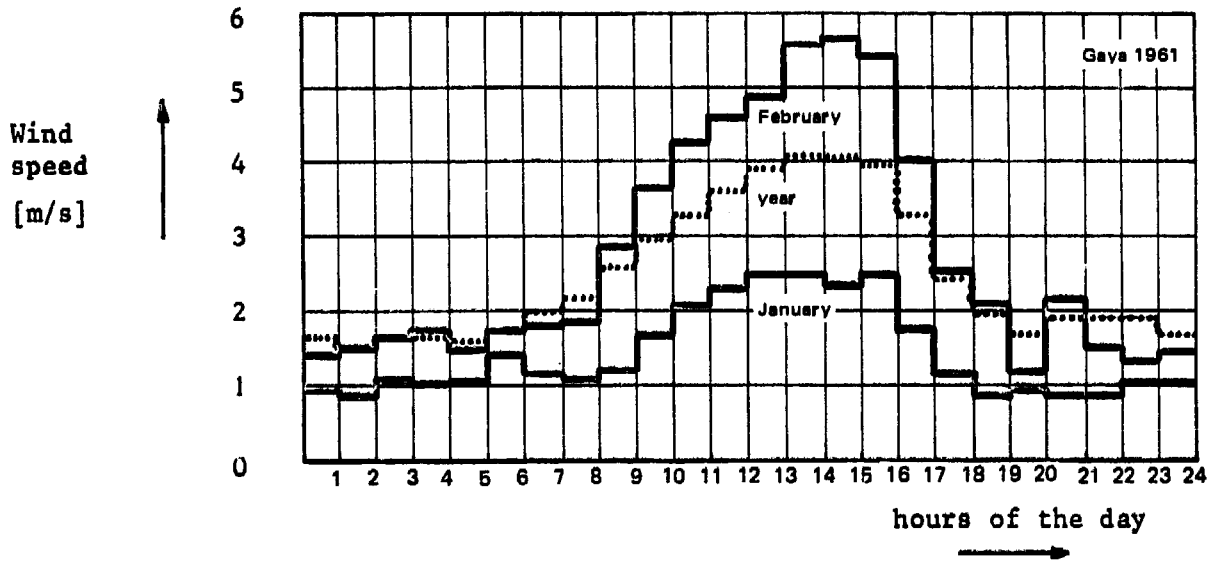
Fig. 3.4. The monthly and annual mean hourly wind speeds during the day at Gaya (India) in 1961. The mean monthly wind speed in January is 1.4 m/s, in February 2.7 m/s, while the mean annual speed is 2.4 m/s.
