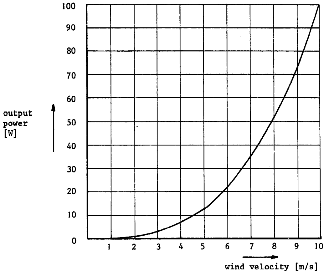
Fig. 3.2. A conservative estimate of the power output from each square metre of area swept by a windrotor: P = 0.1 \times V^3 [W/m 2 ]
