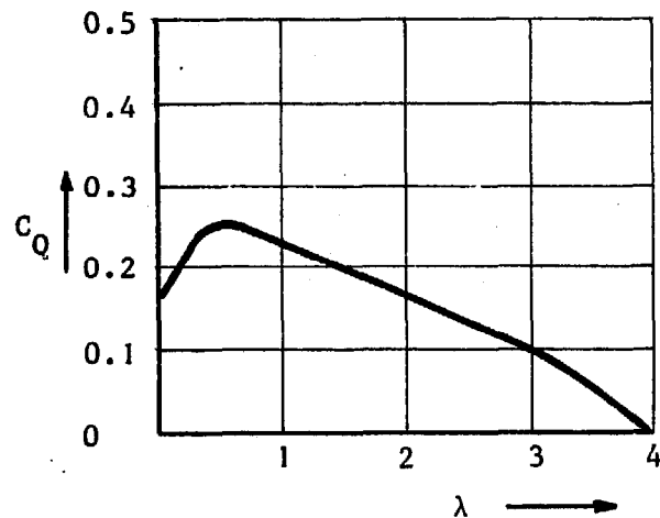
Fig. 4.4. The torque coefficient C_Q of the rotor in fig. 4.1. as a function of tip speed ratio \lambda
