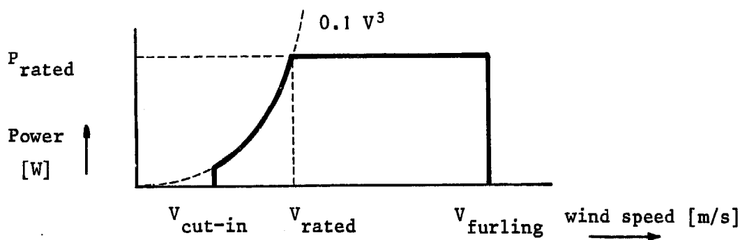
Fig. 3.15. The idealized power output curve of a wind generator
