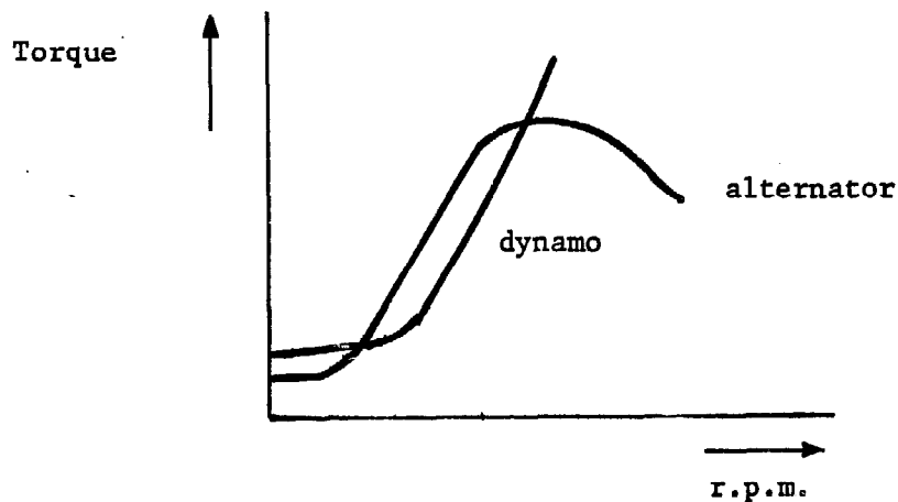
Fig. 4.13. The torque speed curve of a dynamo and an alternator
