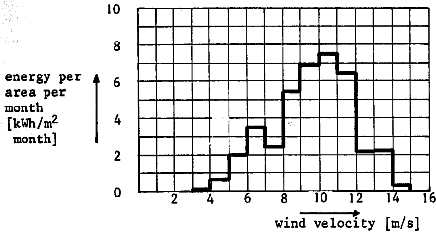
Fig. 3.18. The energy frequency histogram for Praia (June 1975) derived from fig. 3.16.
