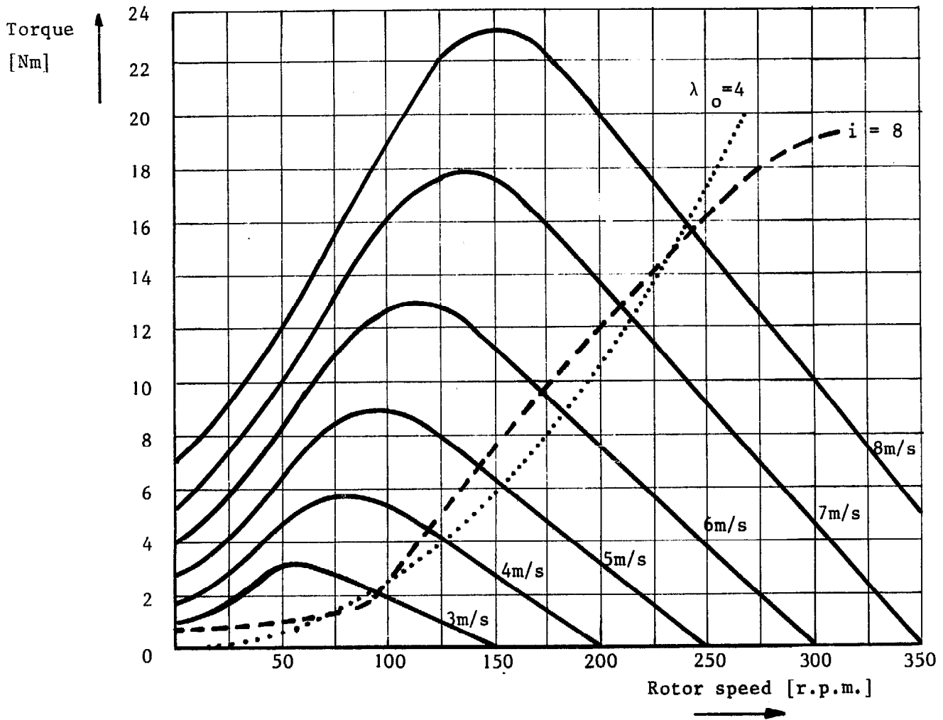
Fig. 4.27. The final torque speed curves of the wind rotor matched with a generator at transmission ratio 1 : 8, as calculated in example 4.3.4.
