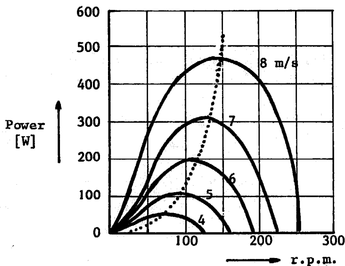
Fig. 4.1. The mechanical power output of a windrotor with four curved metal blades and a diameter of 2.4 m ( A= 4.5m^2 ) as a function of speed for different wind speeds
