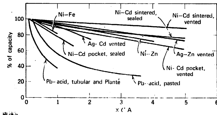
Fig. 5.2. The capacity of different electrolytic cells as a function of multiples of the nominal discharge current.
