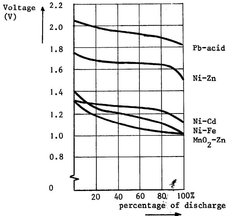
Fig. 5.1. The voltage of electrolytic cells as a function of the percentage of discharge during 5 hours discharging.
