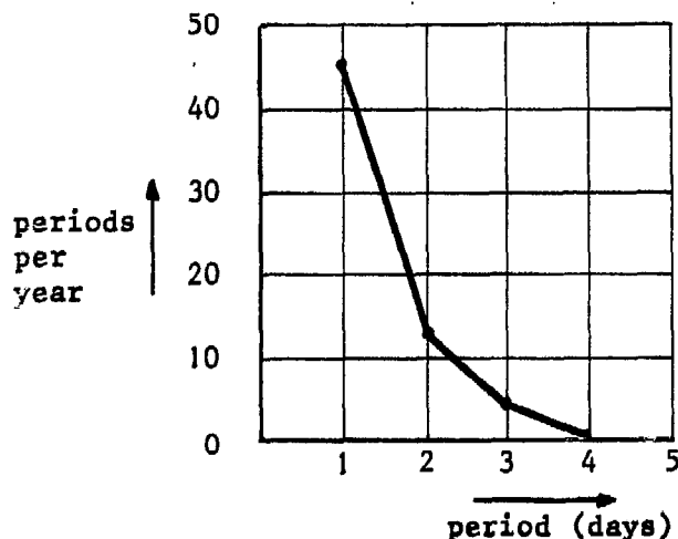
Fig. 3.12. The number of periods per year during which the wind speed was lower than 2 m/s. The data were taken in Bamako, Mali [4].
