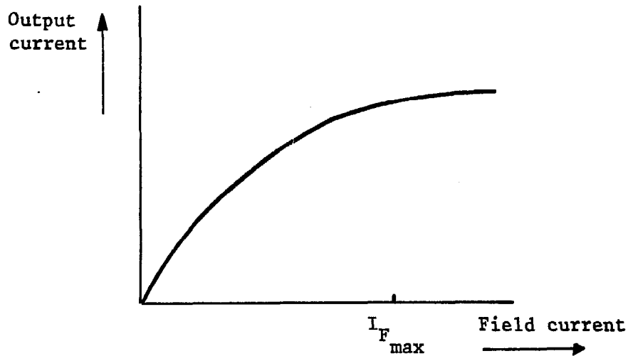
Fig. 4.18. The output current of a generator at fixed speed as a function of field current
