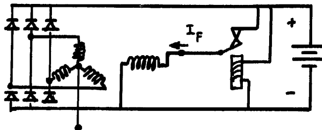
Fig. 4.22. A voltage control relay for a three-phase alternator with rectifiers
