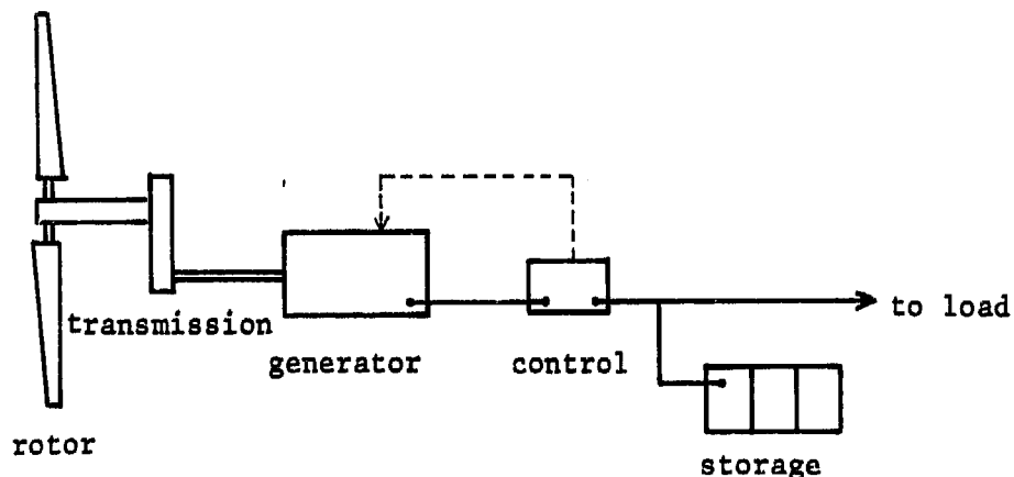
Fig. 2.2. Schematic representation of the energy flow through a wind electricity conversion system
