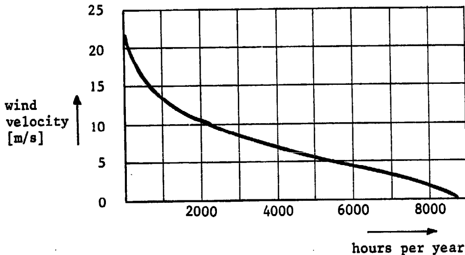
Fig. 3.8. The velocity duration curve of St. Ann's Head (U.K.), derived from fig. 3.6.
