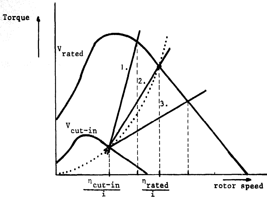
Fig. 4.25(a) The torque speed curves of three different generators are "matched" to a rotor by fixing \lambda = \lambda_0 at V = V_{\text{cut-in}} (see formula 4.10). The generators nr. 1 and nr. 3 do not give the desired result because their speed at V = V_{\text{rated}} is too low, respectively too high. Generator 2 gives a correct matching and will maintain the tip speed ratio approximately at \lambda_0 .
