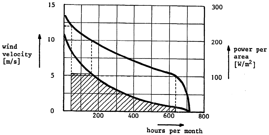
Fig. 3.22. The velocity and power duration curve of Praia (June 1975) with the three design speeds given in case a
