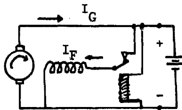
Fig. 4.20(b) Voltage control system with voltage relay (VCR)
