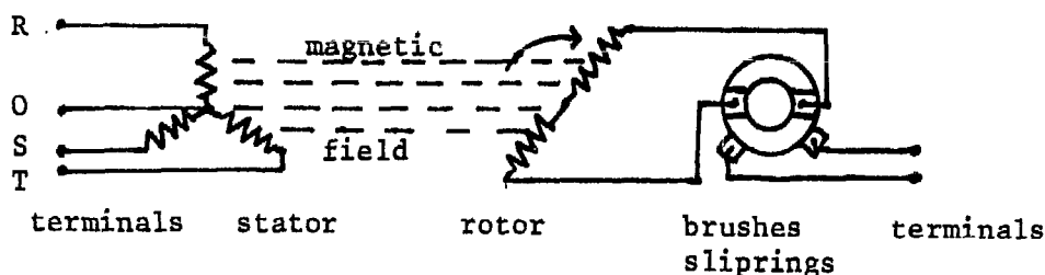
Fig. 4.7. Schematic representation of a three-phase synchronous machine
