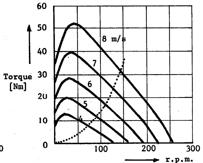
Fig. 4.2. The corresponding torque-speed curves of the rotor in fig. 4.1. for the given wind speeds
