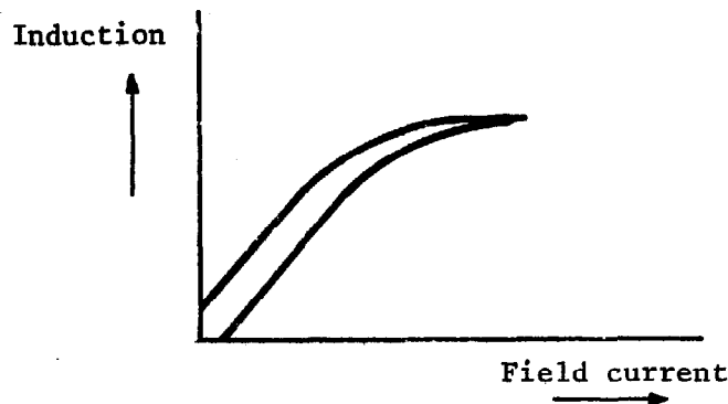
Fig. B.9. Magnetic induction as a function of the field current. The saturation value will be of the order of 1 - 1.5 Tesla.
