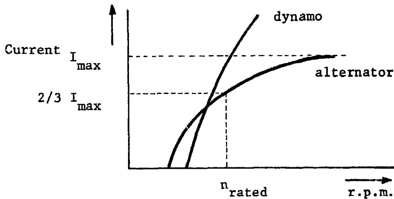
Fig. 4.12. The output current I as a function of the rotational speed of a dynamo and an alternator
