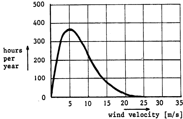
Fig. 3.6. The velocity frequency curve of St. Ann's Head (U.K.) with an annual mean wind speed of 7.2 m/s [5]
