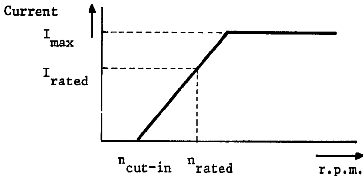
Fig. 4.16. The idealized current speed curve of a generator equipped with a current limiting device
