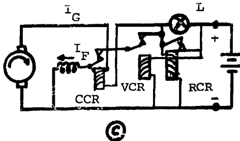
Fig. 4.20(c) Voltage control system with reverse current relay (RCR)
