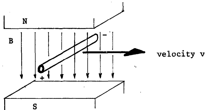
Figure B.2. A moving conductor placed in a magnetic field.
