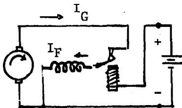
Fig. 4.20(a) Voltage control system with current relay (CCR)
