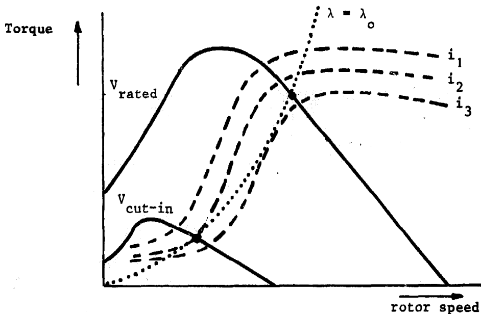
Fig. 4.25(b) The torque speed curve of a generator coupled to a rotor with three different transmission ratios. The calculated transmission ratio i_2 , which is the best choice at V = V_{\text{cut-in}} , turns out to be less good at wind speeds around V_{\text{rated}} . In this case i_3 is a better choice.
