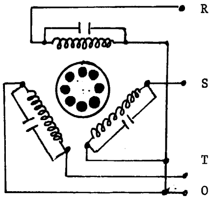
Fig. 4.8. Schematic representation of an asynchronous machine (AM), equipped with capacitors to provide self excitation
