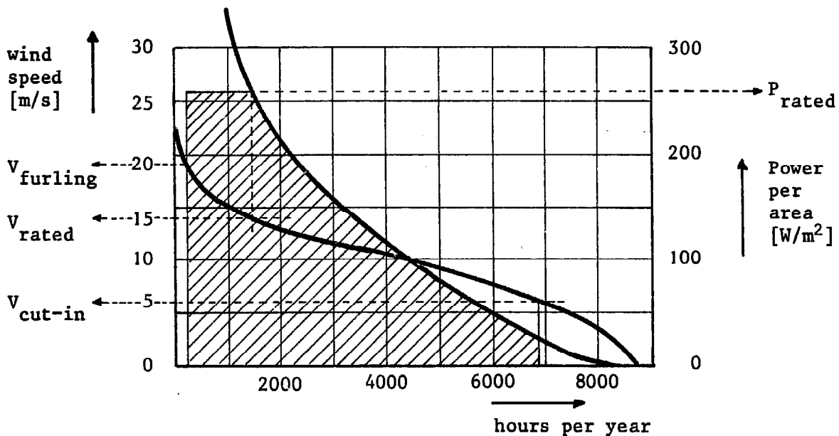
Fig. 3.14. Velocity and power duration curve at Mount Vermont (U.S.A.) with a mean annual wind speed of 9.4 m/s [5]
