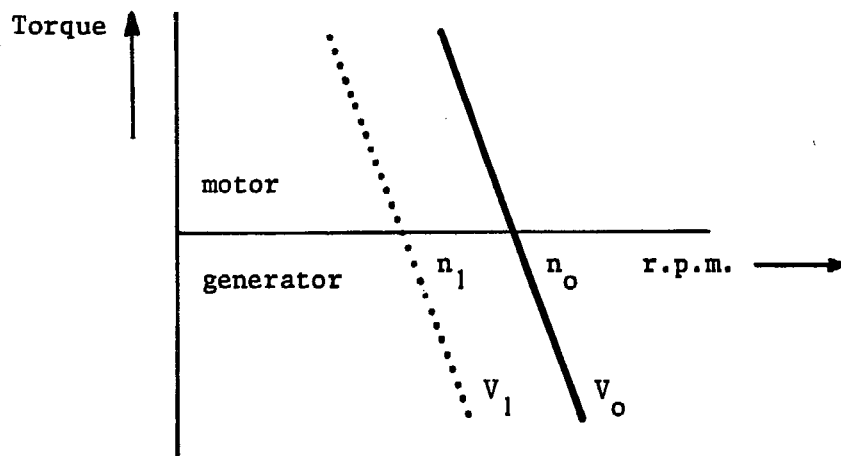
Fig. 4.11. The torque speed curve of a (shunt-wound) commutator machine at two voltages
