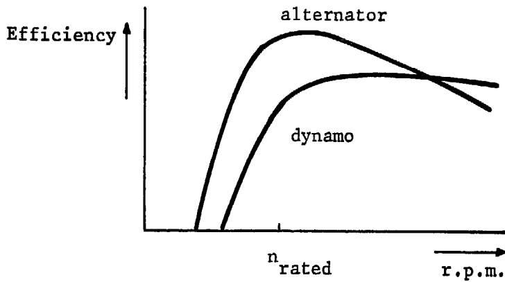
Fig. 4.15. The efficiency speed curve of a dynamo and an alternator
