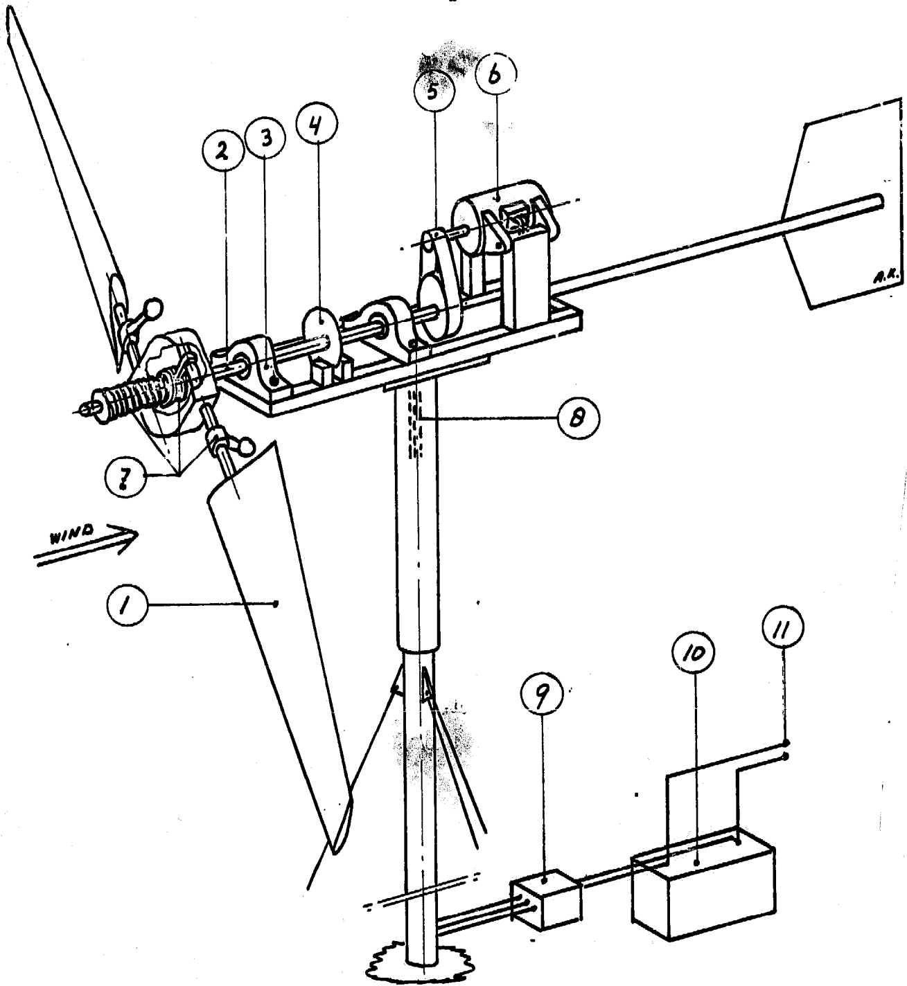
Fig. 2.1. The components of a typical wind-electricity conversion system:
