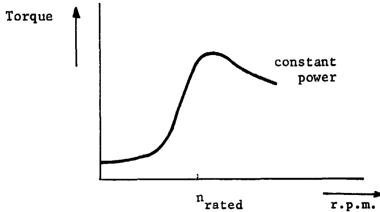
Fig. 4.17. The idealized torque speed curve of a generator
