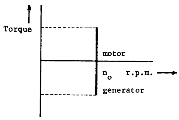
Fig. 4.9. The torque speed curve of a synchronous machine coupled to a strong grid
