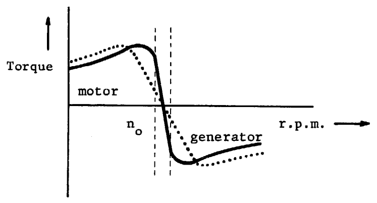
Fig. 4.10. The torque speed curve of an asynchronous machine coupled to a strong grid. Its operating range lies between n_0 + 4\% and n_0 - 4\% . The dotted curve indicates a machine with a resistance in the rotor circuit.
