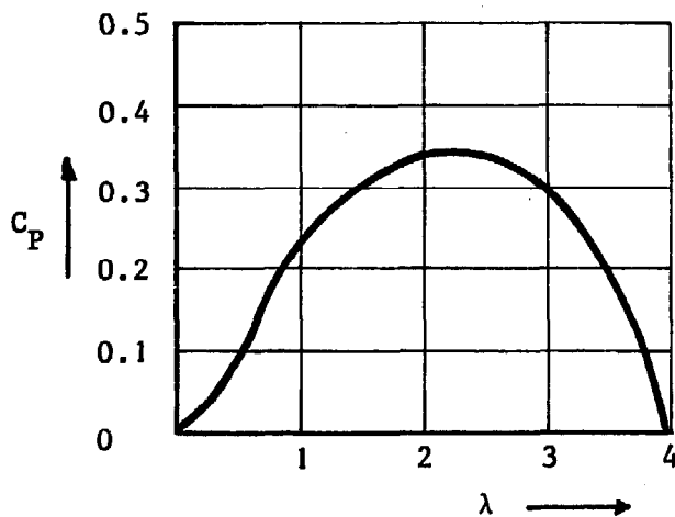
Fig. 4.3. The power coefficient C_P of the rotor in fig. 4.1. as a function of tip speed ratio \lambda
