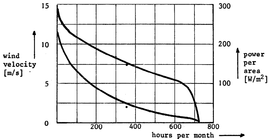
Fig. 3.17. The velocity duration curve (upper) and power duration curve (lower) for Praia (June 1975). The abnormal dip at 7.5 m/s in fig. 3.16. is smoothed out in these curves.
