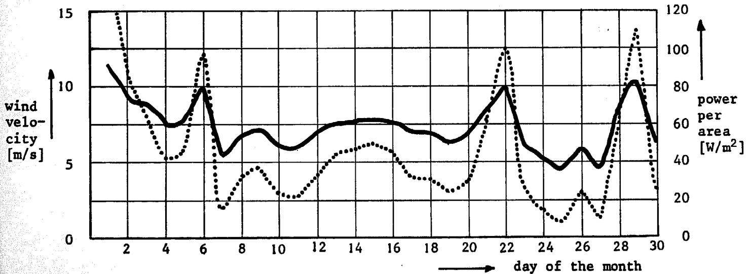
Fig. 3.20. The mean diurnal wind speed in Praia (June 1975). The dotted line indicates the average available power.
