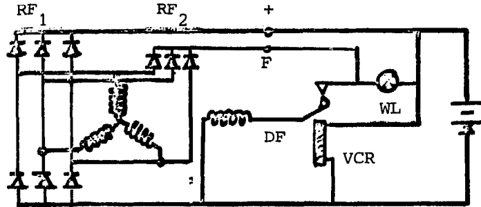
Fig. 4.23. A control system to prevent reverse current at low r.p.m. for an alternator
