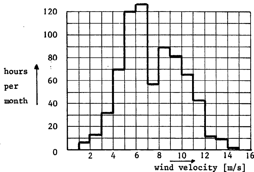
Fig. 3.16. The velocity frequency histogram for Praia (June 1975) derived from the data in table 3.4.
