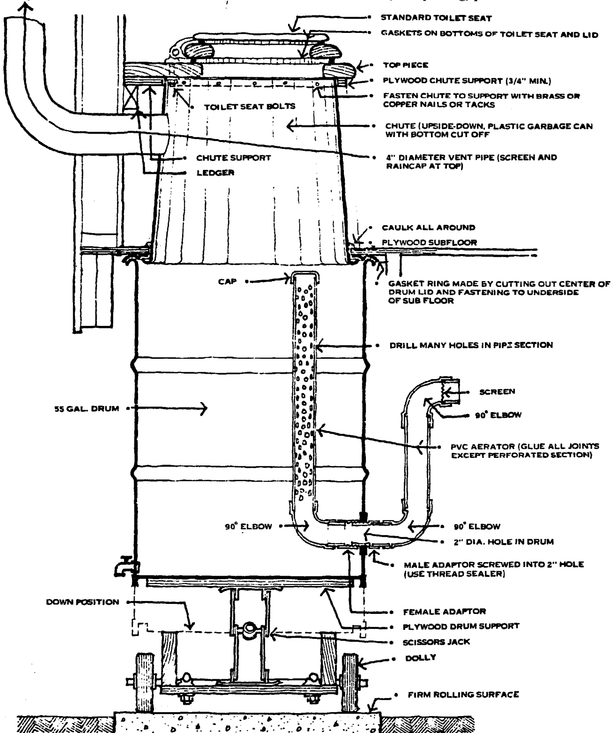
Matson drum privy (from 2135).
