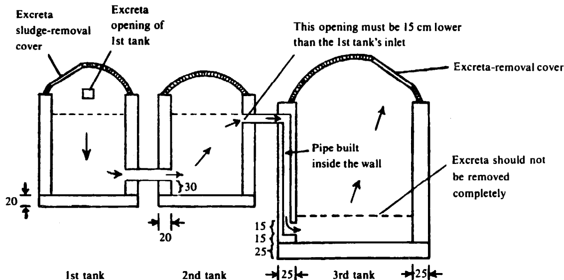
The Chinese three-tank toilet (from 2303).
