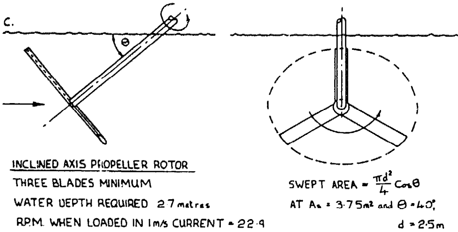
FIGURE 2.7: Sketches of Alternative Turbine Rotors.
