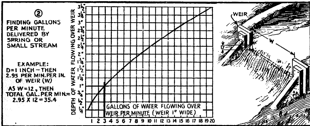
First measure distance D , which is the depth of water flowing over the weir, by the method shown in Fig. 3. Locate this value at the left-hand side of the chart, follow across to the curve, and then drop down where the amount of water in gallons per minute for each inch of weir length is given. Multiplying this number by the length of the weir in inches gives the total amount of water passing over the weir per minute
