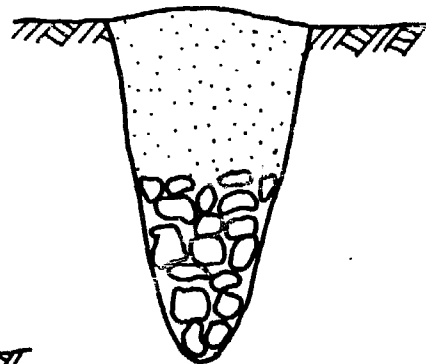
DRAIN TRENCH FILLED WITH RUBBLE
