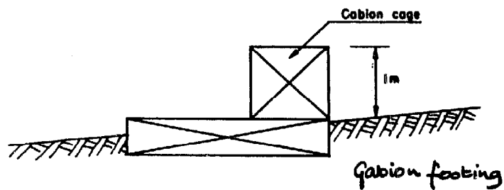
GABION DAM
