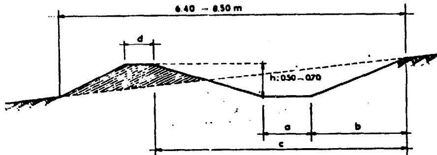
Channel-type flattened cross-section bench terrace (cropping terrace)
