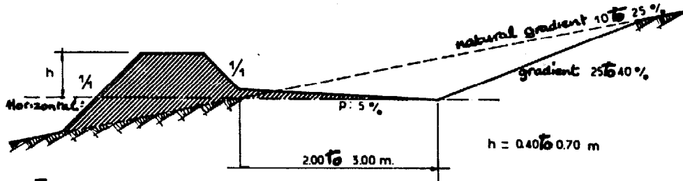
FLATTENED-HUMP TERRACE
