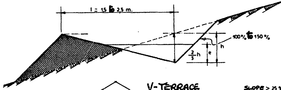
V-TERRACE
