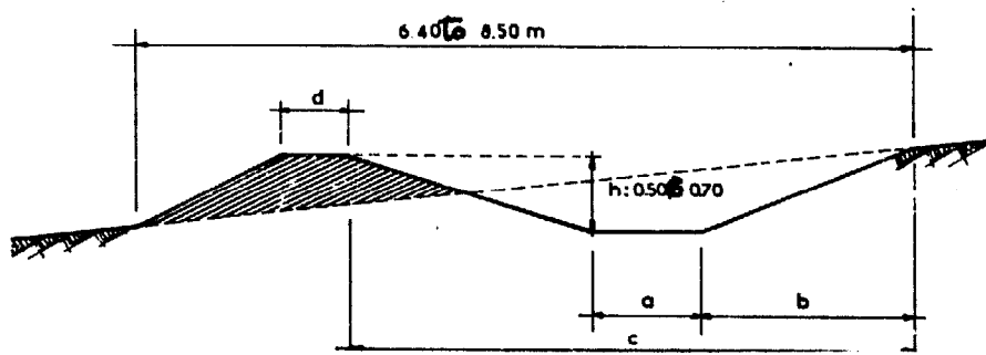
CHANNEL-TYPE FLATTENED CROSS-SECTION TERRACE (CROPPING TERRACE)
