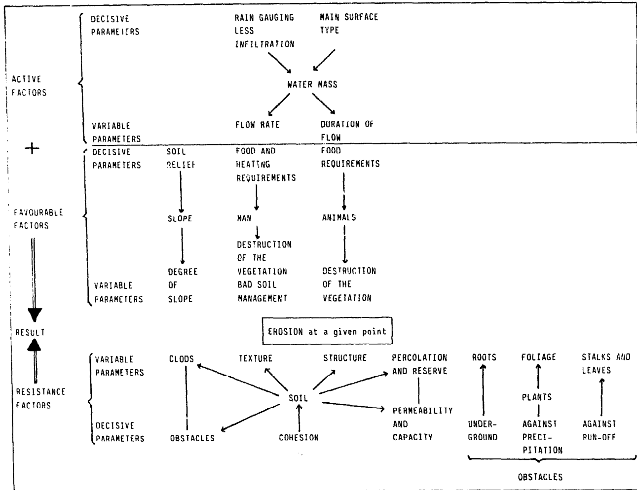
Fig. A.1: Diagram of the main natural factors in run-off erosion
