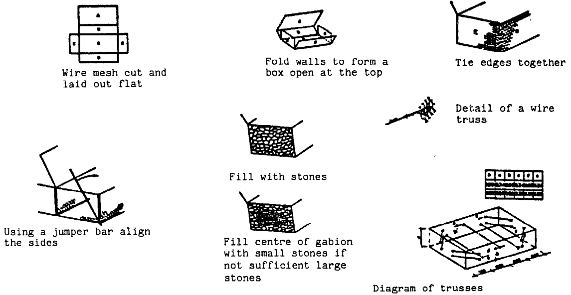
Trusses Gabion 4x1x1
