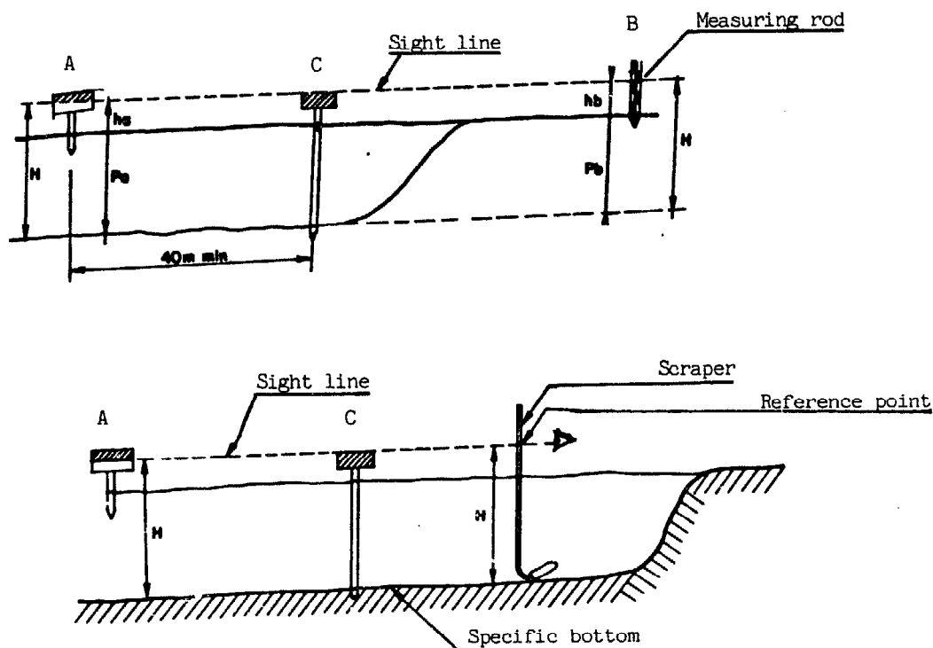
Fig. E.30: Trimming a trench bottom
