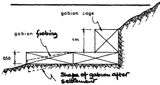
BANK PROTECTION USING GABIONS
