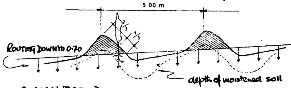
STEPPE METHOD
