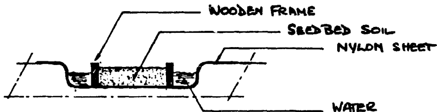
Soak-irrigated seedbed
