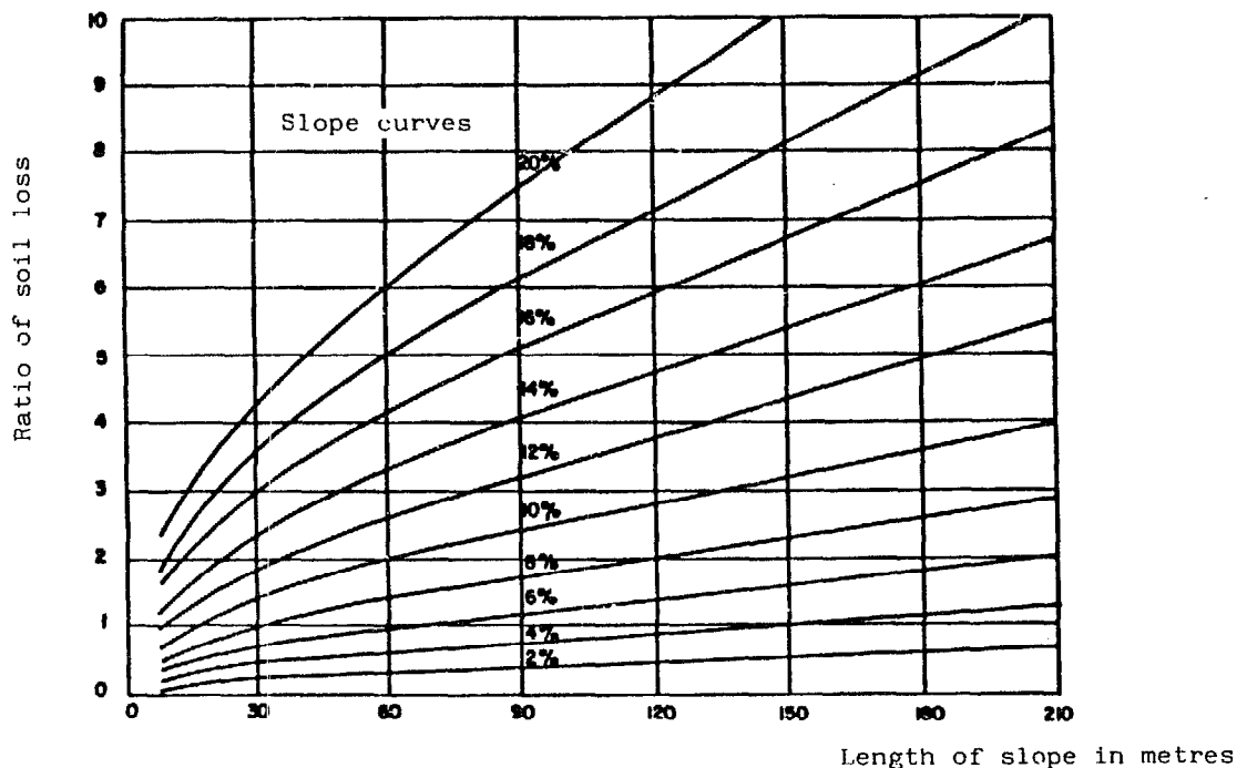
Fig. A.2: Wischmeier's universal equation (graph giving the values of the factor L.S as a function of the length and percentage of the slope (ref. 23))
