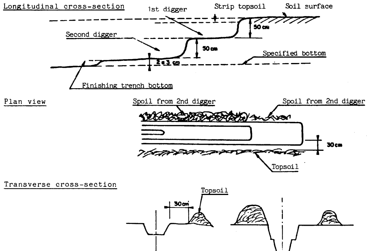
Fig. E.29: Digging a drainage trench
