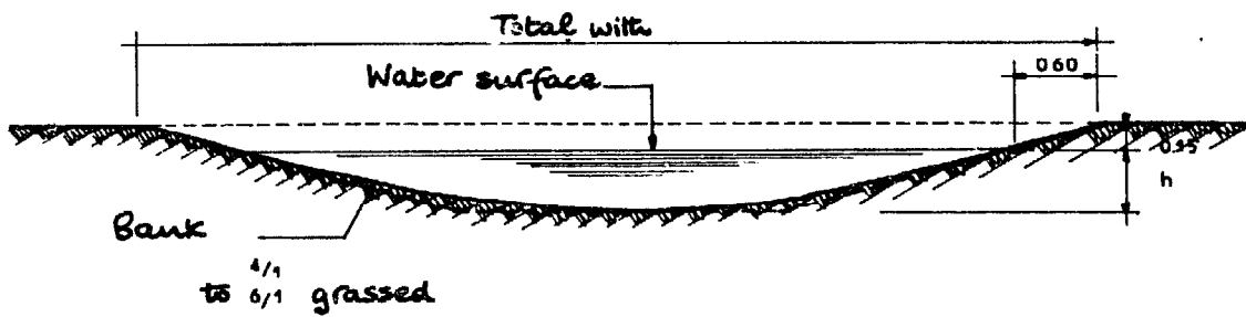
VALUES OF h AS A FUNCTION OF THE SPEED AND THE GRADIENT (in metres)
