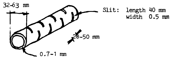
Rigid PVC drainpipe
