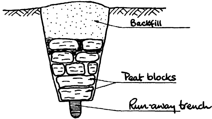
PEAT DRAIN
