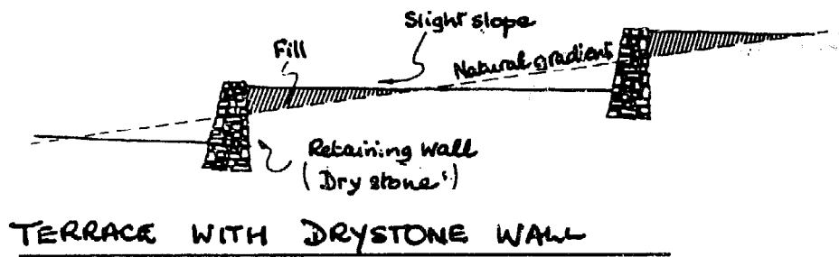
IRRIGATION TERRACE
