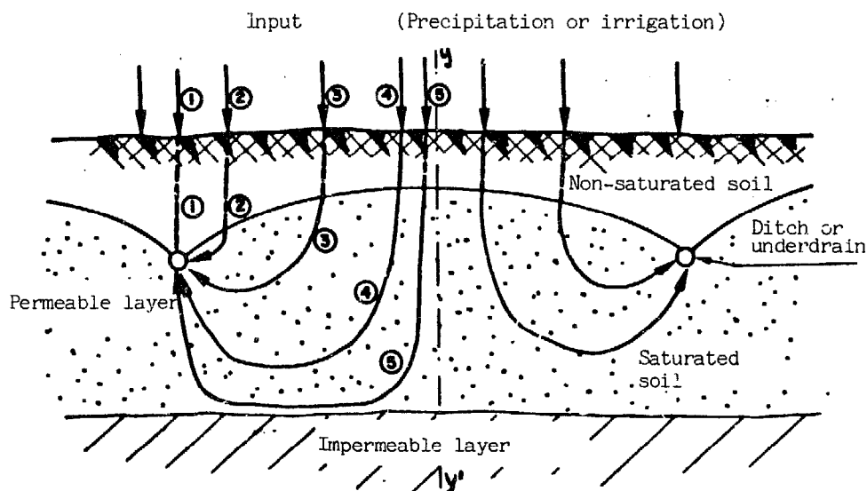
Fig. C.2: Water movement in drained soil
