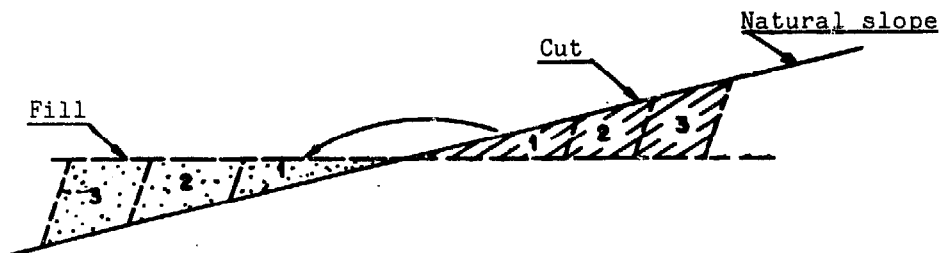
Fig. E.19: Terrace construction
