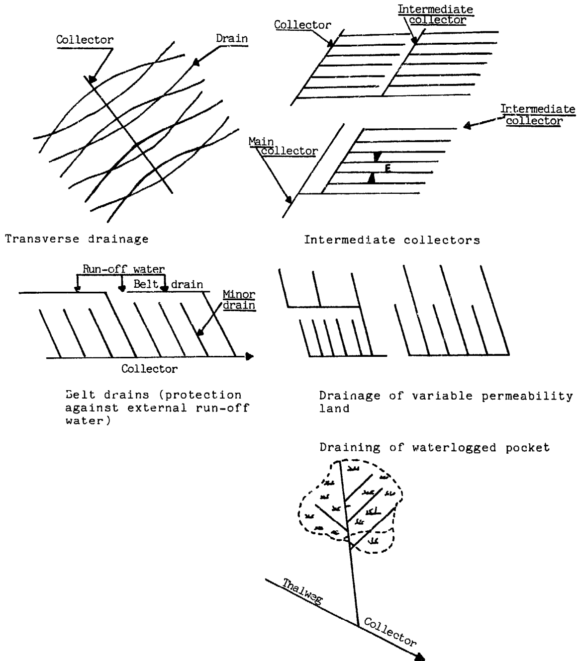
Fig. C.7: Layout of a drainage network
