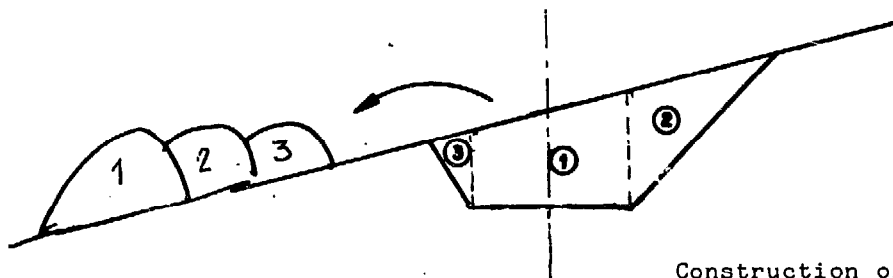
Construction of a protection ditch with spoil thrown downhill
