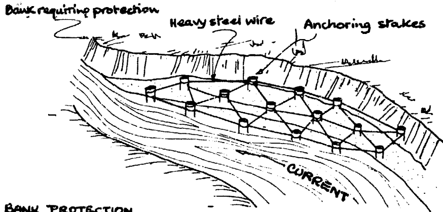
BANK PROTECTION BY ANCHORING STAKES intertwined with steel wire
