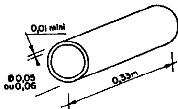
EARTHENWARE DRAINPIPE
