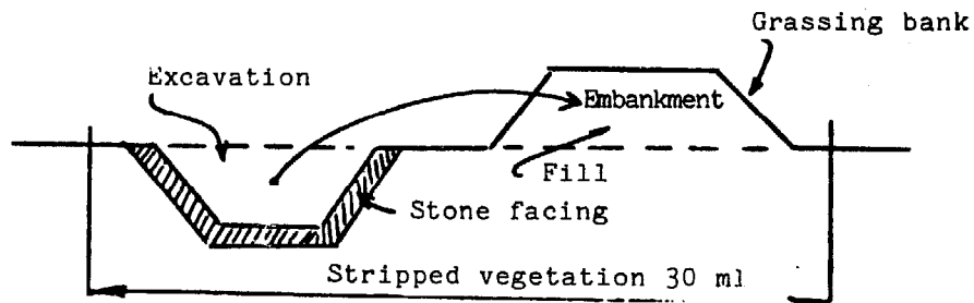
Fig. E.1: Cross-section of channel and embankment
