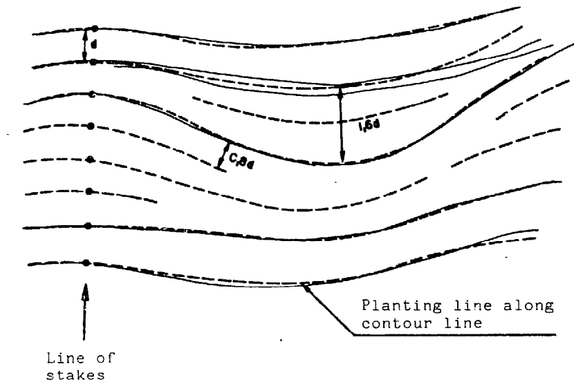
Fig. E.27: Planting along contour lines
