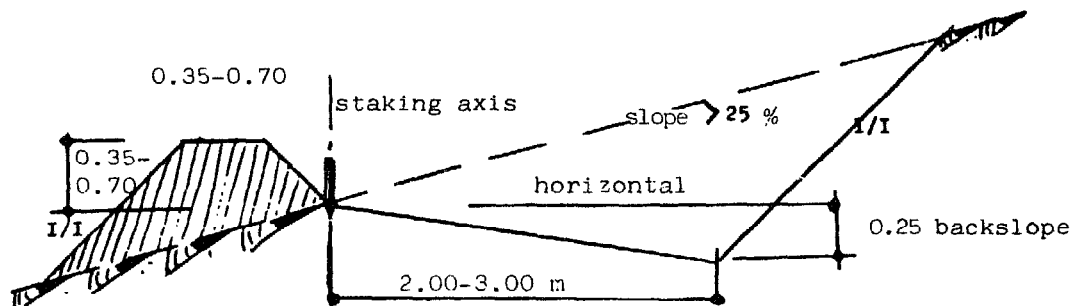
Normal cross-section terrace (Algerian type)
