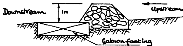
DRYSTONE AND GABION DAM
