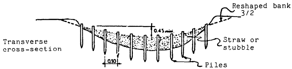
Pile and straw weir
