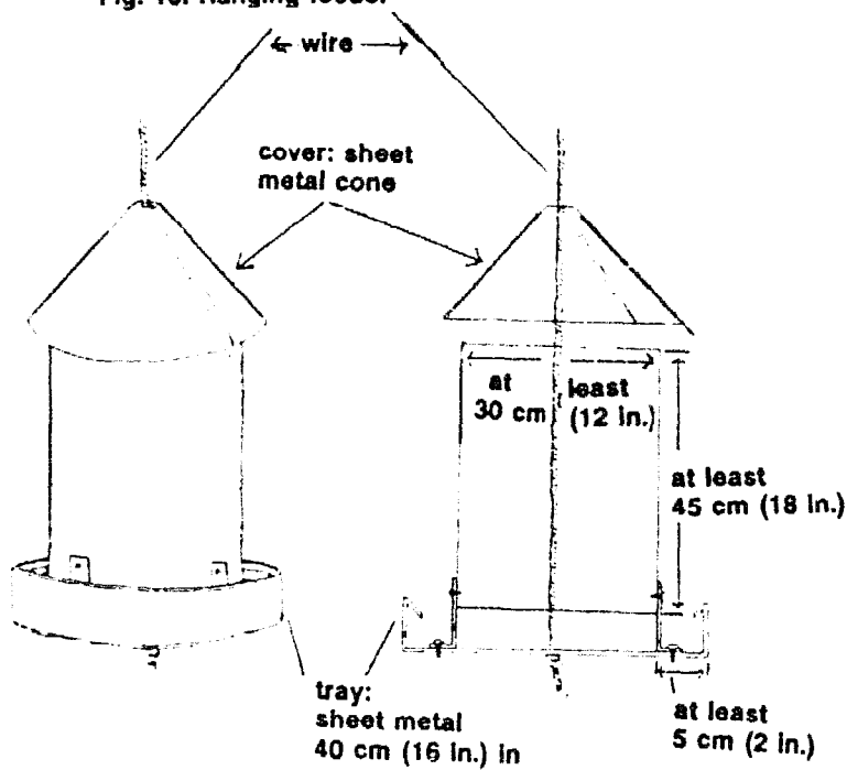
Fig. 15. Hanging feeder
