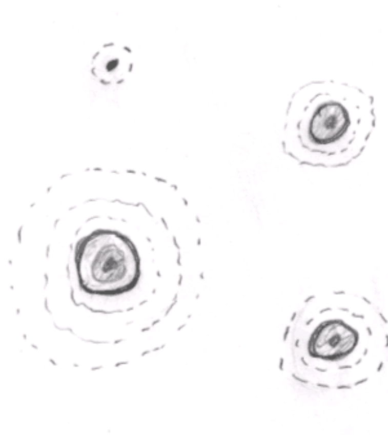
Figure 9. Holonic Matter and Energy.
