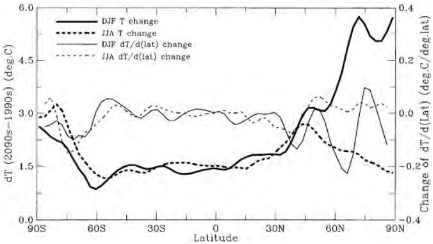
Fig. 10.24 Latitudinal distribution of predicted changes of the zonally averaged surface air temperature from the 1990s to the 2090s for Northern Hemisphere winter (DJF: heavy solid curve) and Northern Hemisphere summer (JJA: heavy dashed curve) for a scenario with approximate doubling of the atmospheric carbon dioxide concentration. Also shown as light curves (right side ordinate) are changes (2090s minus 1990s) of the pole to equator temperature gradient in ^{\circ}\text{C} per degree of latitude. (After Dai et al., 2001.)
