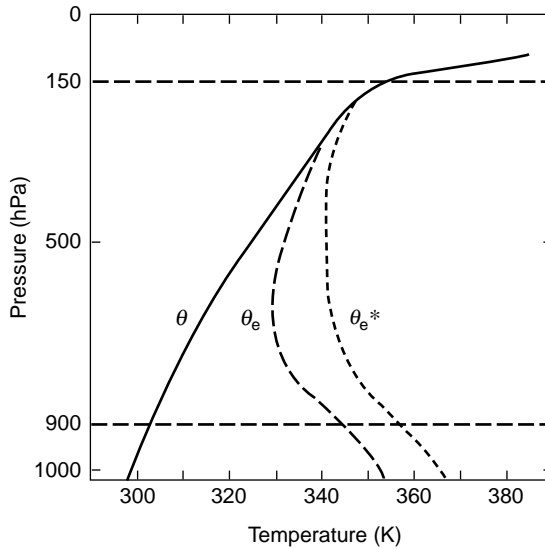
Fig. 11.1 Typical sounding in the tropical atmosphere showing the vertical profile of potential temperature \theta , equivalent potential temperature \theta_e , and the equivalent potential temperature \theta_e^* of a hypothetically saturated atmosphere with the same temperature at each level. This figure should be compared with Fig. 9.10, which shows similar profile for a midlatitude squall line sounding. (After Ooyama, 1969. Reproduced with permission of the American Meteorological Society.)
