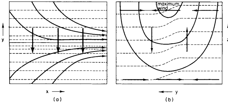
Fig. 9.3 (a) Horizontal streamlines, isotherms, and \mathbf{Q} vectors in a frontogenetic confluence (b) Vertical section across the confluence showing isotachs (solid), isotherms (dashed), and vertical and transverse motions (arrows). (After Sawyer, 1956.)
