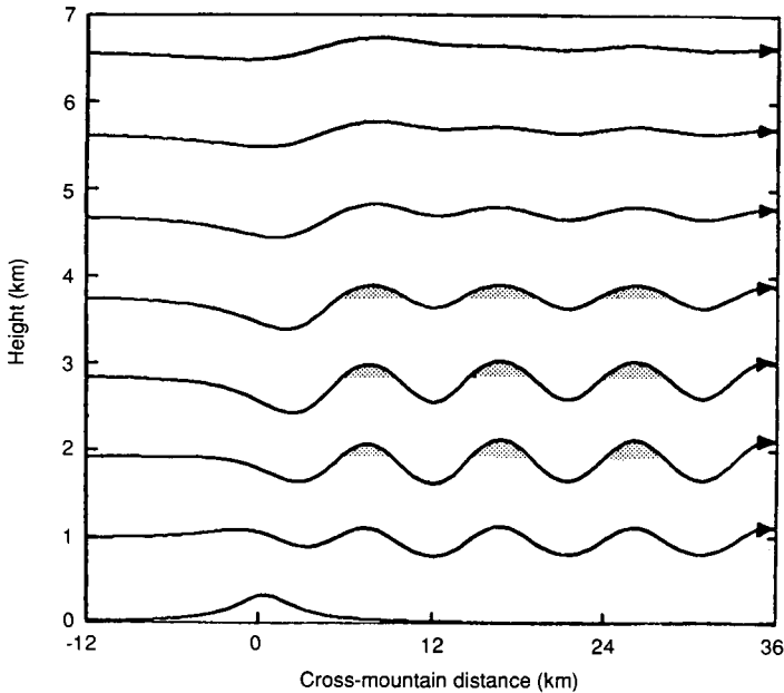
Fig. 9.8 Streamlines for trapped lee waves generated by fl w over topography with vertical variation of the Scorer parameter. Shading shows locations where lee wave clouds may form. (After Durran, 1990.)
