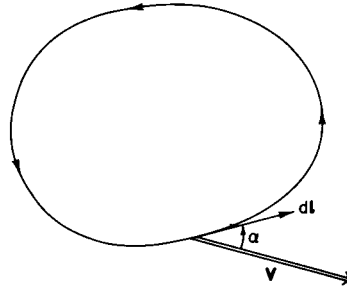
Fig. 4.1 Circulation about a closed contour.
