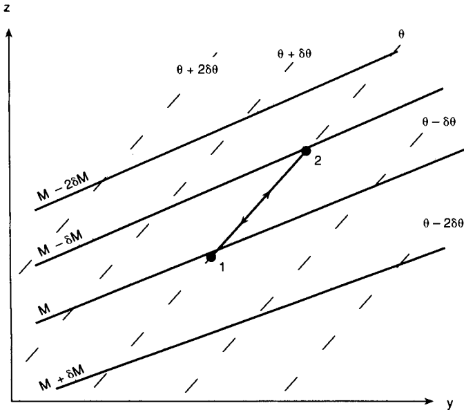
Fig. 9.6 Cross section showing isolines of absolute momentum and potential temperature for a symmetrically unstable basic state. Motion along the isentropic path between points labeled 1 and 2 is unstable, as M decreases with latitude along the path. See text for details.
