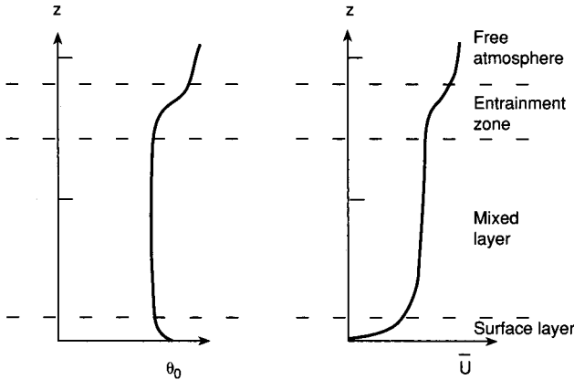
Fig. 5.2 Mean potential temperature, \theta_0 , and mean zonal wind, U , profile in a well-mixed boundary layer. Adapted from Stull (1988).
