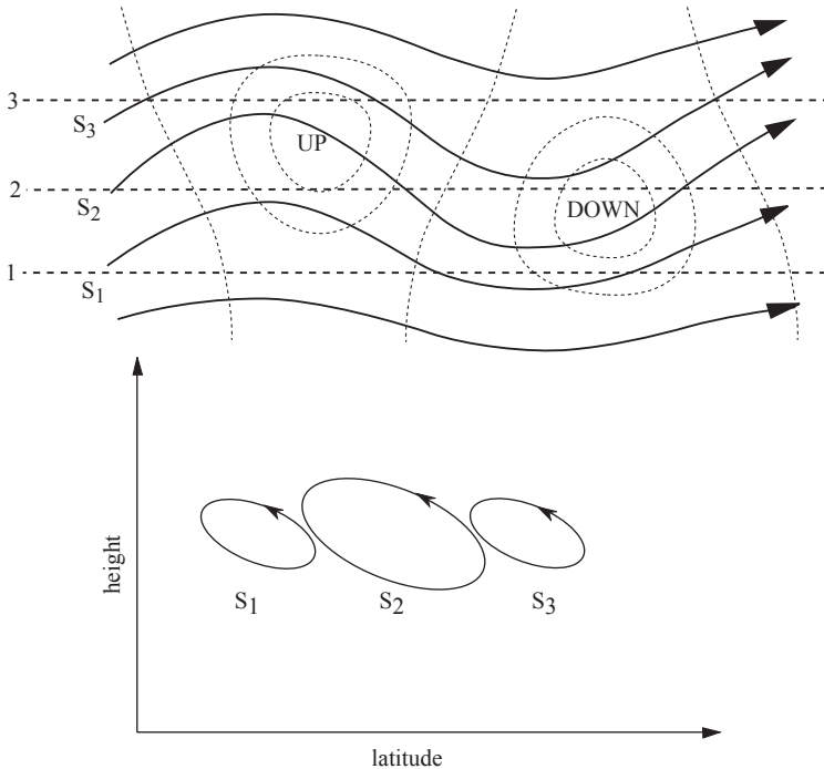
Fig. 12.5 Parcel motions for an adiabatic planetary wave in a westerly zonal fl w. (a) Solid lines labeled S_1 , S_2 , S_3 , are parcel trajectories, heavy dashed lines are latitude circles, and light dashed lines are contours of vertical velocity field (b) Projection of parcel oscillations on the meridional plane.
