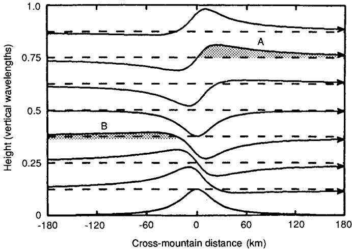
Fig. 9.7 Streamlines of fl w over a broad isolated ridge showing upstream phase tilt with height. The pattern is periodic in height and one vertical wavelength is shown. Orographic clouds may form in the shaded areas where streamlines are displaced upward from equilibrium either upstream or downstream of the ridge if sufficient moisture is present. (After Durran, 1990.)
