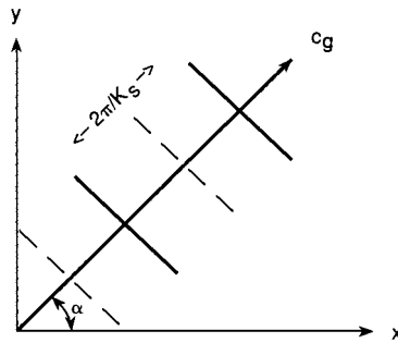
Fig. 10.14 Stationary plane Rossby wave in a westerly fl w. Ridges (solid lines) and troughs (dashed lines) are oriented at an angle \alpha to the y axis, and the group velocity relative to the ground, c_{g_s} , is oriented at an angle \alpha to the x axis. The wavelength is 2\pi/K_s . (Adapted from Hoskins, 1983.)
