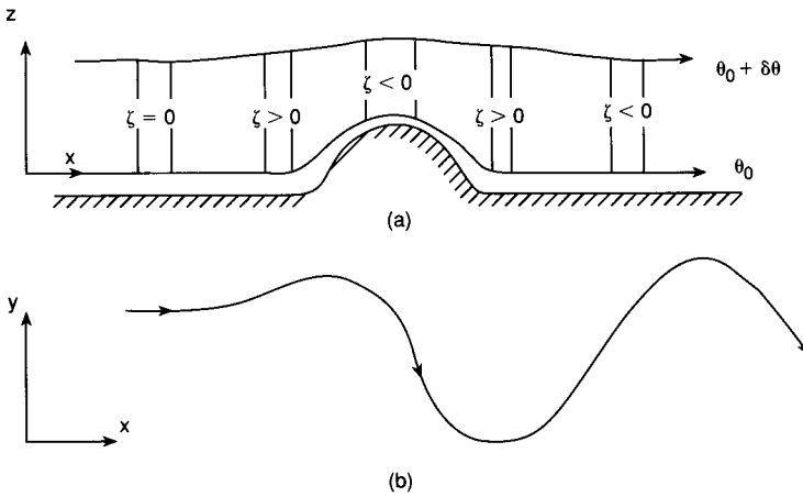
Fig. 4.9 Schematic view of westerly fl w over a topographic barrier: (a) the depth of a fluid column as a function of x and (b) the trajectory of a parcel in the (x, y) plane.
