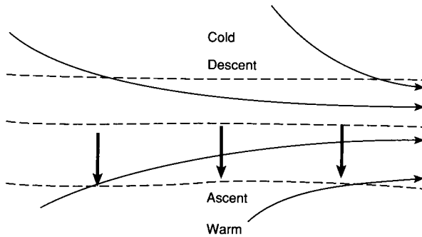
Fig. 6.14 Orientation of \mathbf{Q} vectors (bold arrows) for confluent (jet entrance) fl w. Dashed lines are isotherms. (After Sanders and Hoskins, 1990.)
