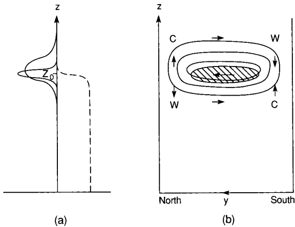
Fig. 12.11 Schematic of transient wave, mean-fl w interactions occurring during a stratospheric warming. (a) Height profile of EP flu (dashed), EP flu divergence (heavy line), and mean zonal fl w acceleration (thin line); z_0 is the height reached by the leading edge of the wave packet at the time pictured. (b) Latitude–height cross section showing region where the EP flu is convergent (hatched), contours of induced zonal acceleration (thin lines), and induced residual circulation (arrows). Regions of warming (W) and cooling (C) are also shown. (After Andrews et al., 1987.)
