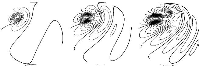
Fig. 10.15 The vorticity pattern generated on a sphere when a constant angular velocity westerly fl w impinges on a circular forcing centered at 30^\circ\text{N} and 45^\circ\text{W} of the central point. Left to right, the response at 2, 4, and 6 days after switch on of the forcing. Five contour intervals correspond to the maximum vorticity response that would occur in 1 day if there were no wave propagation. Heavy lines correspond to zero contours. The pattern is drawn on a projection in which the sphere is viewed from infinit . (After Hoskins, 1983.)
