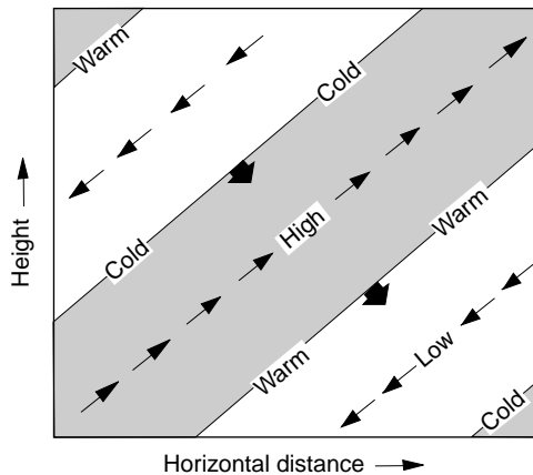
Fig. 7.9 Idealized cross section showing phases of pressure, temperature, and velocity perturbations for an internal gravity wave. Thin arrows indicate the perturbation velocity field blunt solid arrows the phase velocity. Shading shows regions of upward motion.
