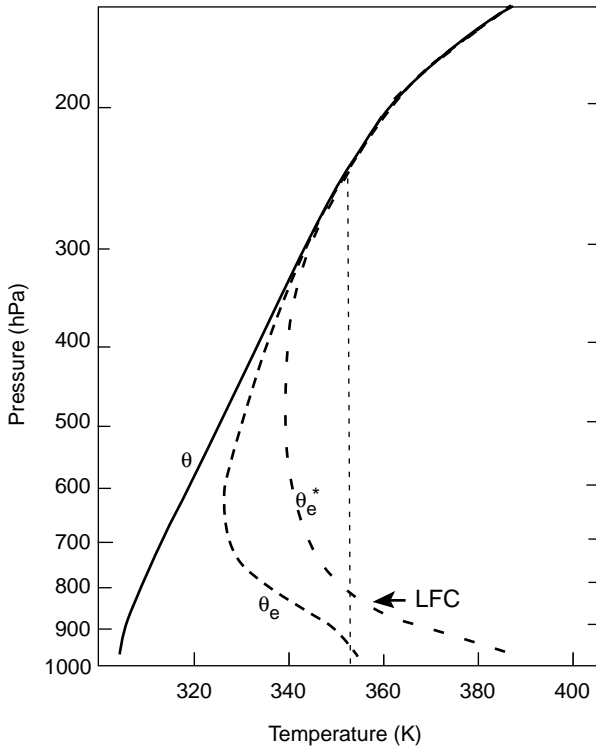
Fig. 9.10 Schematic sounding for a conditionally unstable environment characteristic of Midwestern North America thunderstorm conditions showing the vertical profile of potential temperature, \theta , equivalent potential temperature, \theta_e , and the equivalent temperature, \theta_e^* , of a hypothetically saturated atmosphere with the same temperature profile. Dotted line shows \theta_e for a nonentraining parcel raised from the surface. Arrow denotes the LFC for the parcel.
