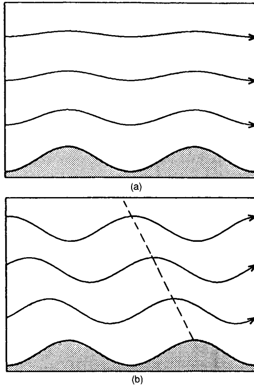
Fig. 7.10 Streamlines in steady fl w over an infinit series of sinusoidal ridges for the narrow ridge case (a) and broad ridge case (b). The dashed line in (b) shows the phase of maximum upward displacement. (After Durran, 1990.)
