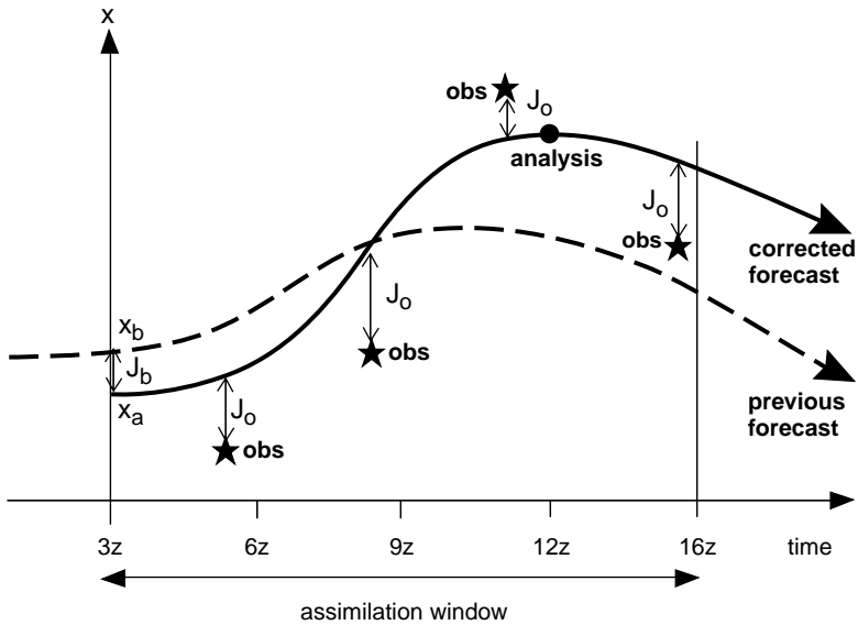
Fig. 13.8 The ECMWF data assimilation process. Vertical axis indicates the value of an atmospheric field variable. The curve labeled x_b is the first guess or “background” field and x_a is the analysis field. J_b indicates the misfit between the background and analysis fields. Stars indicate the observations, and J_o designates the “cost function,” a measure of the misfit between the observations and the analysis, which along with J_b is minimized to produce the best estimate of the state of the atmosphere at the analysis time (Courtesy ECMWF.)
