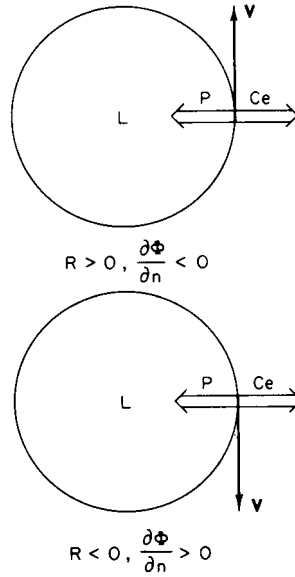
Fig. 3.4 Force balance in cyclostrophic fl w: P designates the pressure gradient and C_e the centrifugal force.
