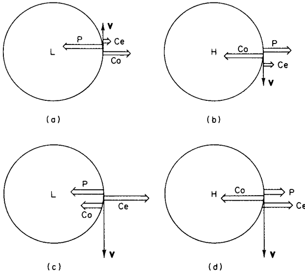
Fig. 3.5 Force balances in the Northern Hemisphere for the four types of gradient fl w: (a) regular low (b) regular high (c) anomalous low (d) anomalous high.
