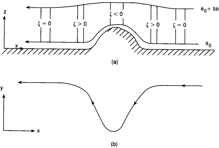
Fig. 4.10 As in Fig. 4.9, but for easterly fl w.
