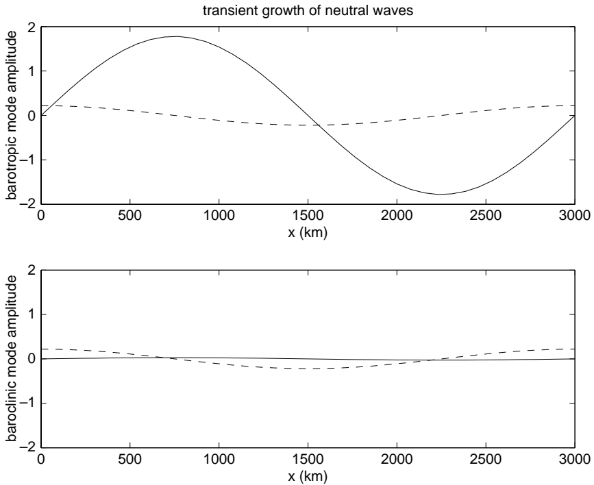
Fig. 8.11 Zonal distribution of the amplitude of a transient neutral disturbance initially confine entirely to the upper layer in the two-layer model. Dashed lines show the initial distribution of the baroclinic and barotropic modes; solid lines show the distribution at time of maximum amplification
