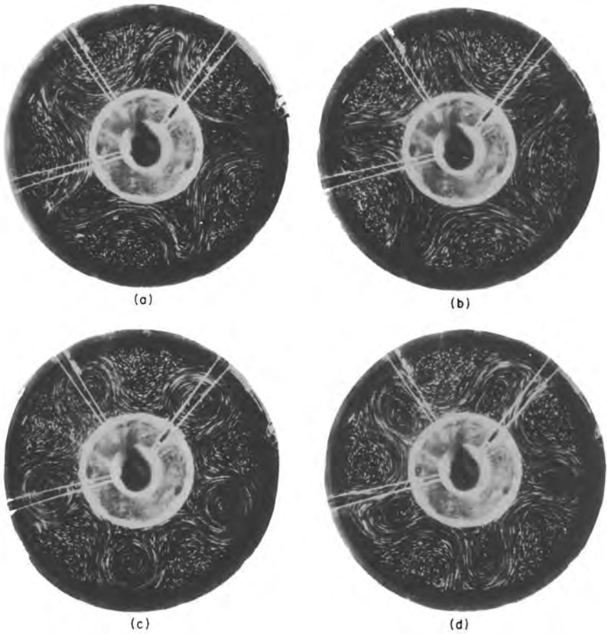
Fig. 10.20 Time exposures showing the motion of surface tracer particles in a rotating annulus. The four photographs illustrate various stages of a free-wave-tilted trough vacillation cycle. The period of the vacillation cycle is 16.25 revolutions, and the photographs are at intervals of four revolutions. (Photographs by Dave Fultz.)
