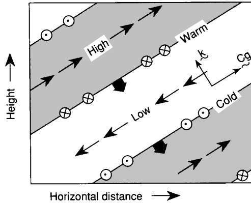
Fig. 7.12 Vertical section in a plane containing the wave vector \mathbf{k} showing the phase relationships among velocity, geopotential, and temperature fluctuation in an upward propagating inertia-gravity wave with m < 0 , v > 0 , and f > 0 (Northern Hemisphere). Thin sloping lines denote the surfaces of constant phase (perpendicular to the wave vector), and thick arrows show the direction of phase propagation. Thin arrows show the perturbation zonal and vertical velocity fields. Meridional wind perturbations are shown by arrows pointed into the page (northward) and out of the page (southward). Note that the perturbation wind vector turns clockwise (anticyclonically) with height. (After Andrews et al., 1987.)
