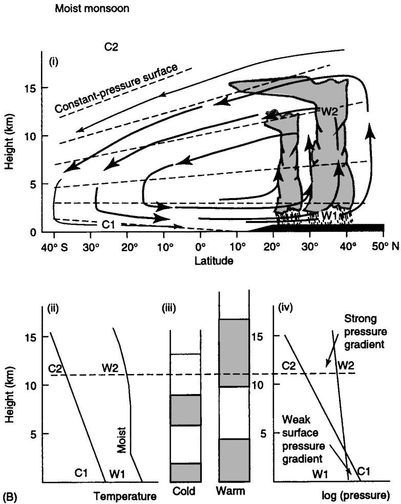
Fig. 11.9 Schematic representation of the moist phase of the Asian monsoon. (i) Arrows show the meridional circulation, dashed lines the isobars. (ii) Temperature profile for columns C1–C2 and W1–W2, respectively. (iii) Schematic of the mass distribution in the cold and warm sectors. (iv) Horizontal pressure difference as a function of height. (After Webster and Fasullo, 2003.)
