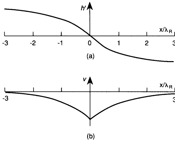
Fig. 7.13 The geostrophic equilibrium solution corresponding to adjustment from the initial state defined in (7.78). (a) Final surface elevation profiles (b) the geostrophic velocity profile in the final state. (After Gill, 1982.)
