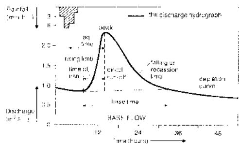
Storm hydrograph.
