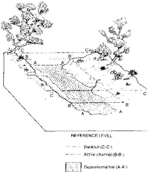
Channel capacity. Commonly used reference levels. Source: E.R. Hedman and W.R. Osterkamp 1981: Streamflow characteristics related to channel geometry of streams in western United States . US Geological Survey water supply paper 2193.
