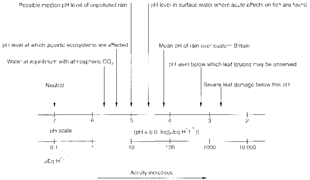
Scale of pH and \text{H}^+ concentration; acidity ( \text{H}^+ ) increases, while pH decreases on a 'log scale', i.e. 10:1. Source: G. Howells 1990: Acid rain and acid waters . Chichester: Ellis Horwood.
