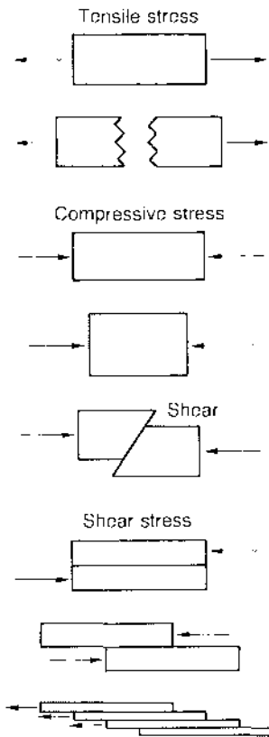
Stress. Schematic illustration of tensile, compressive and shear stresses.
