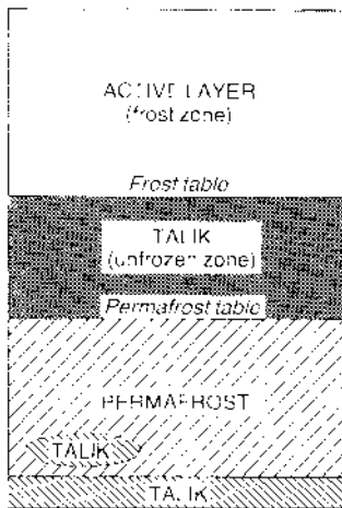
Permafrost: 1. Terminology of some features associated with permafrost.
