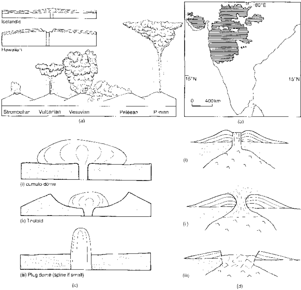
Volcano. Some major volcanic landforms: (a) types of eruption; (b) a lava plateau – the Deccan of India; (c) acid lava (viscous) extrusion forms; (d) the stages in the formation of a caldera by collapse: (i) initial volcano; (ii) explosion; (iii) collapse.
