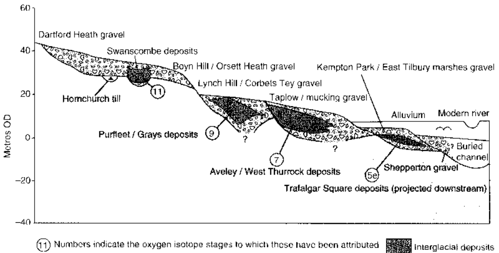
⑪ Numbers indicate the oxygen isotope stages to which these have been attributed Idealized transverse sequence through the terraces of the lower Thames, England. Source: Reproduced from D.R. Bridgland, P. Allen and B.A. Haggart eds 1995: The Quaternary of the lower reaches of the Thames: field guide . Durham: Quaternary Research Association.
