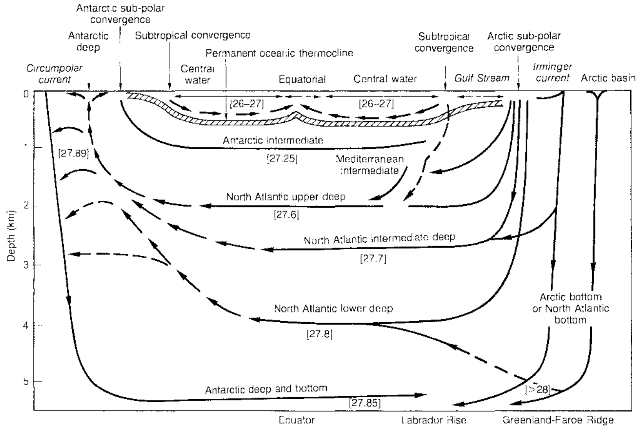
Water mass: 2. Schematic representation of the meridional circulation in the Atlantic Ocean. The numerical values in square brackets are mean density values ( \sigma_t ). Source: Tchernizic 1985.
