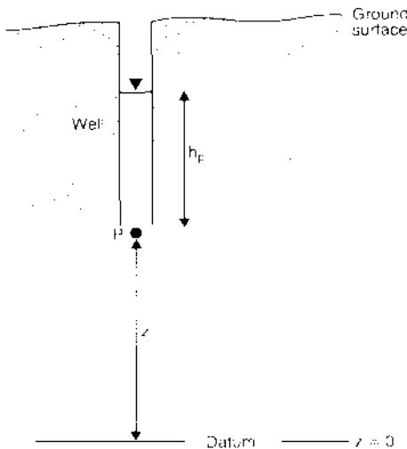
Figure 7. The Hydraulic Head h = hp + z where hp = Pressure head and z = Elevation head. \nabla signifies standing water level.
