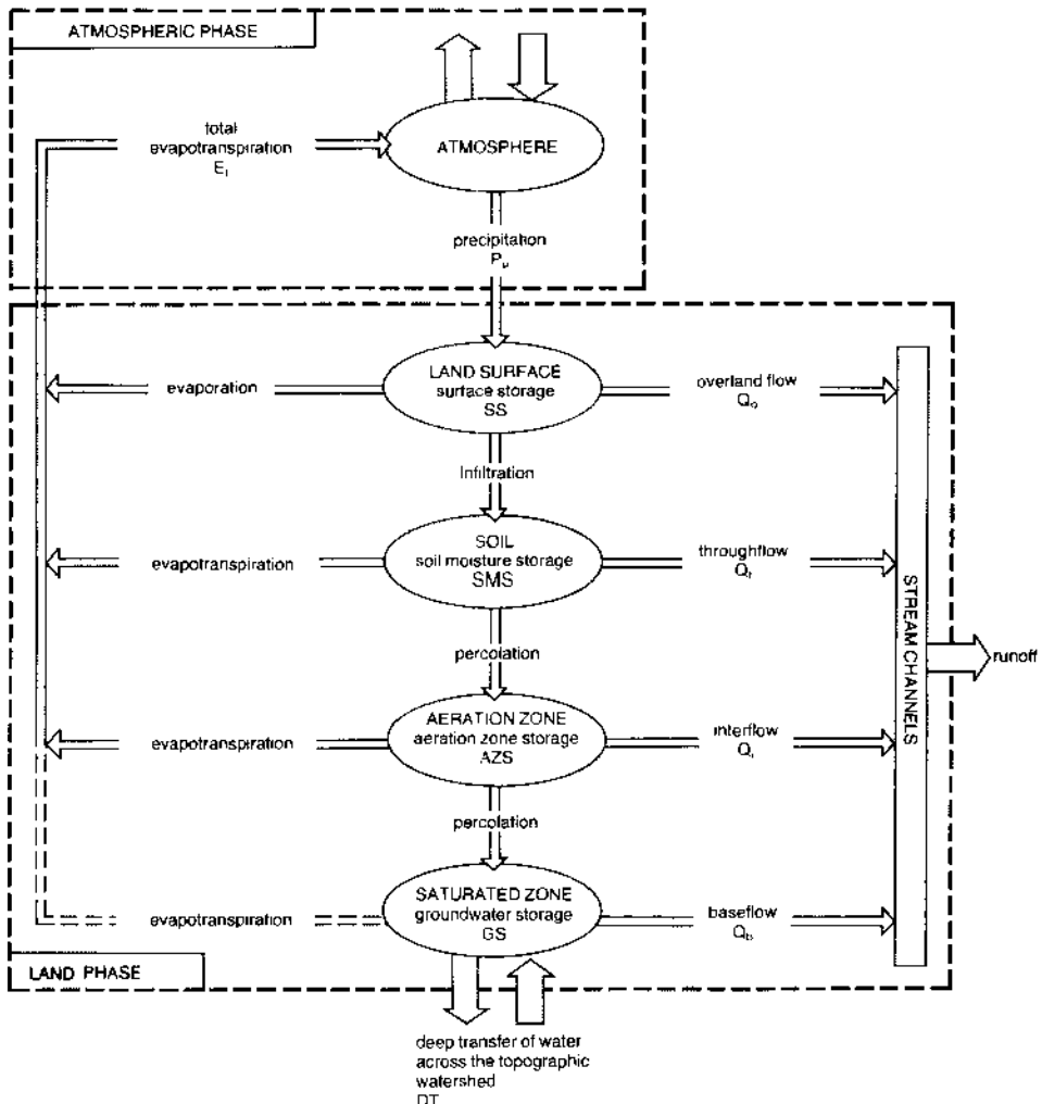
Hydrological cycle: 1. Drainage basin.
