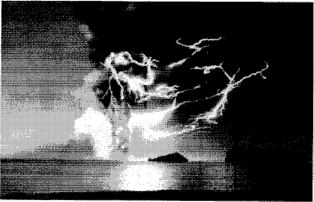
Lightning strikes the earth's surface an average 100,000 times each day. This spectacular example was photographed over the new volcanic island of Surtsey, Iceland.
