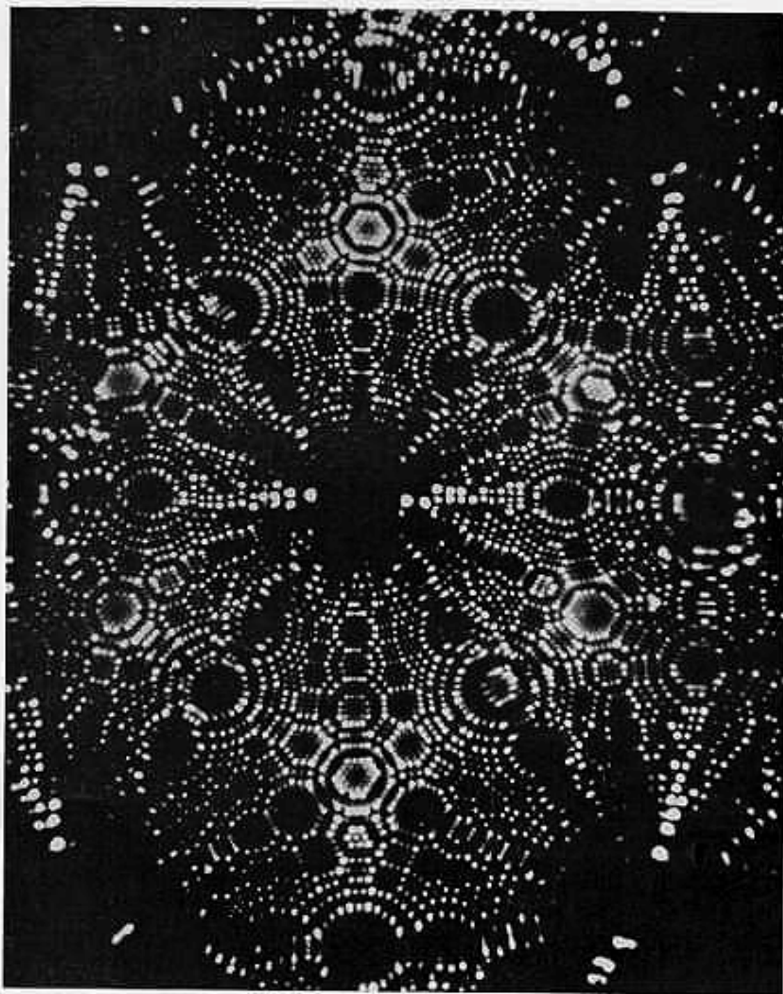
FIG. 71 Photomicrograph of a pure tungsten crystal magnified 2,700,000 times, which was made by the Conco-Muller Field Ion Microscope. The hexagonal form of water crystals is clearly shown in this picture.
