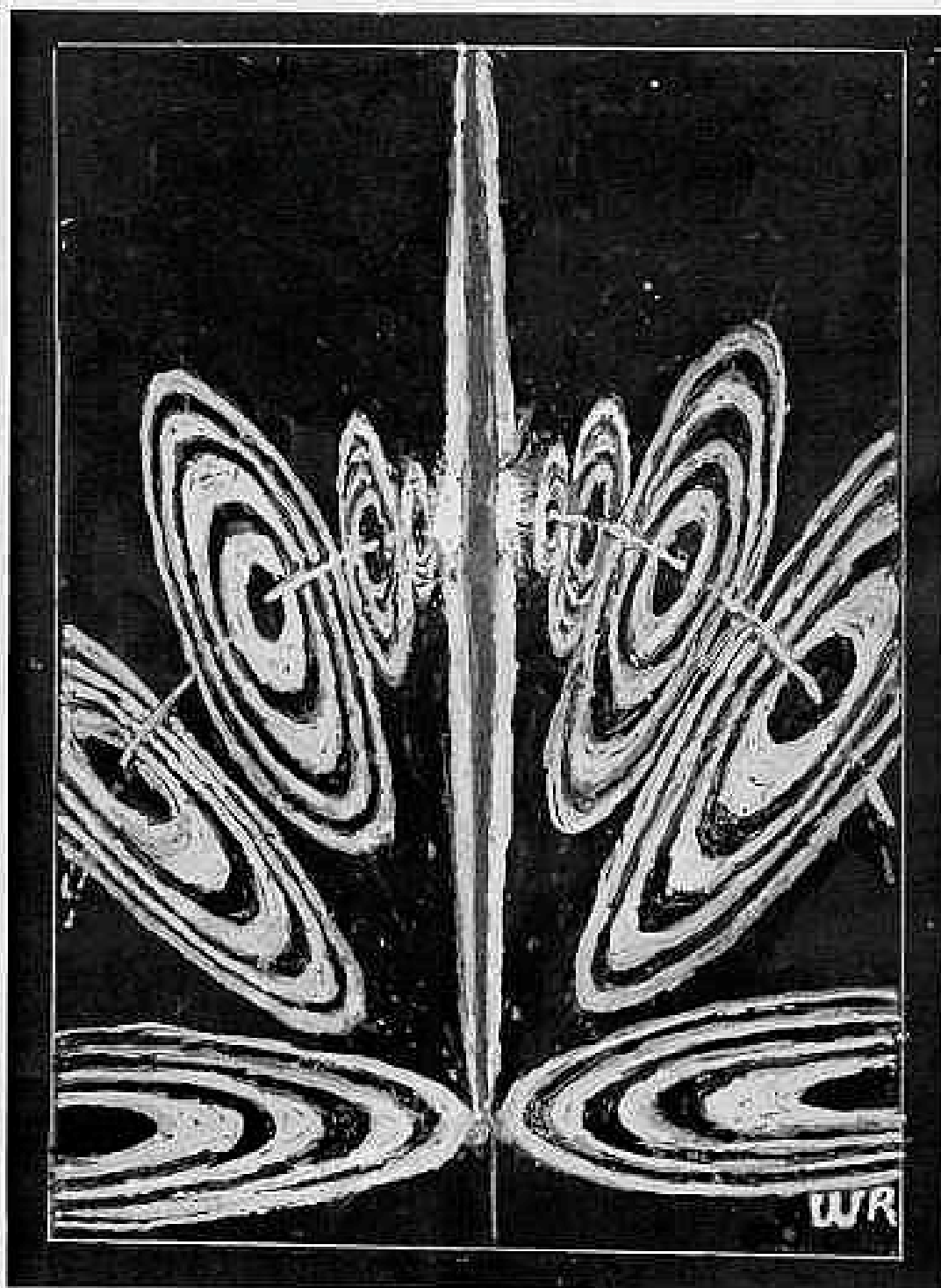
FIG. 54 Compression rings on the wave in octave formation, which is the basic cause of this curved universe of motion. In the center of this diagram are the expansion rings and spiral arms which radiate the heat which the gold has generated. (See our new Laws of Thermodynamics)
