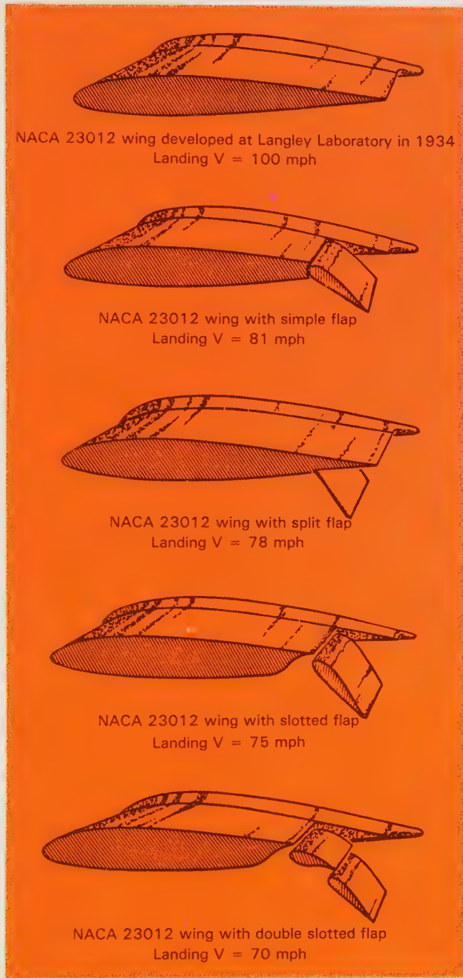
Steps taken to modify wings for increased lift during landing.
