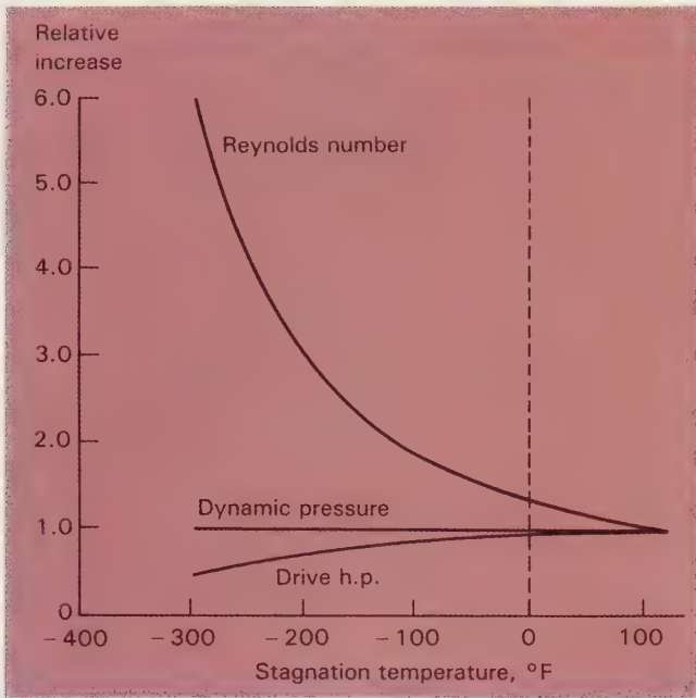
At very low temperatures, the Reynolds number rises dramatically as the viscosity of the test gas drops. The drive power also decreases.
