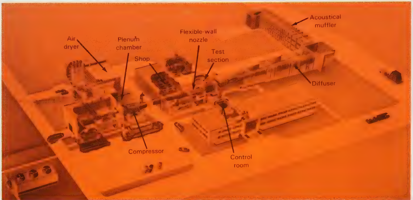
The first supersonic tunnel built at Lewis had an 8 × 6-foot supersonic test section. Doors downstream from the sound muffler permitted either open- or closed-circuit operation.
