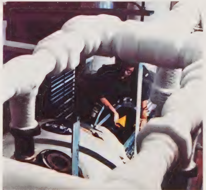
At very low temperatures, the Reynolds number rises dramatically as the viscosity of the test gas drops. The drive power also decreases.
