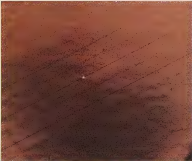
Schlieren photo of several Mach lines generated by strips of Scotch tape on one wall (air velocity = Mach 2).
