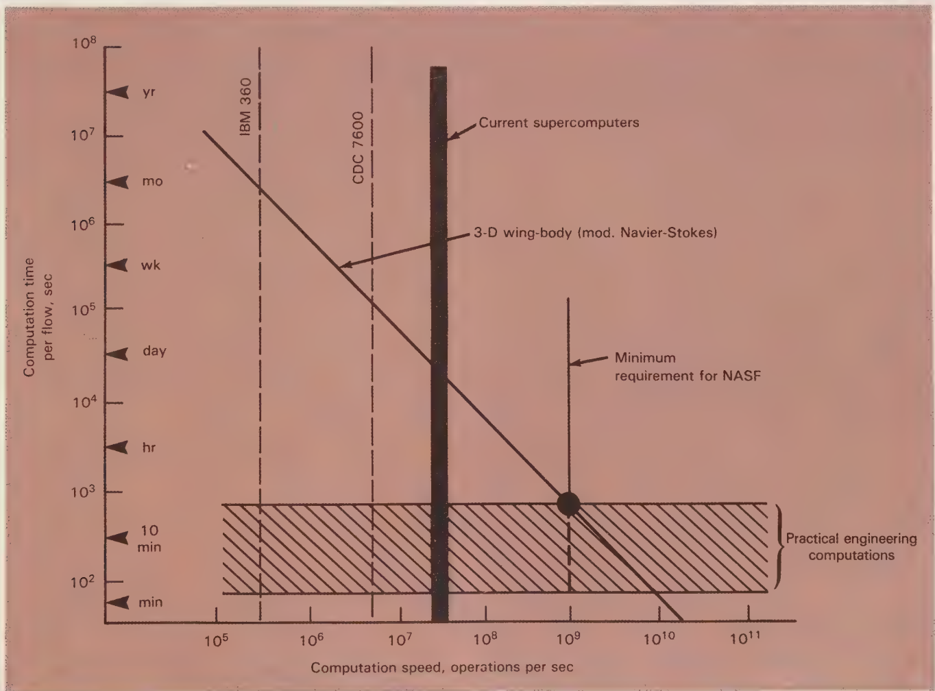
The computer time required to perform a specific aerodynamic computation is plotted against computation speed. Present supercomputers are fast approaching the speeds desired for practical operations at the proposed National Aerodynamics Simulation Facility. (Ames)
