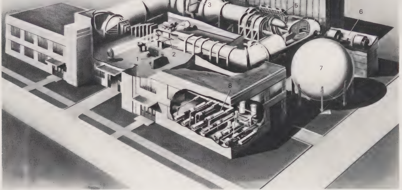
The Ames 6 × 6-foot supersonic wind tunnel with supporting facilities.
