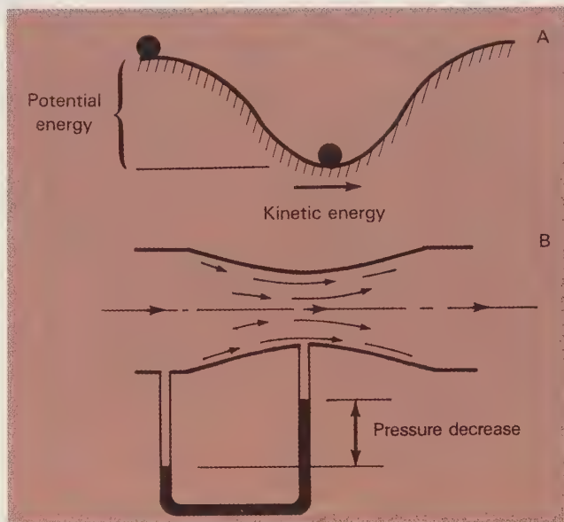
(A) As the ball rolls down the hill, the loss of potential energy is converted into kinetic energy, illustrating the law of conservation of energy. (B) Likewise in fluid flow, an increase of fluid velocity (kinetic energy) is balanced by a decrease in static pressure (potential energy). This is Bernoulli's principle.
