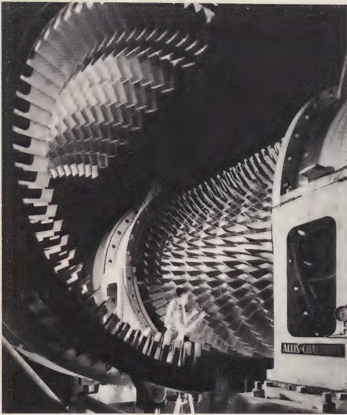
A multistage compressor for supersonic wind tunnel use, showing a section of the stator removed. Each ring of blades constitutes a stage.
