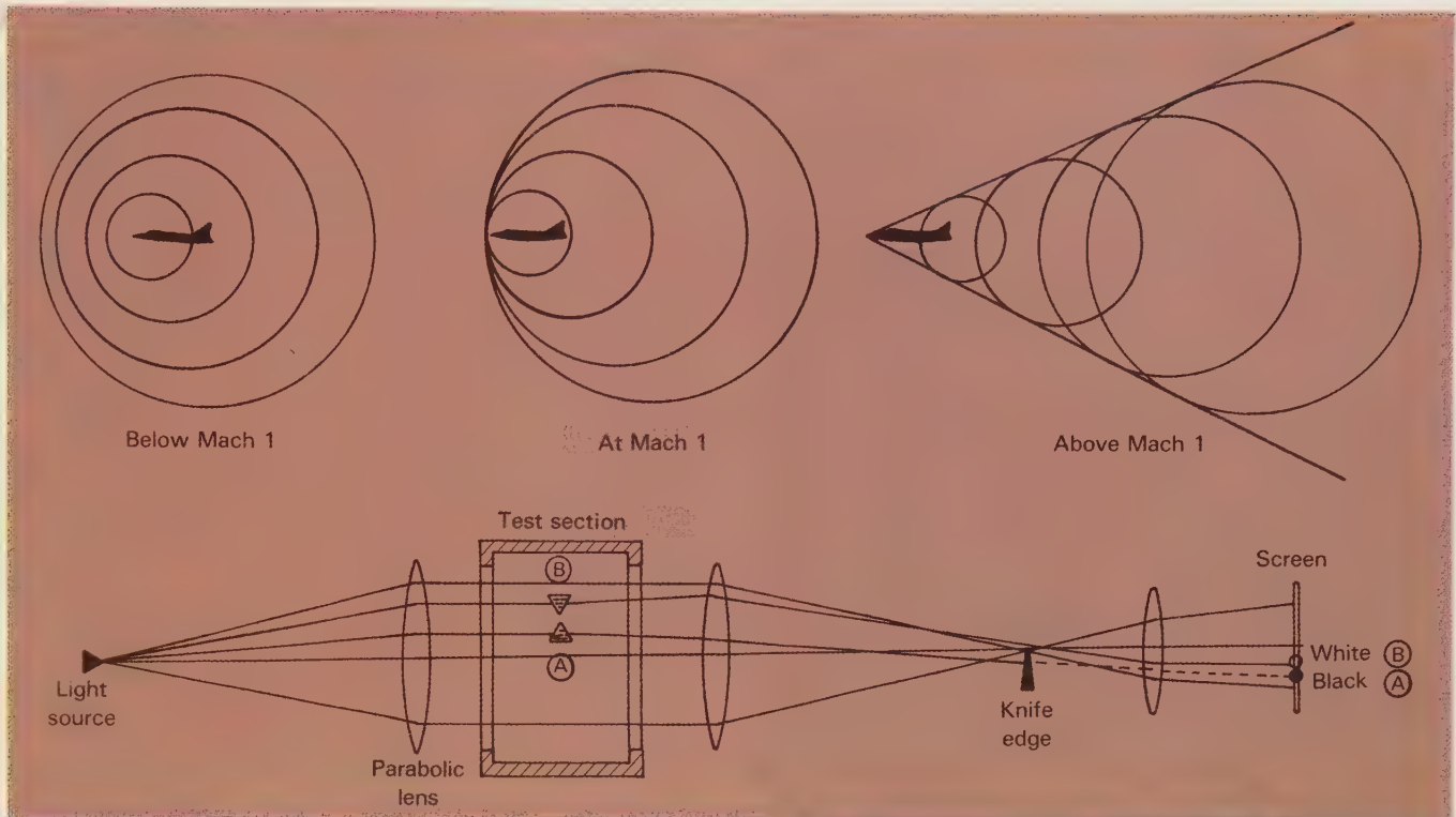
(Top) The origin of shock waves. (Bottom) Shock waves can be seen only rarely under natural conditions. In the controlled conditions existing in a wind tunnel, shock waves can be made sharply visible by means of a schlieren optical system. First, a small but intense source of light outside the test section illuminates the test section through a parabolic lens. A second lens collects the light rays on the other side of the test section and focuses them on a sharp edge (called a knife edge). Any air disturbances in the wind tunnel will deflect the light rays up or down, depending on the changes in air density. Triangles A and B show how high- and low-pressure disturbances, respectively, will bend the rays. Light rays bent downward will be intercepted by the knife edge and create a dark area on the screen; those bent upward form light areas. The net effect is that changes in air density produced by shock waves and other flow disturbances show up as dark and light areas on the screen. (Right) A schlieren photograph of shock waves around a model in a supersonic tunnel.
