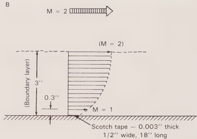
Tiny imperfections in the wall of a supersonic wind tunnel will generate Mach lines that can be seen in schlieren photos. (A) At Mach 2, the lines make 30 degree angles with the tunnel axis. (B) Scotch tape 0.003 inch thick will create Mach lines even though the tape is well within the subsonic boundary layer of air.
