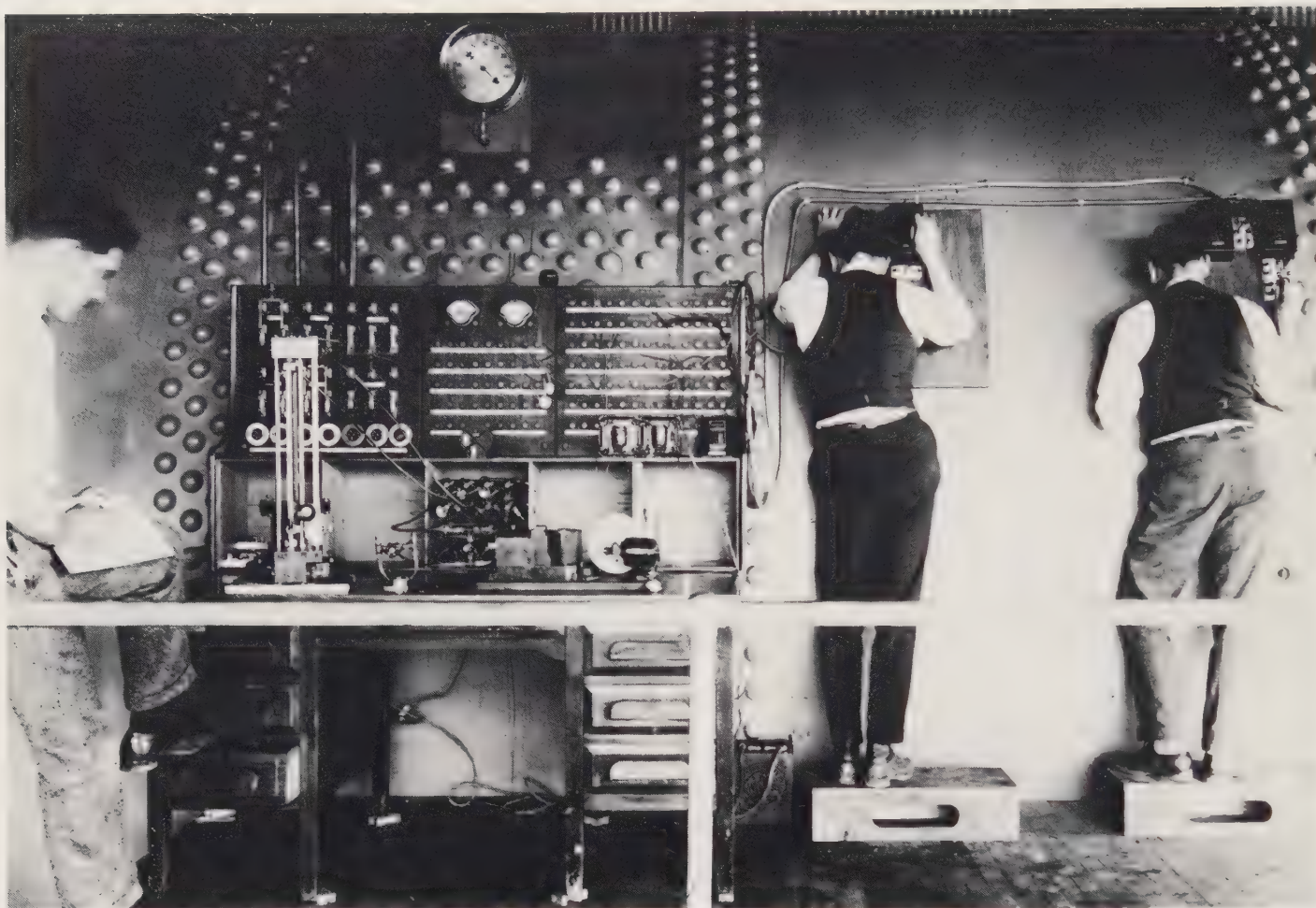
Two engineers reading balances located inside the Langley variable density wind tunnel in 1923.
