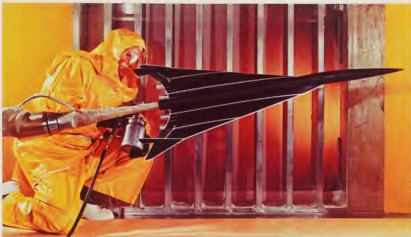
Preparation of an SST model in the Langley unitary tunnel.
