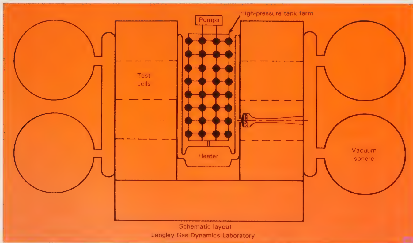
Arrangement of the Langley Gas Dynamics Laboratory. High-pressure air was released through the various test cells, as required, into the vacuum spheres.
