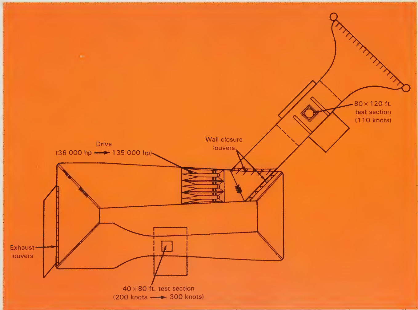
Circuit diagram of the Ames 40 × 80-foot modified tunnel with the 80 × 120-foot test section grafted on.
