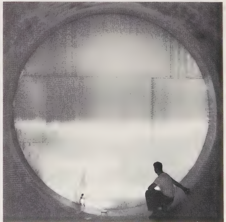
Fine-mesh antiturbulence screens inside the settling chamber of the 12-foot pressure tunnel at Ames.
