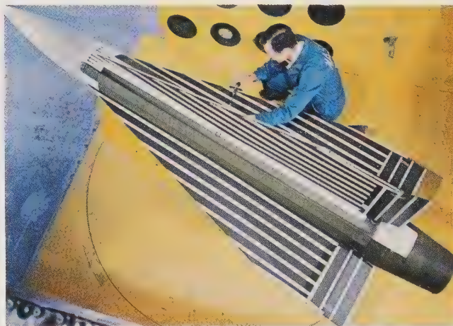
Model of a delta-winged craft in the thermal structures tunnel.
