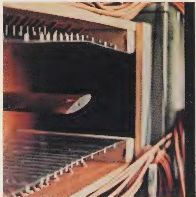
An airfoil in a small wind tunnel with adaptive walls that conform automatically to the streamlines established by the airfoil under test.
