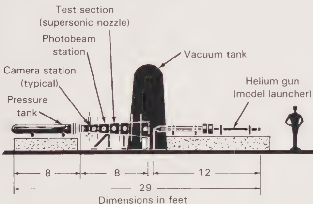
The small-scale atmospheric entry simulator located at Ames Research Center.
