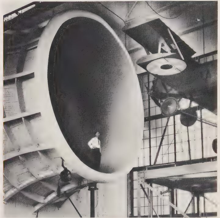
The Sperry M-1 Messenger was the first full-scale airplane tested in the propeller research tunnel in mid-1927. Note the removal of the outer wing panels which would have extended beyond the 20-foot throat diameter.
