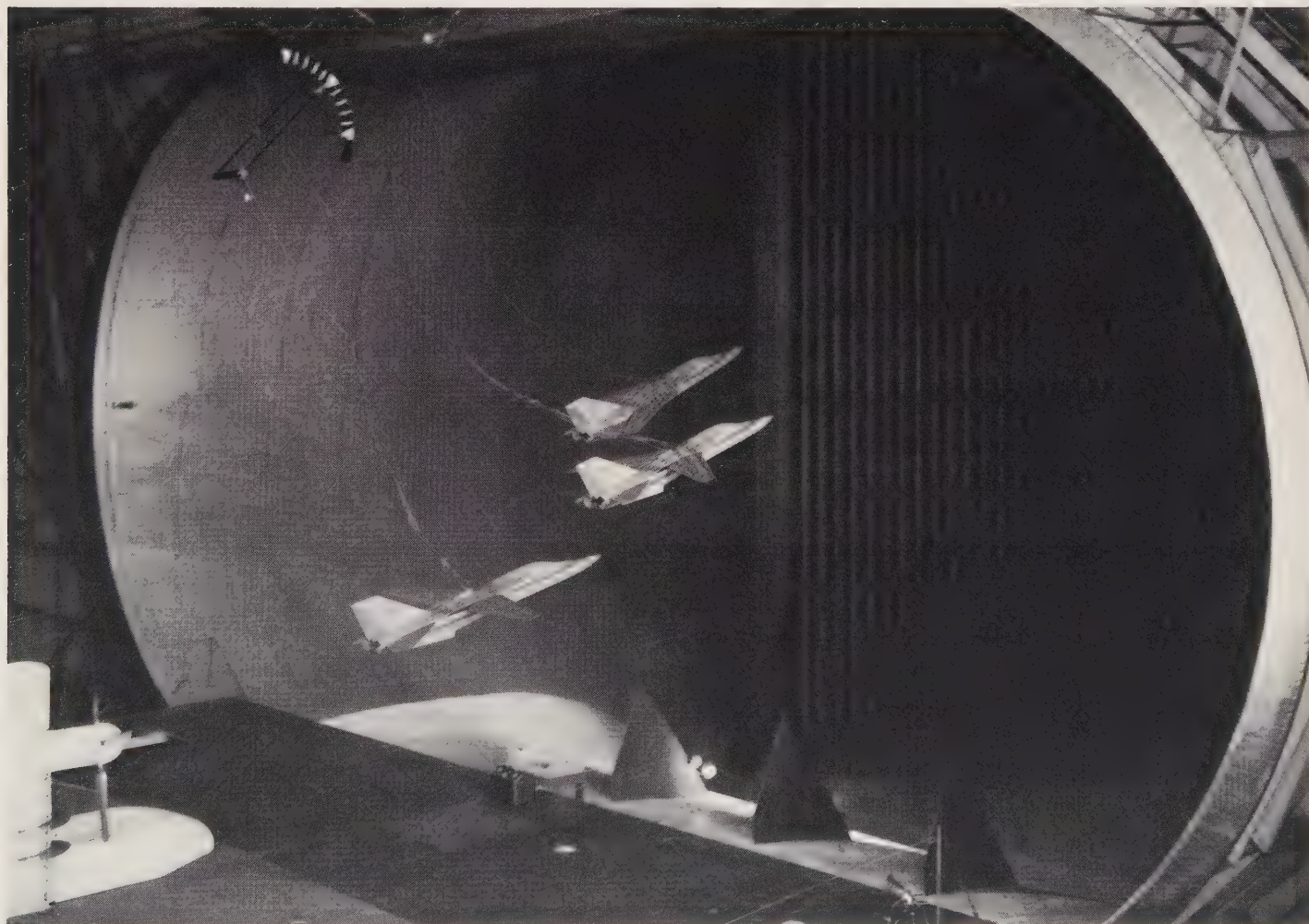
A powered model of the F-111 fighter-bomber sweeps its wings during free-flying tests in the Langley full-scale wind tunnel.
