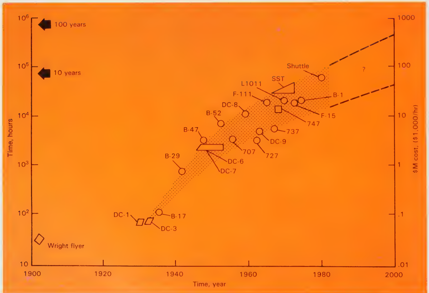
The number of wind tunnel tests required for new aircraft has risen by several orders of magnitude during the past half century.
