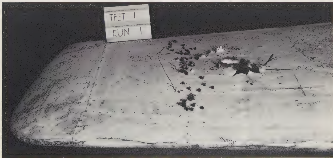
A bullet-riddled wing section undergoing aerodynamic tests in the 8-foot high-speed tunnel.
