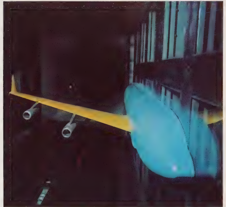
Half an aircraft mounted in the Langley 8-foot transonic pressure tunnel to measure the wing bending moments generated by a winglet.
