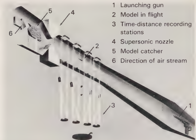
(Top left) Loading the gun in the Ames supersonic free-flight tunnel. (Top right) Schematic drawing of the Ames supersonic free-flight tunnel. (Bottom left) Shadowgraph of sabot separation. (Bottom right) Diagram of sabot operation.
