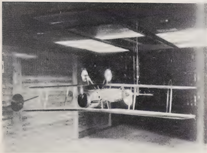
National Physical Laboratory duplex wind tunnel with a biplane model in place for lift and drag measurements. (It was easier to measure lift forces when the plane was upside down.) (Photo, National Physics Laboratory)
