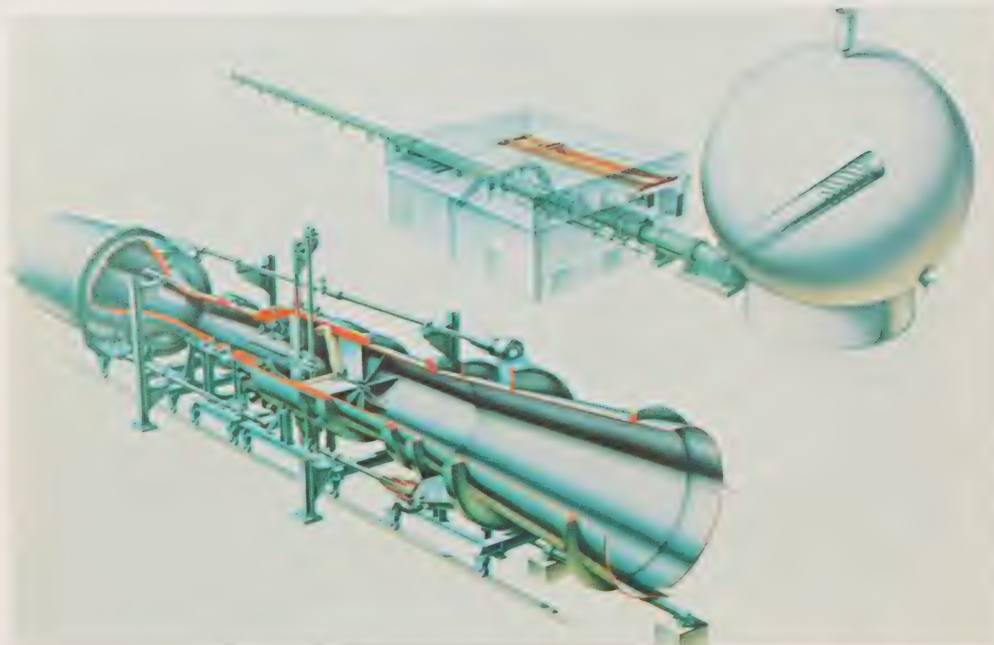
Phantom drawing of the Ludwig tube wind tunnel built at Marshall Space Flight Center for aerodynamic research on launch vehicles.
