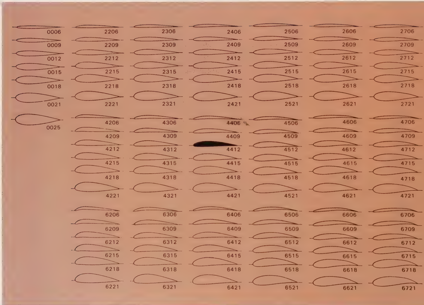
Cross sections of the early series of NACA airfoils (from TR 460).
