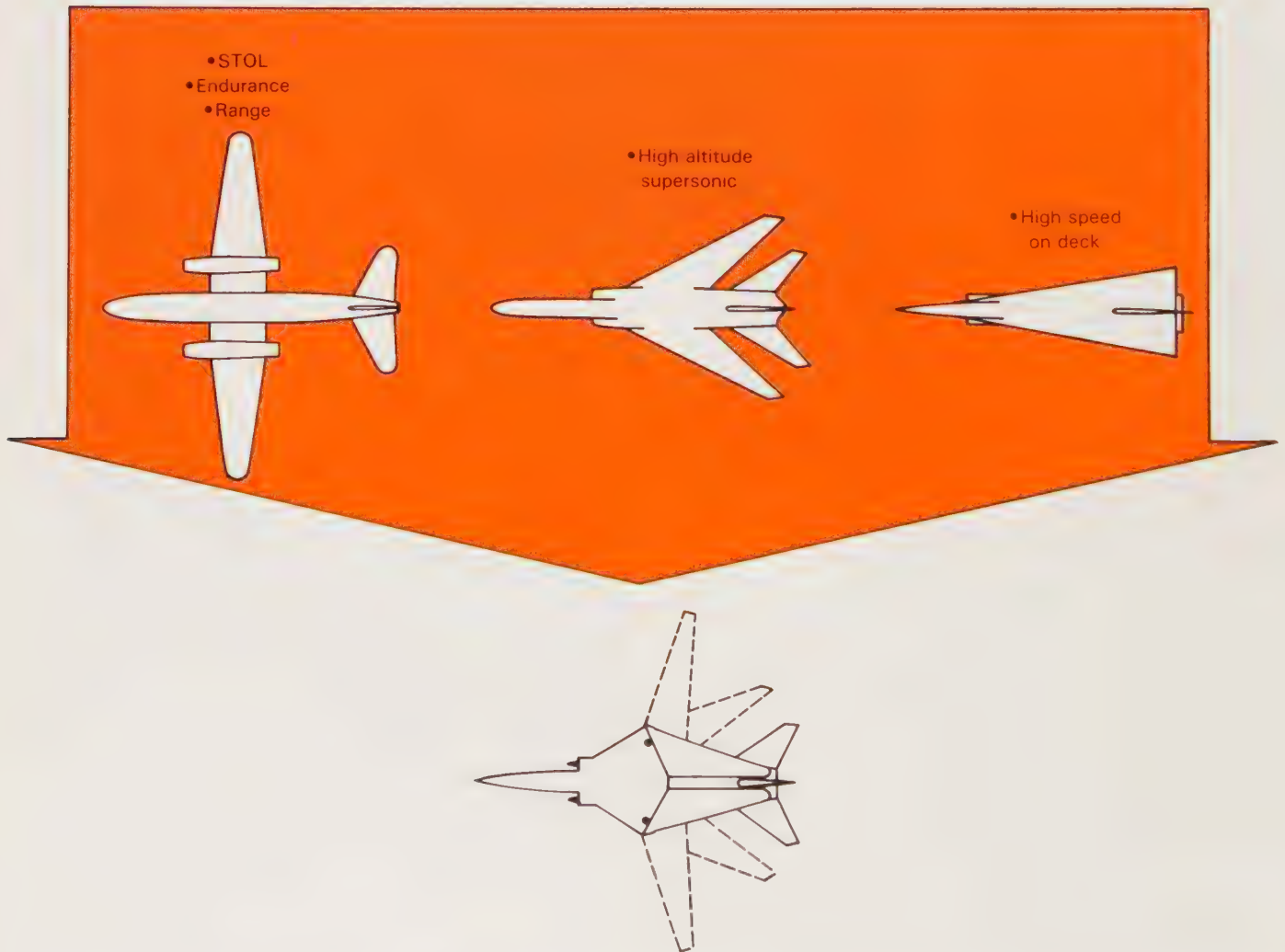
Wing configurations desirable for different missions. An aircraft with variable-sweep wings can operate effectively in all three regimes.
