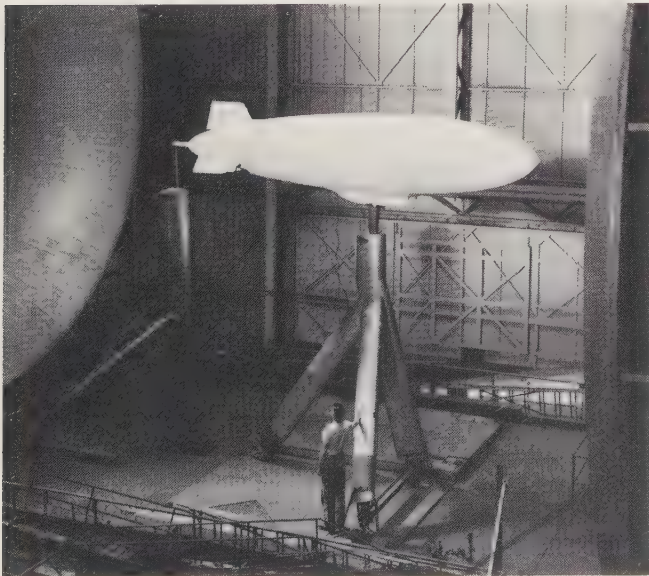
A scale model of an airship under test in the full-scale tunnel.
