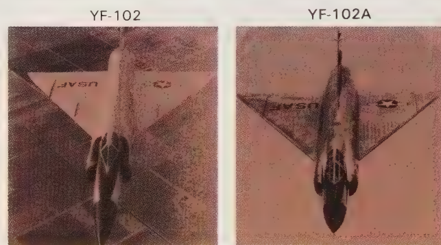
The YF-102 and YF-102A side by side. The narrowing of the YF-102A fuselage near the wings was dictated by the Area Rule and enabled the craft to become supersonic. Without the Area Rule, the YF-102 prototype never attained supersonic speeds in level flight.
