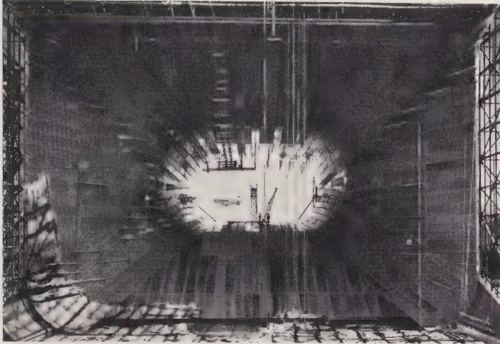
The cavernous entrance cone and test section of the Ames 40 x 80-foot full-scale wind tunnel.
