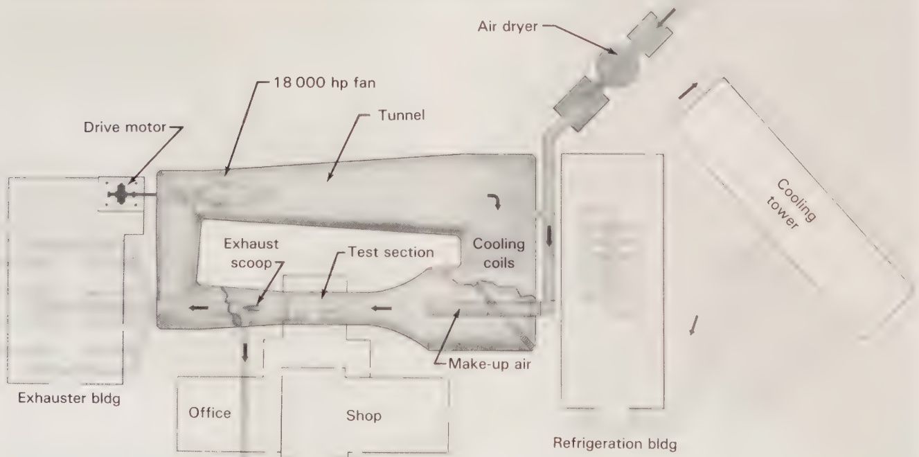
Layout of the Lewis altitude wind tunnel, showing equipment necessary to purge combustion products, control air pressure, and reduce air temperatures.
