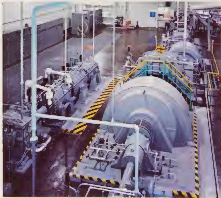
A linear array of five compressors feeding the Langley continuous-flow hypersonic tunnel. This facility achieved a Mach 10 flow through a test section 31 inches square on a continuous basis.
