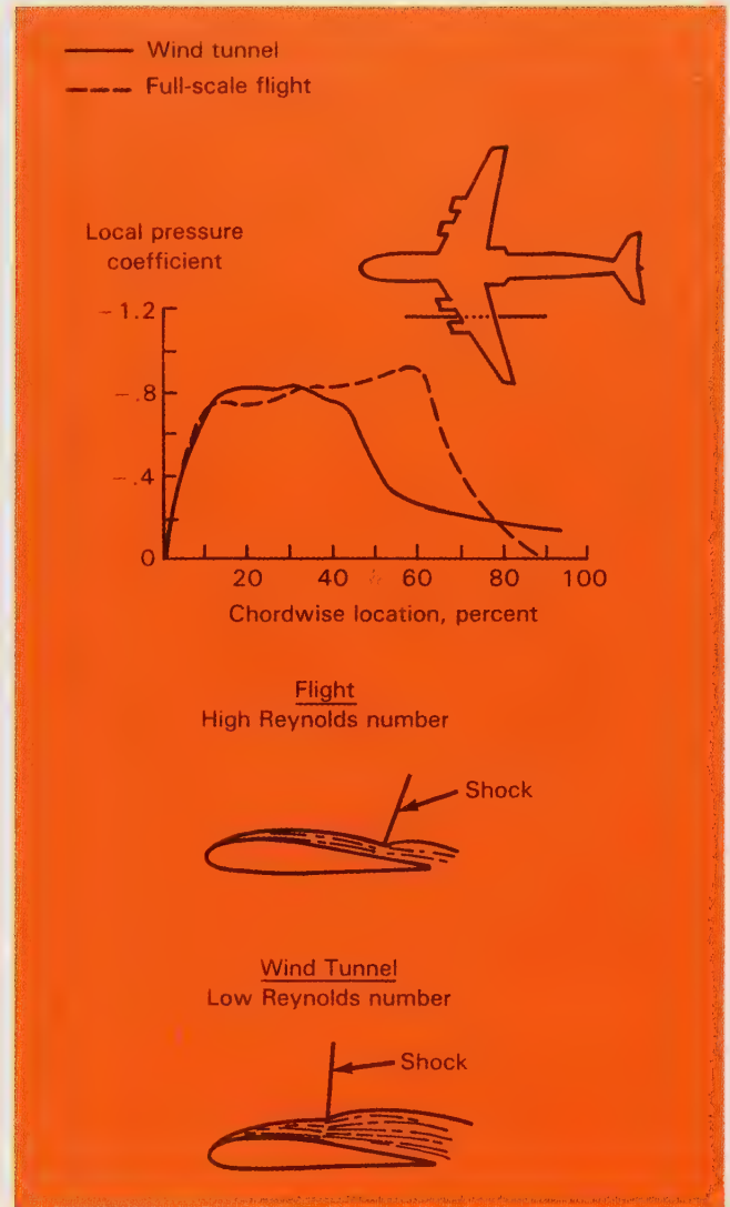
Wind tunnel measurements of shock-wave-induced flow separation are pessimistic when compared with actual flight data. The discrepancy is due to the inability of most wind tunnels to simulate high Reynolds numbers.
