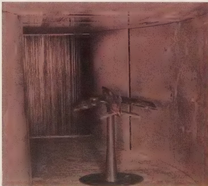
A model aircraft encounters a turning airstream inside the Langley stability tunnel.
