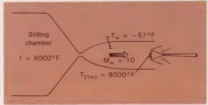
Profile of a hypersonic wind tunnel illustrating how the temperature is roughly the same within the stilling chamber and where the flow has stagnated in front of the model.
