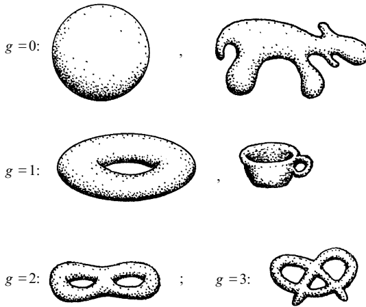
Fig. 8.9 The genus of a Riemann surface is its number of ‘handles’. The genus of the sphere is 0, that of the torus, or teacup surface is 1. The surface of a normal pretzel has genus 3.
