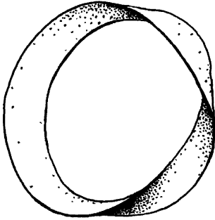
Fig. 12.15 The Möbius strip: an example of a non-orientable space.
