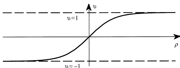
Fig. 18.12 The graph of velocity v (with c = 1 ) in terms of rapidity \rho defined by \rho = \frac{1}{2} \log \{(1+v)/(1-v)\} , i.e. v = (e^\rho - e^{-\rho}) / (e^\rho + e^{-\rho}) = \tanh \rho .
