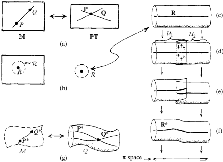
Fig. 33.26 Construction of a left-handed non-linear graviton. (a) In the standard flat-space twistor correspondence, points P and Q of \mathbb{CM}^1 are null separated whenever the corresponding lines \mathbf{P} and \mathbf{Q} in \mathbb{P}^3\mathbb{T} meet. (b) We wish to deform \mathbb{P}^3\mathbb{T} , somehow, to a curved twistor space, but mathematical theorems tell us that this cannot be done globally. Accordingly, we take only a suitable (open) neighbourhood \mathcal{R} , of a point R in \mathbb{CM}^1 as our starting ‘spacetime’. (c) This corresponds to a tubular neighbourhood \mathcal{Q} , in \mathbb{P}^3\mathbb{T} , of the line \mathbf{R} . (d) We can now apply the procedure of Fig. 33.25 to deform \mathcal{Q} (considered as the union of two open sets \mathcal{U}_1 and \mathcal{U}_2 ). (e) However, we find that the original line \mathbf{R} is now broken, and cannot be used as a sensible definition of a ‘spacetime point’. (f) A theorem of Kodaira comes to our rescue, to tell us that there is a 4-parameter family of ‘lines’ \mathbf{R}^* (compact holomorphic curves, belonging to the same topological class as our original lines), which will serve this purpose. (g) The points of our sought-for ‘non-linear graviton’ space \mathcal{M} (a complex 4-space) are given by Kodaira’s curves \mathbf{R}^* . The (complex conformal) metric of \mathcal{M} is defined (as in (a)) by the condition that P^* and Q^* are null separated whenever the corresponding lines \mathbf{P}^* and \mathbf{Q}^* meet. The Weyl curvature of \mathcal{M} turns out to be automatically anti-self-dual, and it is also Ricci-flat by virtue of the details of the construction.
