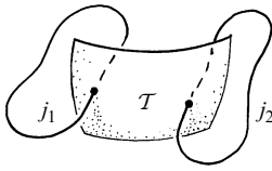
Fig. 32.4 A 2-dimensional test surface \mathcal{T} in the 3-surface \mathcal{S} . Each intersection of \mathcal{T} with a loop contributes the value 8\pi G\eta\hbar\sqrt{j(j+1)} of area ( j being the loop's 'spin' value).
