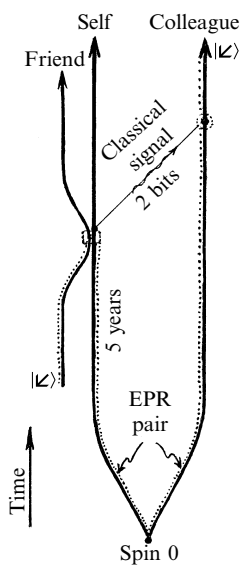
Fig. 23.7 ‘Quantum teleportation’, demonstrating the acausal propagation of quanglement. A space-time diagram illustrates the process whereby the unknown quantum state ( |L\rangle ) of spin \frac{1}{2} , given to me by my friend, can be conveyed to my colleague on Titan by the mere transmission of 2 bits of classical information, provided that my colleague and I already share an EPR pair. The acausal quanglement link is depicted as a dotted path.
