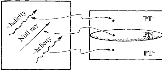
Fig. 33.6 The real 5-manifold \mathbb{P}\mathbb{N} divides projective twistor space \mathbb{P}\mathbb{T} into two complex-3-manifold pieces \mathbb{P}\mathbb{T}^+ and \mathbb{P}\mathbb{T}^- , these representing massless particles of positive and of negative helicity, respectively.
