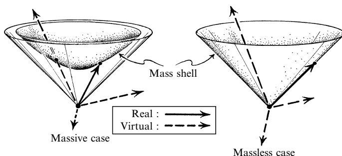
Fig. 26.6 The mass shell in momentum space. (Compare Figs. 18.7, 18.17.) For real (free) particles of rest-mass M , the 4-momentum p^a lies on the mass shell (so p^a p^a is future timelike or future null with p_a p^a = M^2 ), but virtual particles, in the interior of a Feynman graph, can be ‘off shell’.
