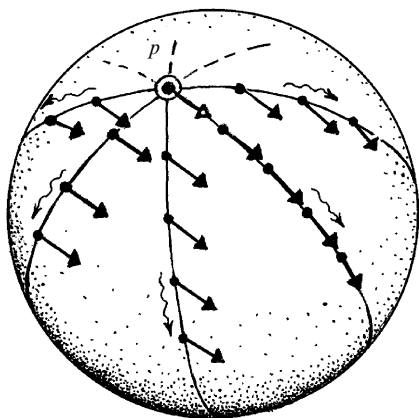
Fig. 14.3 Parallel transport of v along five different paths (all great circles).
