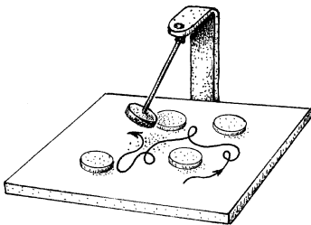
Fig. 27.1 Chaotic motion. An ‘executive toy’ consisting of a magnetic pendulum swinging just above a collection of fixed magnets. The actual path taken by the pendulum depends extremely sensitively on its initial position and velocity.
