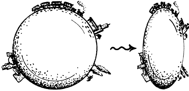
Fig. 18.14 FitzGerald–Lorentz ‘flattening effect’. A spherical planet moves to the right at a speed v (close to that of light) with respect to a fixed reference system. In that system it would be described as being flattened by a factor (1 - v^2/c^2)^{1/2} in its direction of motion.
