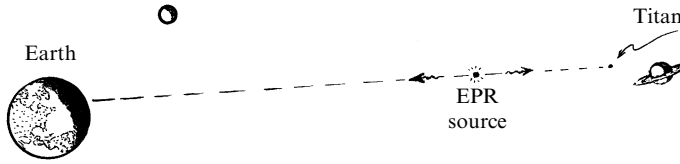
Fig. 23.4 The author, situated on the Earth, imagines himself to be the receiver of one component of a succession of EPR particle pairs, the other being a colleague on Titan, where the source of the pairs is roughly equidistant between the two receivers. Even for particles travelling at the speed of light, there would be about 45 minutes to decide on the detector orientations.
