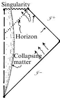
Fig. 30.4 Hawking's calculation of a black hole's temperature, involving the collapse of some matter to a black hole in the distant past, requires only the (standard) notion of positive/negative frequency splitting on \mathcal{S}^+ and on \mathcal{S}^- . The black hole's vacuum becomes a thermal state (a density matrix) because the initial information on \mathcal{S}^+ gets divided between that at \mathcal{S}^+ and that at the final singularity, the latter becoming lost.
