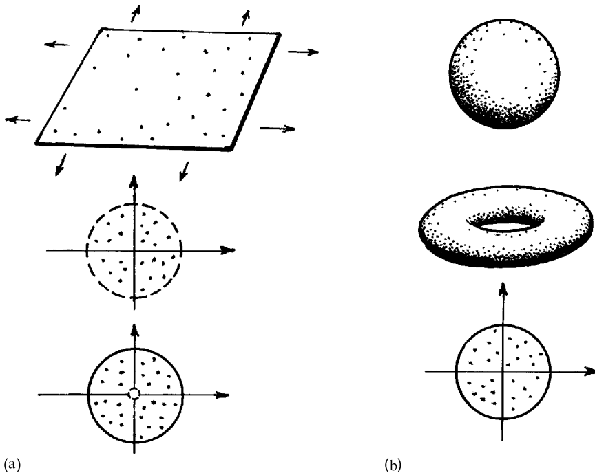
Fig. 12.13 (a) Some non-compact spaces: the infinite Euclidean plane, the open unit disc, and the closed disc with the centre removed. (b) Some compact spaces: the sphere, the torus, and the closed unit disc. (Solid boundary lines are part of the set; broken boundary lines are not.)
