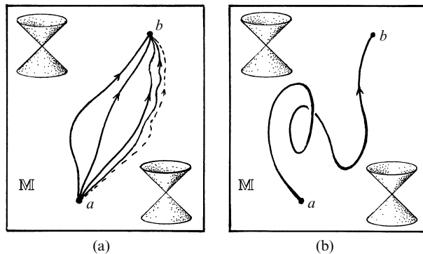
Fig. 26.3 (a) For a single structureless particle, a classical history is a curve in spacetime (here Minkowski space \mathbb{M} ), taken between fixed events a, b . (b) The curve need not be a classically allowable smooth world-line, with tangent always future-timelike; it can even wander backwards and forwards in time.
