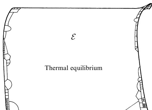
Fig. 27.4 The particular box \mathcal{E} , representing thermal equilibrium, has a volume E , that is normally practically equal to the volume \mathcal{P} of the entire phase space \mathcal{P} , and therefore far exceeds the volumes of all the other boxes together.
