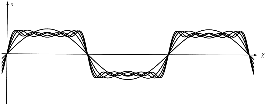
Fig. 9.12 Partial sums of the Fourier series s(\chi) = \sin \chi + \frac{1}{3} \sin 3\chi + \frac{1}{5} \sin 5\chi + \frac{1}{7} \sin 7\chi + \frac{1}{9} \sin 9\chi + \dots converging to a square wave (like that of Fig. 9.11a).
