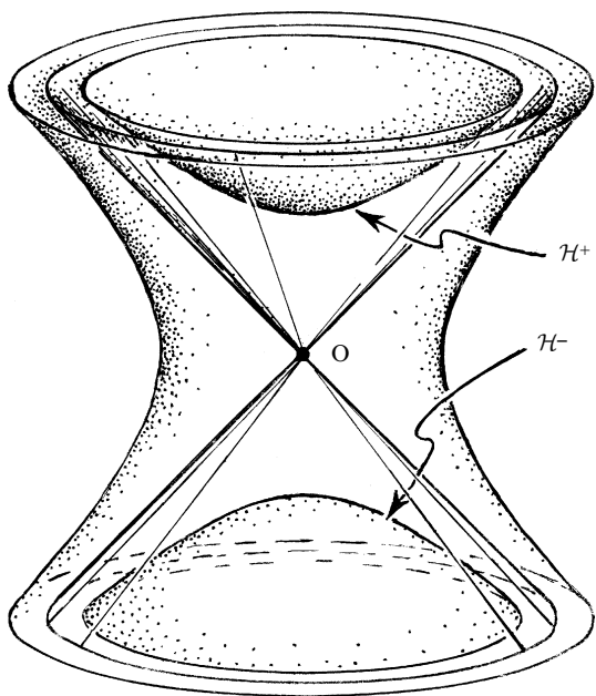
Fig. 18.7 ‘Spheres’ in \mathbb{M} , as the loci of points a fixed Minkowski distance a from a fixed point O . If a > 0 (with the +--- ds^2 signature) we get two ‘hyperbolic’ pieces, the ‘bowl-shaped’ \mathcal{H}^+ (within the future light cone) and the ‘hill-shaped’ \mathcal{H}^- , (within the past light cone). For imaginary a (or with real a and the +++ d\ell^2 signature) we get a one-sheeted hyperboloid, spacelike-separated from O .
