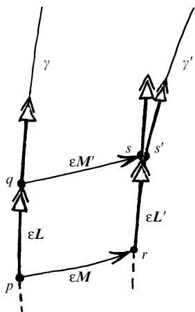
Fig. 14.11 Geodesic deviation: choose N = L in the parallelogram of Fig. 14.10. The sides pq and rs' are segments of two neighbouring geodesics \gamma and \gamma' ( \gamma being \lambda and \gamma' being \lambda' ) starting from p and r , respectively, with parallel-propagated tangent vectors L and L' , the connecting vector at p being M . The geodesic deviation between \gamma and \gamma' is measured by the difference between the results of parallel displacement of L along the routes prs' and pqs , which is basically \varepsilon^2 L^a M^b L^c R_{abc}{}^d .
