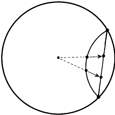
Fig. 2.15 To get from the conformal to the projective representation, expand out from the centre by a factor 2R^2/(R^2 + r_c^2) , where R is the radius of the bounding circle and r_c is the Euclidean distance out of the point in the conformal representation.
