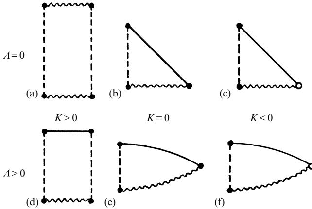
Fig. 27.17 Strict conformal diagrams for the respective Friedmann models of Fig. 27.13: (a) K > 0, \Lambda = 0 ; (b) K = 0, \Lambda = 0 ; (c) K < 0, \Lambda = 0 ; (d) K > 0, \Lambda > 0 (and \Lambda large enough); (e) K = 0, \Lambda > 0 ; (f) K < 0, \Lambda > 0 .
