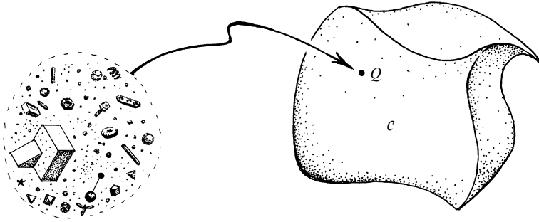
Fig. 20.1 Configuration space. Each point Q of the N -dimensional manifold C represents an entire possible configuration of (say) a family of Newtonian point particles and rigid bodies. As the system evolves in time, Q describes some curve in C .
