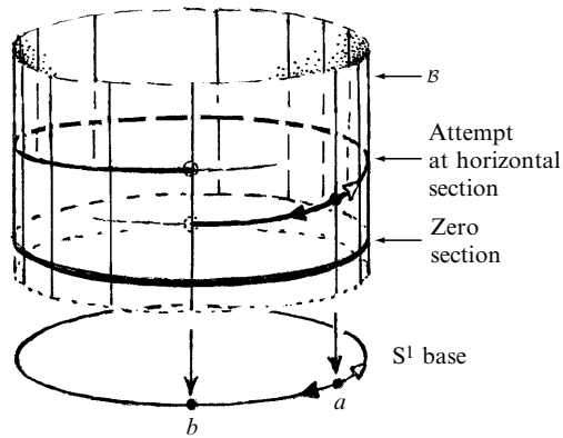
Fig. 15.16 A ‘strained’ line bundle \mathcal{B} over \mathcal{M}=\mathbb{S}^1 , using a different symmetry of the fibre \mathcal{V} from that of Figs. 15.4, 15.5, and 15.7 (where \mathcal{V} is still a 1-dimensional real vector space \mathbf{V}^1 ), namely a stretch by a positive factor (here 2). The topology is just that of the cylinder \mathbb{S}^1 \times \mathbb{R} , but there is a ‘strain’ that can be recognized in terms of a connection on \mathcal{B} . This connection defines a local notion of ‘horizontal’, for curves in \mathcal{B} . But consider two paths from a to b in the base, the direct path (black arrow) and the indirect one (white arrow). When we arrive at b we find a discrepancy (by a factor of 2), indicating that the notion of ‘horizontal’ here is path dependent.
