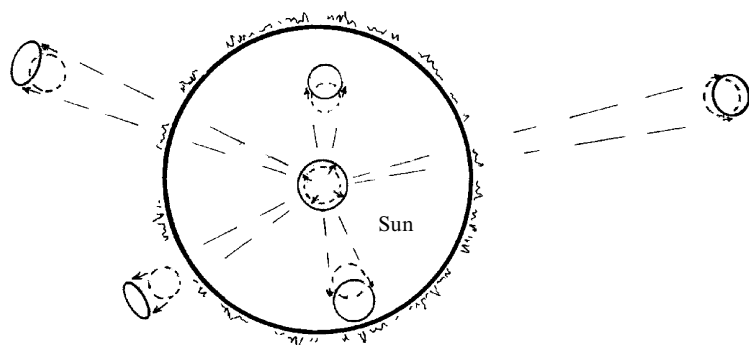
Fig. 28.16 We get a good impression of (lowest-order) effects of the two different kinds of spacetime curvature by ‘looking’ at the star field through a transparent non-refracting Sun (as though with massless neutrinos). To a reasonable approximation, rays passing through the Sun are focused just by Ricci curvature, resulting in magnification (as by a positive lens), whereas outside the Sun’s rim, we get essentially purely astigmatic Weyl distortions, so a small circular pattern in the star field would appear elliptical.
