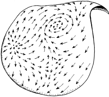
Fig. 10.5 The geometrical interpretation of a vector field \xi as a ‘field of arrows’ drawn on \mathcal{S} .
