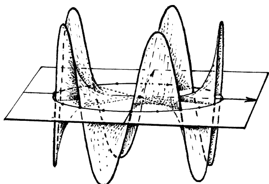
Fig. 9.4 On the unit circle, the real and imaginary parts of the function z^n appear as n th harmonic cos and sin waves (the real and imaginary parts of e^{in\lambda} , respectively, where z = e^{i\lambda} ). Here, for n = 5 , the real part of z^5 is plotted.
