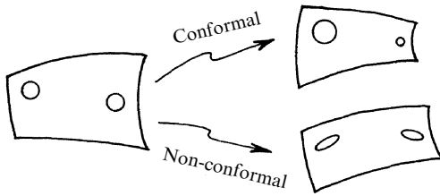
Fig. 8.4 For a conformal map, little (infinitesimal) circles can be expanded or contracted, but not distorted into little ellipses.
