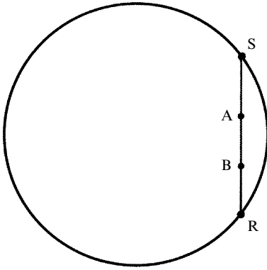
Fig. 2.14 In the projective representation, the formula for hyperbolic distance is now \frac{1}{2} \log \{RA.SB/RB.SA\} , where R and S are the intersections of the Euclidean (i.e. hyperbolic) straight line AB with the bounding circle.
