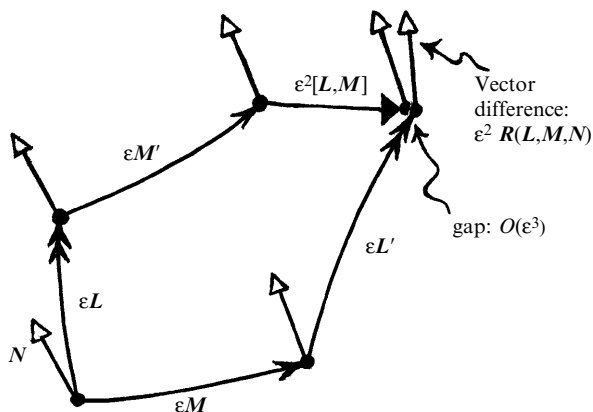
Fig. 14.19 Curvature, in the ‘mathematician’s notation’ (\nabla_L M - \nabla_M L - \nabla_{[L, M]})N = R(L, M, N) , from the O(\epsilon^2) discrepancy in parallel transport of a vector N around the (incomplete) ‘quadrilateral’ with sides \epsilon L, \epsilon M, \epsilon L', \epsilon M' . The Lie bracket contribution \epsilon^2[L, M] fills an O(\epsilon^2) gap, to order O(\epsilon^3) . (The index form of the vector R(L, M, N) is L^a M^b N^c R_{abc}{}^d .)
