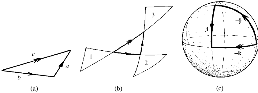
Fig. 11.4 (a) Translations in the Euclidean plane represented by oriented line segments. The double-arrowed segment represents the composition of the other two, by the triangle law. (b) For rotations in Euclidean 3-space, the segments are now great-circle arcs drawn on the unit sphere, each representing a rotation through twice the angle measured by the arc (about an axis perpendicular to its plane). To see why this works, reflect the triangle made by the arcs, in each vertex in turn. The first rotation takes triangle 1 into triangle 2, the second takes triangle 2 into triangle 3, and the composition takes triangle 1 into triangle 3. (c) The quaternionic relation \mathbf{ij} = \mathbf{k} (in the form \mathbf{i}(-\mathbf{j}) = -\mathbf{k} ), as a special case. The rotations are each through \pi , but represented by the half-angle \frac{\pi}{2} .
