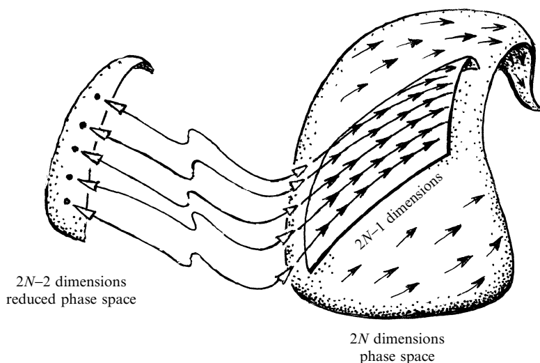
Fig. 20.8 Phase space T^*(C) is a 2N -dimensional symplectic manifold, for an N -dimensional C . For a given energy value (constant \mathcal{H} , as in Fig. 20.5), we have a (2N-1) -dimensional region containing a (2N-2) -dimensional family of the Hamiltonian flow trajectories. The reduced phase space, whose points represent these trajectories, is itself a 2(N-1) -dimensional symplectic manifold.
