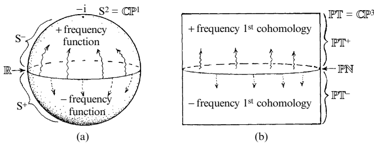
Fig. 33.22 An analogy between the Riemann sphere S^2 (= \mathbb{C}\mathbb{P}^1) and projective twistor space \mathbb{P}\mathbb{T} (= \mathbb{C}\mathbb{P}^3) . (a) A complex function (i.e. a '0th cohomology element'), defined on the real axis \mathbb{R} of S^2 , splits into its positive frequency part, extending holomorphically into what is here depicted as the northern hemisphere S^- , and its negative frequency part, extending into the southern hemisphere S^+ . (The Riemann sphere is here drawn so that \mathbb{R} is its equator, but so that -i is at the north pole and i at the south pole; compare Figs. 8.7 and 9.10, §9.5.) (b) A 1st cohomology element, defined on \mathbb{P}\mathbb{N} (and representing a massless field) splits into its positive frequency part, extending holomorphically into the top half \mathbb{P}\mathbb{T}^+ of projective twistor space, and its negative frequency part, extending into the bottom half \mathbb{P}\mathbb{T}^- .
