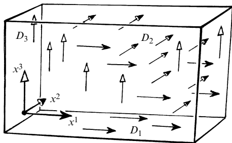
Fig. 21.1 In (affine) Euclidean N -space \mathbb{E}^N , there are N independent translational symmetries generated by the operators (vector fields) D_1 = \partial/\partial x^1, D_2 = \partial/\partial x^2, \dots, D_N = \partial/\partial x^N , satisfying commutation relations D_b x^a - x^a D_b = \delta_b^a with the respective Cartesian coordinates x^1, x^2, \dots, x^N . (The case N = 3 is illustrated.)
