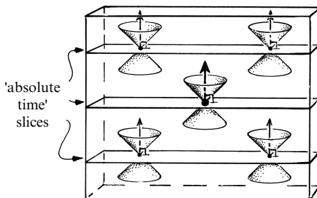
Fig. 17.13 A notion of absolute time introduced into \mathbb{M} would specify a family of \mathbb{E}^3 -slices cutting through \mathbb{M} and hence a local 3-plane-element at each event. But each null cone defines a (pseudo) metric \mathbf{g} , up to proportionality, whose notion of orthogonality thereby determines a state of rest.
