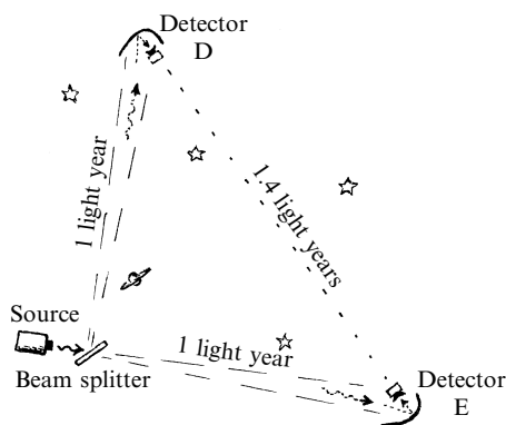
Fig. 21.8 A hypothetical space experiment illustrating the non-local nature of a wavefunction under measurement. The photon's wavefunction starts from the source as a neat little wave packet, but divides into two after encountering the beam-splitter, to arrive, after one year, at light-year distant detectors D and E. But just one of D or E can register the photon.
