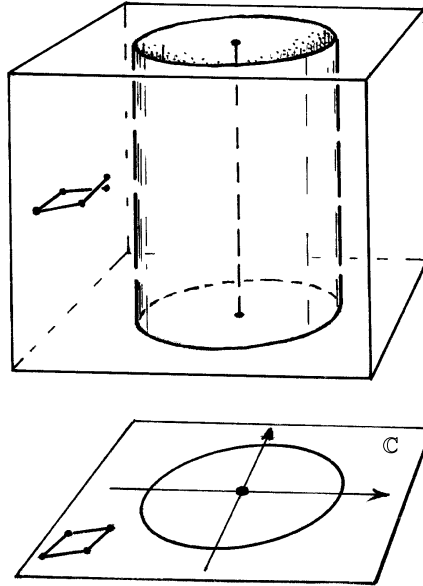
Fig. 15.19 To obtain a local path dependence (with curvature), in our bundle (now \mathcal{B}^{\mathbb{C}} ), we need at least 2 dimensions in the base \mathcal{M}^{\mathbb{C}} , now taken as the complex plane \mathbb{C} , where the S^1 of Fig. 15.16 is its unit circle. The fibres are to remain \mathbb{V}^1 (i.e. modelled on the real line \mathbb{R} ). Using z as a complex coordinate for \mathbb{C} = \mathcal{M}^{\mathbb{C}} , we use the explicit connection \nabla = \partial/\partial z - A , where A is a complex smooth function of z . When A is holomorphic the bundle curvature vanishes, but if A = ikz (with suitable k ), we get the strained bundle of Fig. 15.16 for the part over the unit circle. The bundle curvature is manifested in the failure to close of a horizontal polygon above a small parallelogram in \mathcal{M}^{\mathbb{C}} .
