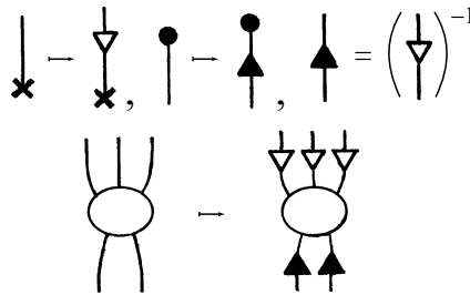
Fig. 13.13 The linear transformation x^a \mapsto T^a_b x^b , applied to \mathbf{x} in the vector space \mathbf{V} (with \mathbf{T} depicted as a white triangle), extends to the dual space \mathbf{V}^* by use of the inverse \mathbf{S} = \mathbf{T}^{-1} (depicted as a black triangle) and thence to the spaces \mathbf{V}^* \otimes \dots \otimes \mathbf{V}^* \otimes \mathbf{V} \otimes \dots \otimes \mathbf{V} of \begin{bmatrix} p \\ q \end{bmatrix} -valent tensors \mathcal{Q} . The case p = 3, q = 2 is illustrated, with \mathcal{Q} shown as an oval with three arms and two legs undergoing Q_{ab}{}^{cde} \propto S^{a'}_a S^{b'}_b T^c{}_{c'} T^d{}_{d'} T^e{}_{e'} Q_{a'b'}{}^{c'd'e'} .
