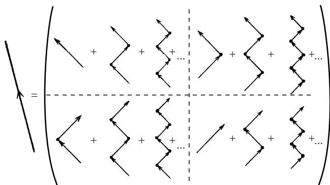
Fig. 25.2 Each zigzag process separately contributes, as part of an infinite quantum superposition, to the total ‘propagator’ in the manner of a Feynman graph. The conventional single-line Feynman propagator is drawn at the left, and it stands for the entire matrix of infinite sums of finite zigzags, drawn on the right.
