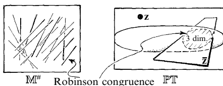
Fig. 33.14 We can obtain a ‘real’ picture of a non-null twistor Z^\alpha by first passing to its complex conjugate Z_\alpha , thus defining a complex projective plane in \mathbb{P}^T . This plane is fixed by its intersection with \mathbb{P}\mathbb{N} , which is a 3-real-dimensional locus. This locus defines a 3-parameter family of light rays in \mathbb{M}^\# called a Robinson congruence.
