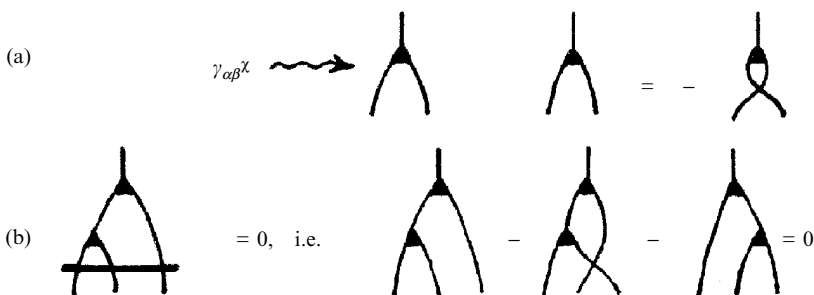
Fig. 13.11 (a) Structure constants \gamma_{\alpha\beta}{}^\lambda in diagrammatic form, depicting antisymmetry in \alpha , \beta and (b) the Jacobi identity.
