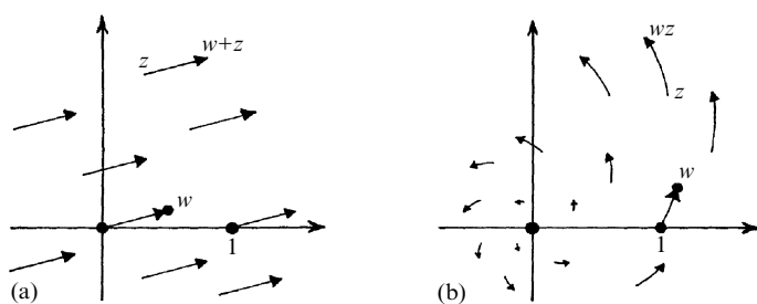
Fig. 5.2 (a) The addition map ‘ +w ’ provides a translation of the complex plane, sending 0 to w . (b) The multiplication map ‘ \times w ’ provides a rotation and expansion (or contraction) of the complex plane about 0 , sending 1 to w .
