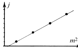
Fig. 31.6 Straight ‘Regge trajectories’ of particle resonances of increasing spin, plotted against mass squared. The elastic string picture provides an explanation.
