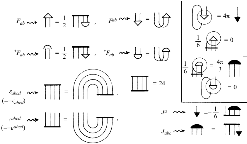
Fig. 19.1 Diagrams for Hodge duals and Maxwell equations. The quantities \epsilon_{abcd} ( =\epsilon_{[abcd]} ) and \epsilon^{abcd} ( =\epsilon^{[abcd]} ), normalized so that \epsilon_{0123} = \epsilon^{0123} = 1 in a standard Minkowski frame, are related to their raised/lowered versions (via g^{ab} and g_{ab} ) by \epsilon_{abcd} = -\epsilon^{abcd} and \epsilon^{abcd} = -\epsilon_{abcd} . In the diagrams (left middle, lower two lines) this sign change is absorbed by an effective index reversal. Boxed off to the top right are the Maxwell equations, first using the field tensor F (with its raised form F^{ab} = g^{ac}g^{bd}F_{cd} ; cf. Fig. 14.21) so the equations are \nabla_a F^{ab} = 4\pi J^b , \nabla_{[a} F_{bc]} = 0 , and beneath that, correspondingly using the dual *F (where *F_{ab} = \frac{1}{2}\epsilon_{abcd}F^{cd} , *J_{abc} = \epsilon_{abcd}J^d ) so the equations are \nabla_{[a} *F_{bc]} = \frac{4\pi}{3} *J_{abc} , \nabla_a *F^{ab} = 0 .
