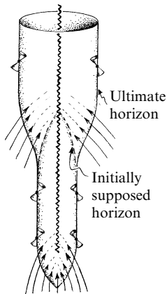
Fig. 30.15 The precise location of a black hole's horizon is determined 'teleologically', as it depends upon how much material ultimately falls into the hole.
