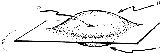
Fig. 20.9 Hamilton’s principle for field Lagrangians. The two fixed end-points a , b , in \mathcal{C} , of Fig. 20.3, represent field configurations in two 3-dimensional spacetime regions \mathcal{A} , \mathcal{B} , respectively—forming a ‘blister’ which encloses the 4-region \mathcal{D} . We may take \mathcal{A} and \mathcal{B} to come together, terminating at a finite 2-surface S (not drawn in the figure), or we may regard ‘ S ’ to be out at infinity, perhaps out along a spacelike hypersurface throughout which \mathcal{A} and \mathcal{B} coincide beyond the region \mathcal{D} (the case illustrated).
