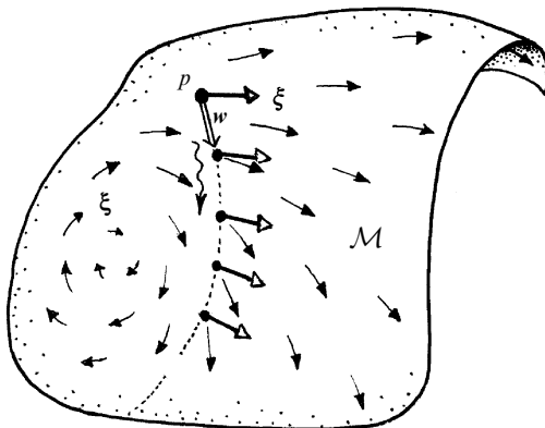
Fig. 14.5 The notion of covariant derivative can be understood in relation to parallel transport. The way in which a vector field \xi on M varies from point to point (black-headed arrows) is measured by its departure from that standard provided by parallel transport (white-headed arrows). This comparison can be made all along a curve \gamma , (starting at p ), but for the covariant first derivative \nabla_w at p we need to know only the tangent vector w to \gamma at p , which determines the covariant derivative \nabla_w \xi of \xi at p in the direction w .
