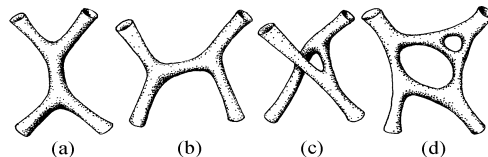
Fig. 31.5 The string-history picture of the respective processes of Fig. 31.4 provides an explanation of the equivalence between (a), (b), and (c), since they can be transformed into each other, as they are topologically the same. (d) Higher-order processes correspond to more complicated topology, where the topological genus corresponds to the number of loops (compare Fig. 8.9).
