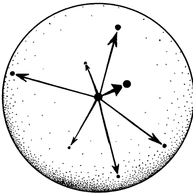
Fig. 22.14 Majorana’s description of the general (projective) spin state for a massive particle of spin \frac{n}{2} , given by n unordered points on the Riemann sphere. We can think of these vectors out from the centre to each of these points to be contributing spin \frac{1}{2} , in accordance with the prescription of Fig. 22.10. The symmetrical product of these spins gives the total. (In 2-spinor notation, the complete spin state is the symmetric n -valent spinor, which factorizes \psi_{AB\dots F} = \alpha_{(A}\beta_B \cdots \varphi_F) , where \alpha_A, \beta_A, \dots, \varphi_A , determine the n points, as in Fig. 22.10.)
