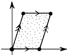
Fig. 8.10 To construct a Riemann surface of genus 1, take a region of the complex plane bounded by a parallelogram, vertices 0, 1, 1+p, p (cyclicly), with opposite edges identified. The quantity p provides a modulus for the Riemann surface.
