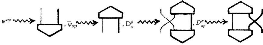
Fig. 29.5 Diagrammatic notation for density matrices constructed by ‘summing over unknown states’. The normalized ket-vector |\psi\rangle is expressed as \psi^{z\rho} , where ‘ \alpha ’ refers to ‘here’ (Earth) and ‘ \sigma ’ refers to ‘there’ (Titan). The Hermitian conjugate (bra-vector \langle\psi| ) is \bar{\psi}_{\alpha\rho} and the normalization is \bar{\psi}_{\alpha\rho}\psi^{z\rho} = 1 . The density matrix used ‘here’ is D^\beta_\alpha = \psi_{\alpha\rho}\psi^{\beta\rho} , while that used ‘there’ is \tilde{D}^\sigma_\rho = \bar{\psi}_{\alpha\rho}\psi^{\alpha\sigma} .
