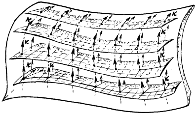
Fig. 30.3 Stationarity of a spacetime is expressed as the presence of a timelike Killing vector \kappa . This generates a continuous family of time-displacements preserving the metric. If \kappa = \partial/\partial t , where t is the ‘time parameter’ of a coordinate system (t, x, y, z) , then x , y , and z must be constant along the integral curves of \kappa . (See §14.7.)
