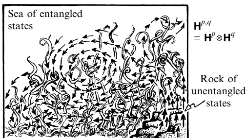
Fig. 23.6 Schrödinger evolution, away from an initial unentangled state (illustrated by the rock at the lower right) almost always leads to increasing entanglements (illustrated by the seaweed-strewn sea). So why do the ordinary objects of experience appear as separated independent things?
