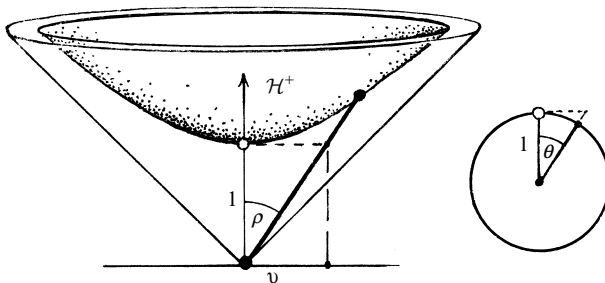
Fig. 18.11 Velocity space in relativity theory is the (unit) hyperbolic space \mathcal{H}^+ , where the rapidity \rho (= \tanh^{-1} v) measures hyperbolic distance along \mathcal{H}^+ (the speed of light c = 1 corresponding to infinite \rho ). This is analogous (by ‘signature flip’) to distance along a unit circle being the angle \theta subtended at its centre.
