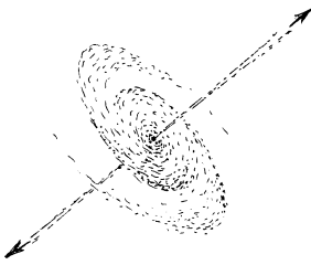
Fig. 30.13 The enormous energy output of a quasar appears to come from the rotational energy of a huge black hole at a galaxy's centre. This seems to be by a process of the general nature described in Fig. 30.12, but possibly mainly through the black hole swallowing electromagnetic fields of negative energy rather than particles.
