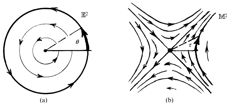
Fig. 30.5 Periodicity in imaginary time, illustrated by Minkowski 2-space \mathbb{M}^2 , complexified to \mathbb{C}\mathbb{M}^2 = \mathbb{C}\mathbb{E}^2 . (a) The Euclidean plane \mathbb{E}^2 is one real section of the complex space \mathbb{C}\mathbb{M}^2 . The Killing vector \partial/\partial\theta generates rotations in \mathbb{E}^2 , where we take polar coordinates (r, \theta) . Any function that is single-valued on \mathbb{E}^2 must be periodic in \theta with period 2\pi . (b) In the Lorentzian real section \mathbb{M}^2 of \mathbb{C}\mathbb{M}^2 , the ‘Rindler’ (uniform-acceleration) time coordinate is \tau = i\theta (an analogue of the Schwarzschild time that is natural for a black hole), and a function that is analytic at the origin O must have an imaginary period in \tau , with period 2\pi i . (Killing vector \kappa = \partial/\partial\tau = -i\partial/\partial\theta .)
