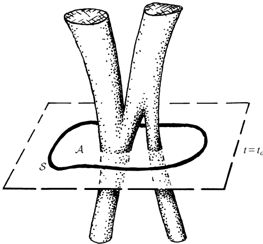
Fig. 19.4 Within the 3-surface of constant time t = t_0 , Maxwell’s d^*F = 4\pi^*J gives us the Gauss law, whereby the integral of electric flux (integral of ^*F ) over a closed spatial 2-surface measures the total charge surrounded (by the fundamental theorem of exterior calculus). In fact, this is not restricted to 2-surfaces at constant time, and the Gauss law is thereby generalized.
