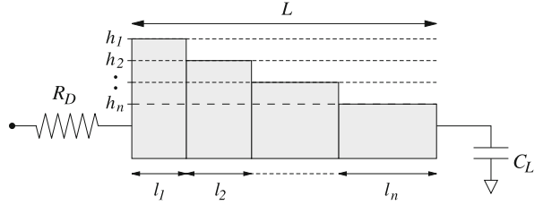
Wire Sizing, Figure 3 Illustration of the simplified wire sizing problem
