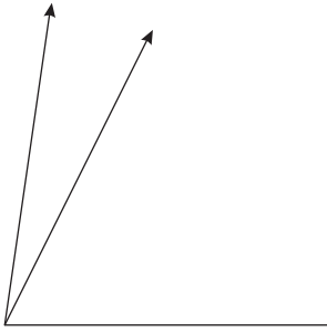
Adjacent angle
