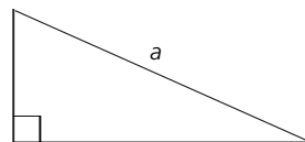
Hypotenuse
