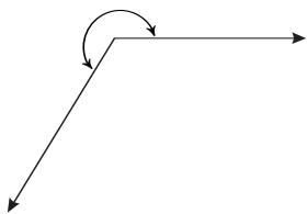
Reflex angle
