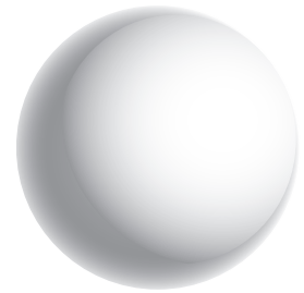
Sphere
