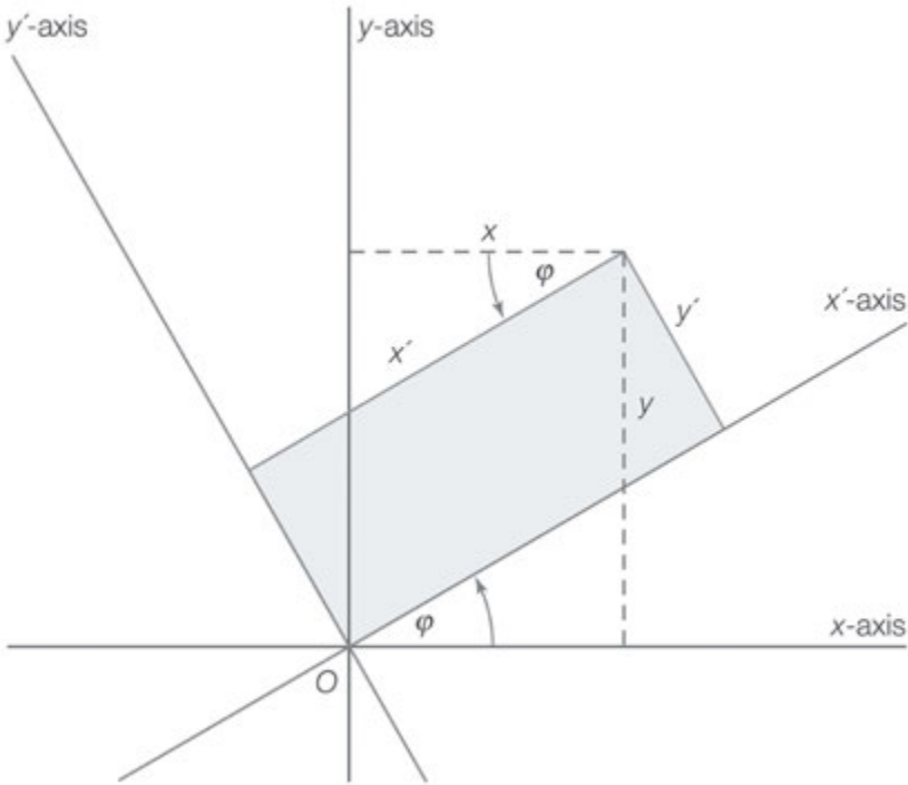
Rotating the coordinate axes through an angle \phi changes the coordinates of a point from (x, y) to (x', y') . Encyclopædia Britannica, Inc.
