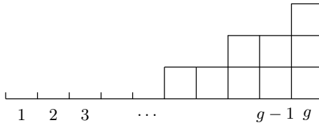
Fig. 1. Young diagram with \xi = \{5, 3, 1\} .
