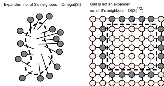
Figure 16.3: In a combinatorial expander , every subset S of the vertices that is not too big has at least \Omega(|S|) neighbors outside the set. The grid (and every other planar graph) is not a combinatorial expander as a k \times k square in the grid has only O(k) neighbors outside it.
