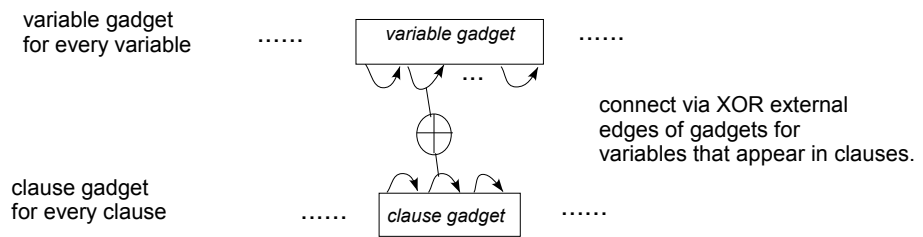
Figure 8.3: The gadgets used in the proof of Valiant's Theorem. Web draft 2006-09-28 18:09
