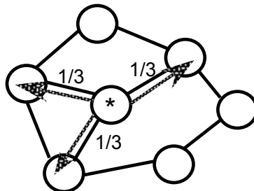
Figure 16.1: A random walk on a graph can be thought of as placing a token on some vertex, and at each step move the token to random neighbor of its current location.
