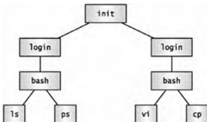
Figure 7.4: Linux processes have parents, leading back to init , the first program the Linux kernel runs.
