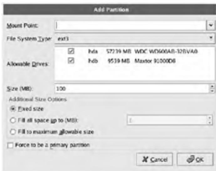
Figure 2.5: You specify critical partition information in a single dialog box.
