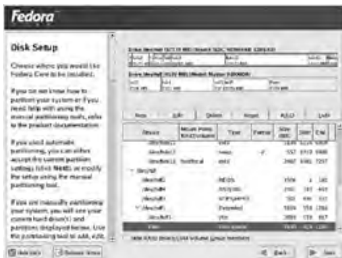
Figure 2.4: Fedora's Disk Druid lets you point at free space or partitions and click options to create or modify partitions.
