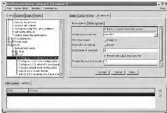
Figure 6.5: GUI administration tools categorize administration tasks and provide point-and-click interfaces to the underlying utilities.
