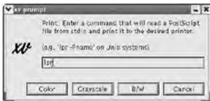
Figure 9.1: Some Linux printing dialog boxes require the user to know the printer's name, which can be intimidating.
