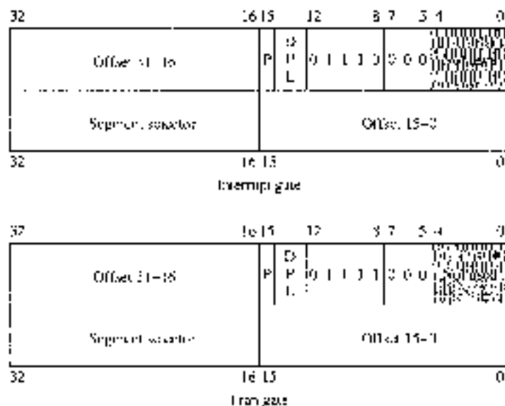
Figure 20.3 The IA 32-bit interrupt descriptors.
