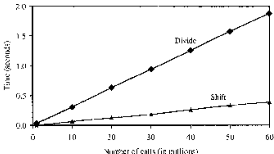
Figure 18.1 Execution time comparison of implementing division by a power of 2 using the shift and divide instructions.
