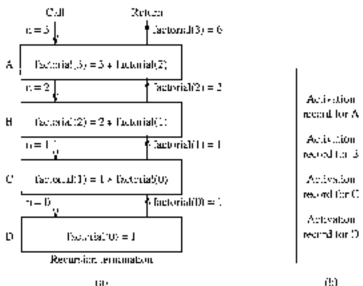
Figure 19.1 Recursive computation of \text{factorial}(3) .
