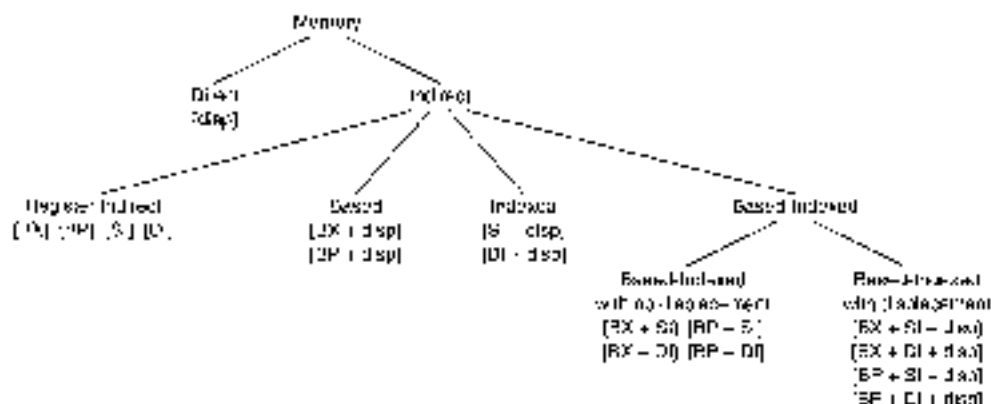
Figure 13.1 Memory addressing modes for 16-bit addresses.
