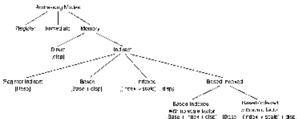
Figure 13.2 Addressing modes of the Pentium for 32-bit addresses.
