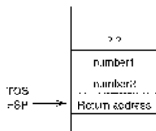
Figure 11.7 Stack state after the sum procedure call: Return address is the ESP value pushed on to the stack as part of executing the call instruction.
