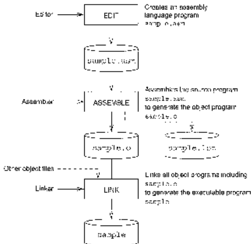
Figure 7.2 Assembling and linking assembly language programs (input and output are shown by dashed lines).
