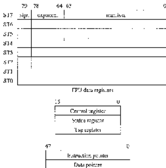
Figure 22.1 FPU registers.
