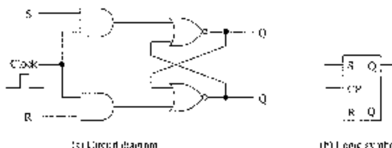
Figure 2.28 Clockless SR latch.
