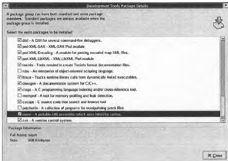
Figure 5.41 Adding the nasm and ddd packages.
