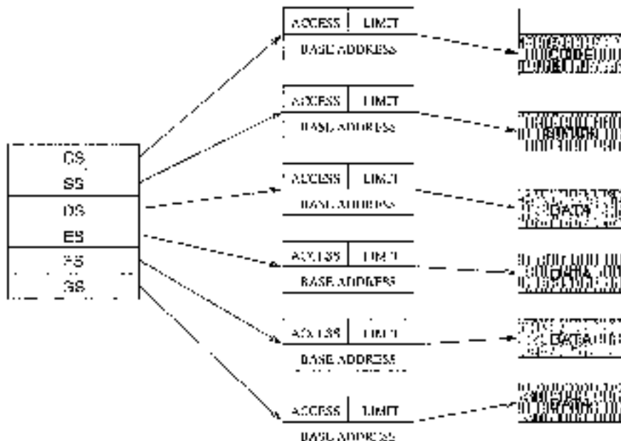
Figure 4.10 Segments in a multi-segment model.
