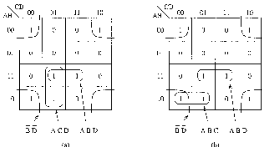
Figure 2.9 Different minimal expressions will result depending on the groupings.
