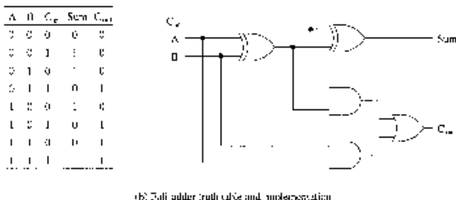
Figure 2.16 Full- and half-adder truth tables and implementations.
