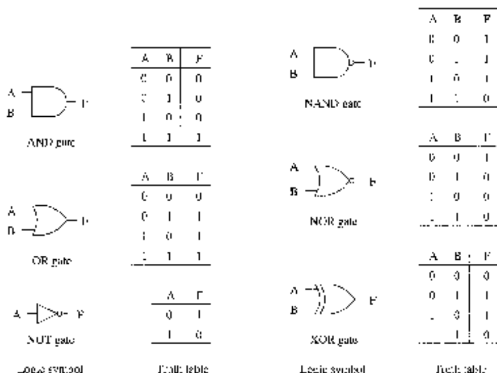
(a) Basic logic gates
