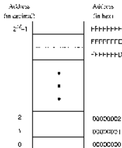
Figure 3.1 Log-off view of the system memory.
