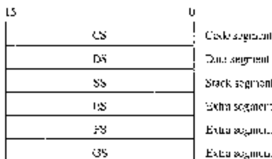
Figure 4.5 The six segment registers support the segmented memory architecture
