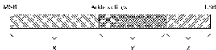
Figure 3.7 Address line partitioning.
