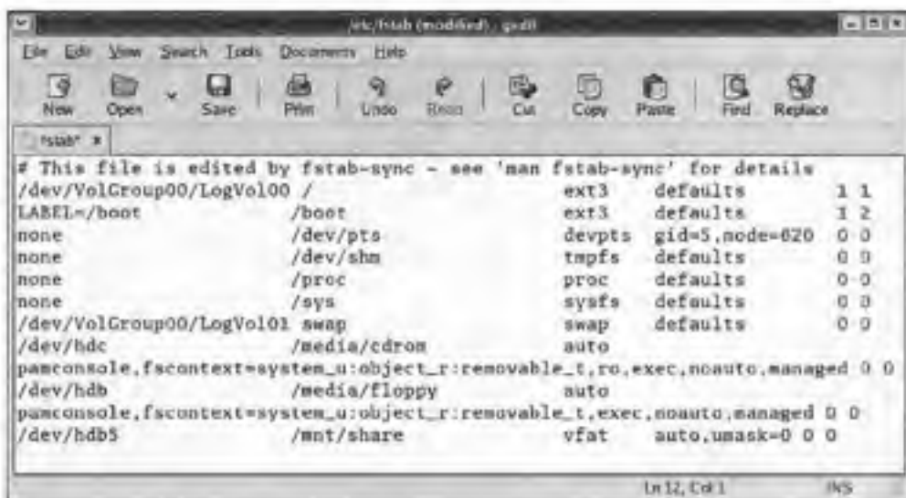
Figure 5.44 Contents of the /etc/fstab file after adding the last line to mount the shared partition.
