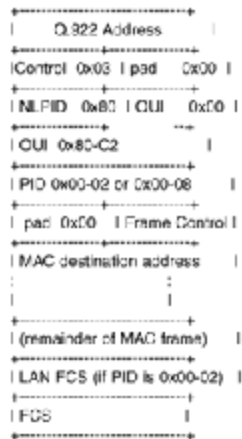
Figure 22-6 Format of bridged Ethernet/802.3 frame.
