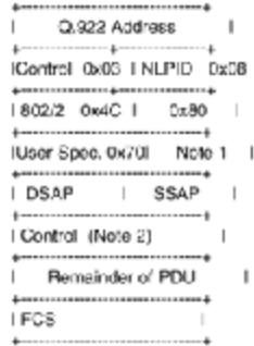
Figure 22-23 ISO 8802/2 with user-specified layer 3.
