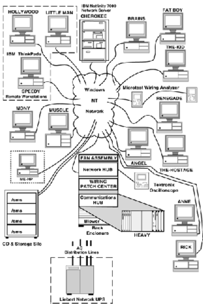
Figure 16-12 Liebert UPS for the network.
