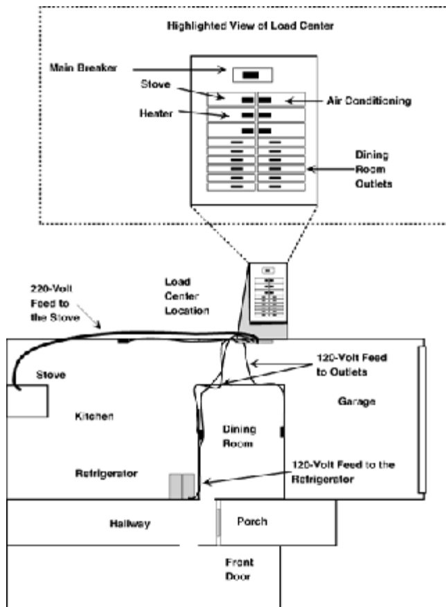
Figure 16-6 Overview of house wiring.
