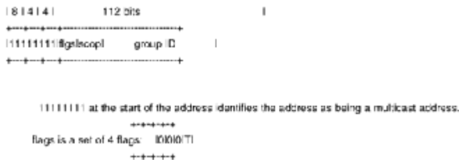
Figure 10-30 IPv6 multicast address format.
