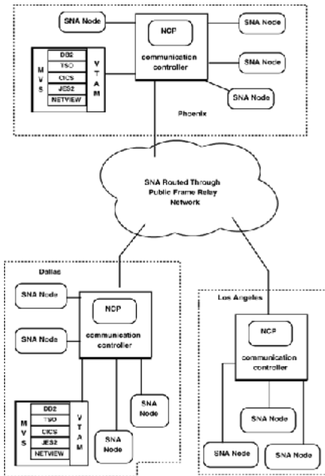
Figure 23-5 SNA routed through public frame-relay network.
