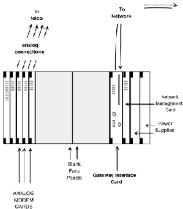
Figure 18-23 Network hub analog functionality.
