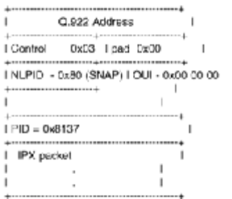
Figure 22-19 Encapsulation of IPX packet by SNAP header.
