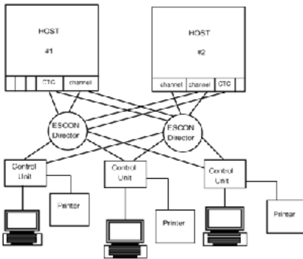
Figure 2-2 ESCON configuration.
