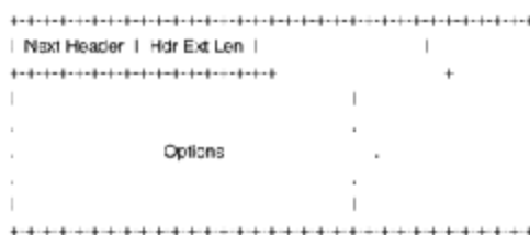
Figure 10-13 IPv6 destination options header.
