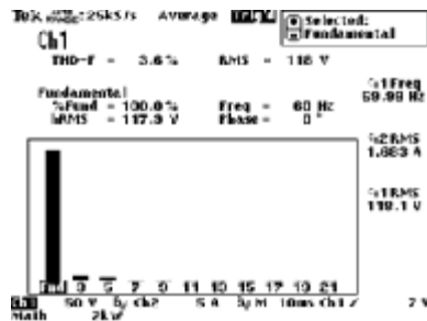
Figure 16-11 Odd harmonics.
