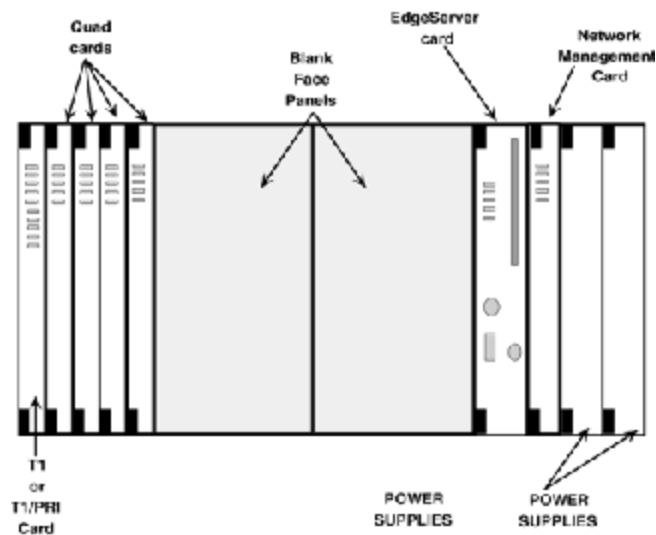
Figure 17-11 Enterprise Network hub.
