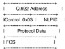
Figure 22-4 Format of routed NLPID protocol.
