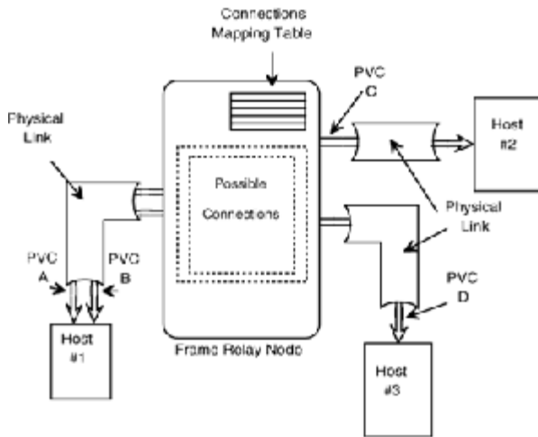
Figure 23-6 Enhanced view of a frame-relay node.
