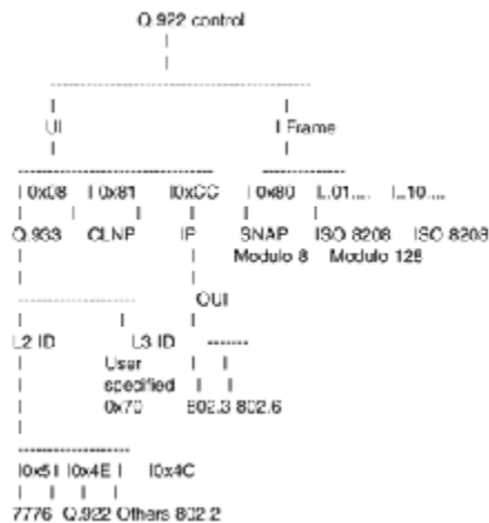
Figure 22-21 A generic encapsulation technique.
