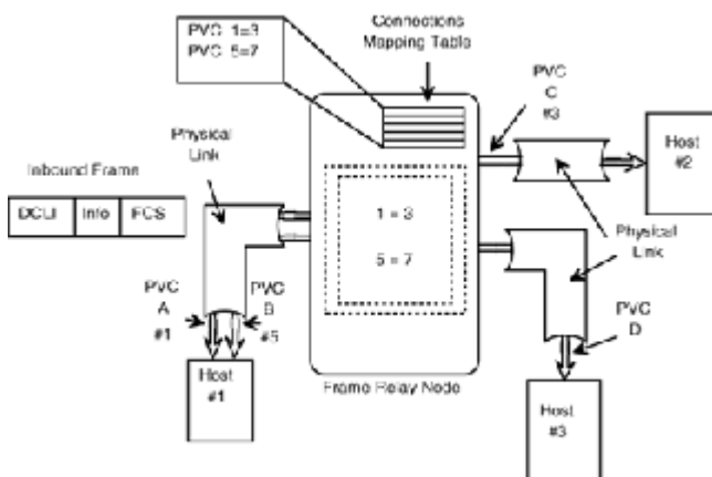
Figure 23-7 Highlighted view of the mapping table.
