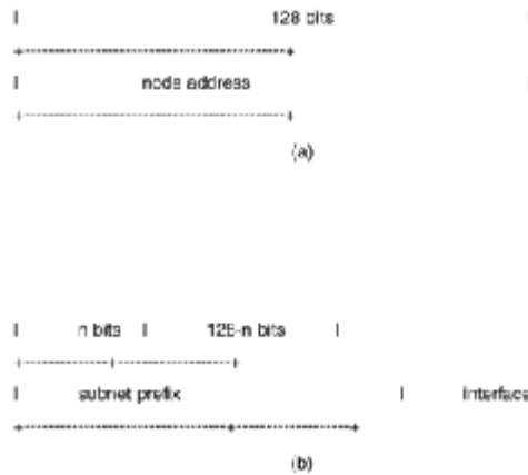
Figure 10-20 IPv6 nodes: (a) simple host. (b) slightly sophisticated host.
