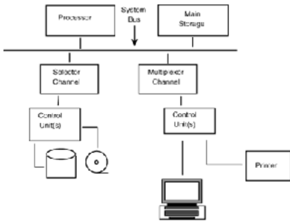
Figure 1-1 Logical view of an S/360.
