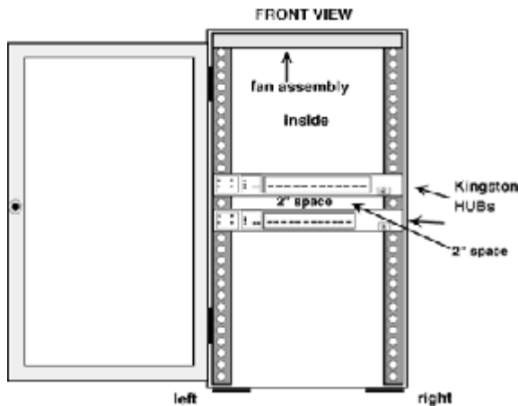
Figure 18-25 Kingston network hubs (front view).
