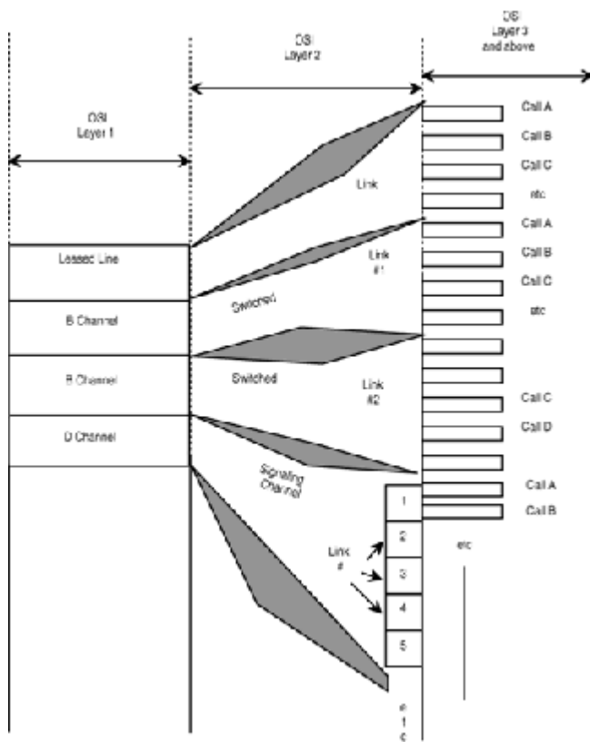
Figure 24-14 Conceptual view of ISDN B and D channels.
