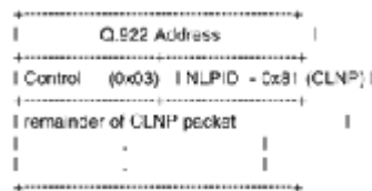
Figure 22-18 CLNP data packet identified "by NLPID.
