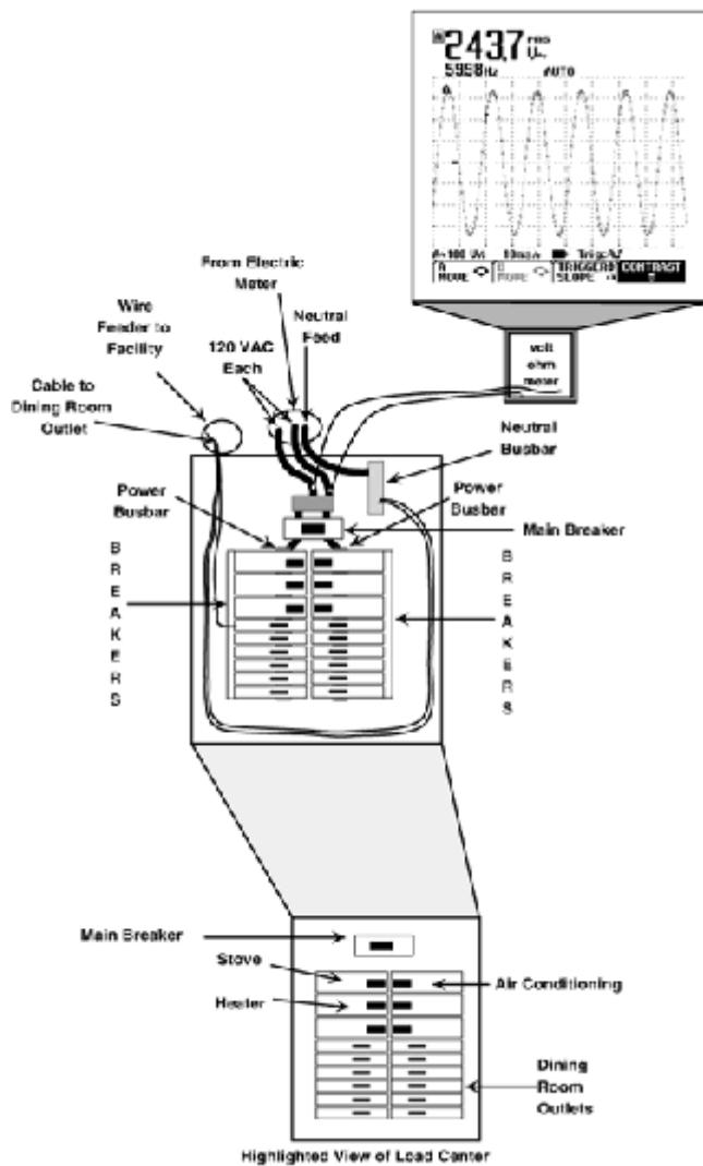
Figure 16-8 Voltage reading from electric meter.
