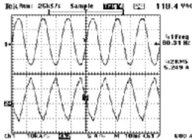
Figure 18-37 Amperage and voltage readings on power-on.
