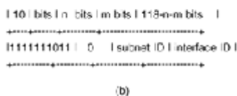
Figure 10-28 Local-use unicast addresses: (a) link-local and (b) site-local.
