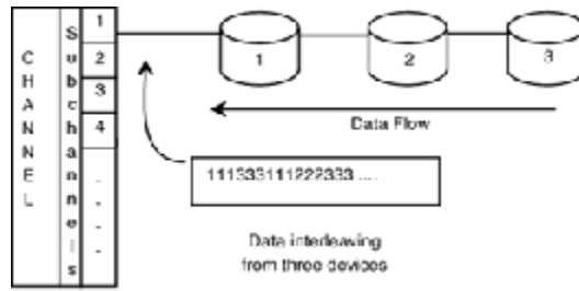
Figure 2-5 Data flow through a block multiplexer channel.
