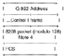
Figure 22-25 Format of ISO 8208 frame modulo 128.
