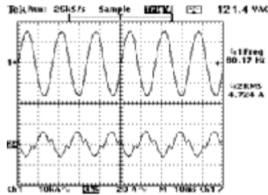
Figure 16-2 Microwave oven voltage and current readings upon initial power-on.
