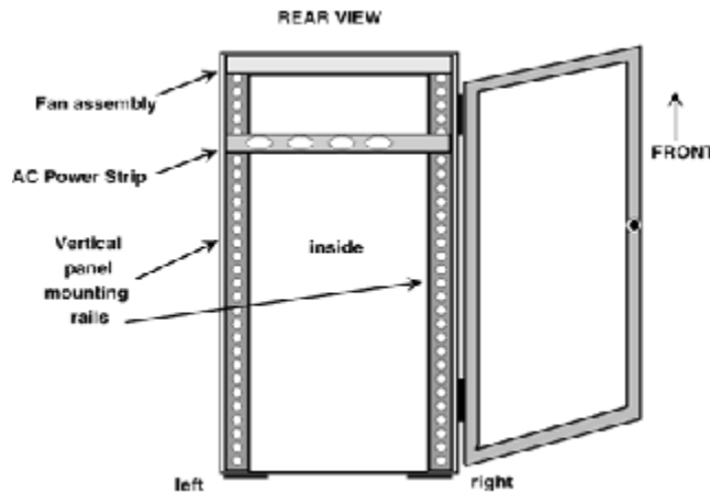
Figure 18-15 Network rack enclosure (rear view).
