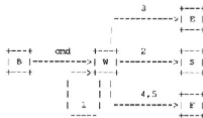
Figure 15-9 FTP commands state diagram.
