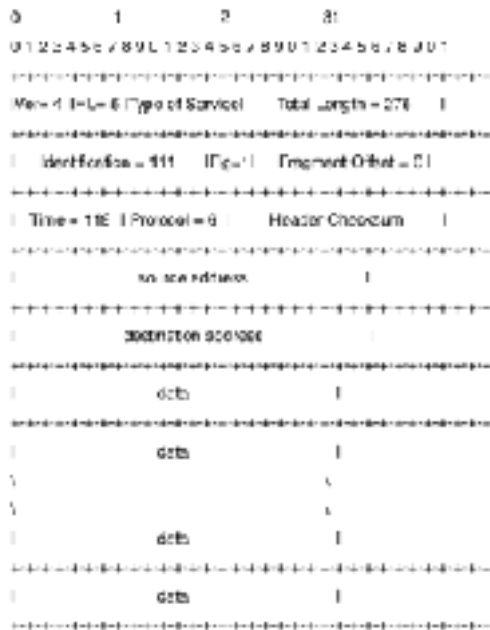
Figure 9-16 IPv4 second datagram fragment.
