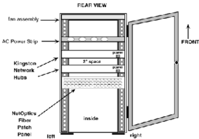
Figure 18-27 NetOptics fiber patch panel.
