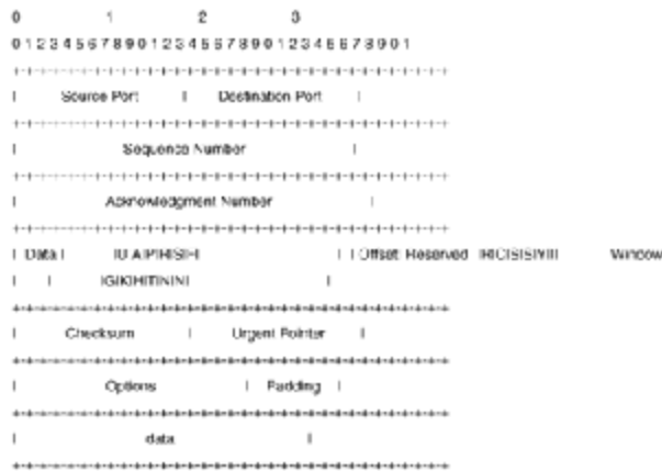
Figure 11-1 TCP header format.
