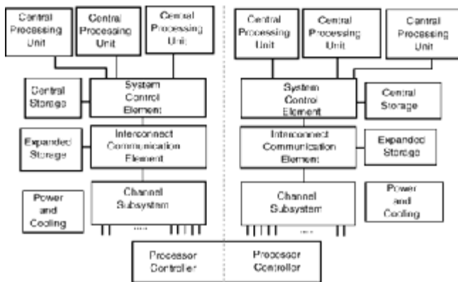
Figure 2-1 A conceptual view of a partitioned ES/9000.
