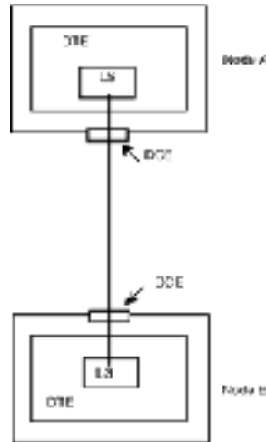
Figure 5-7 Conceptual view of a link station.
