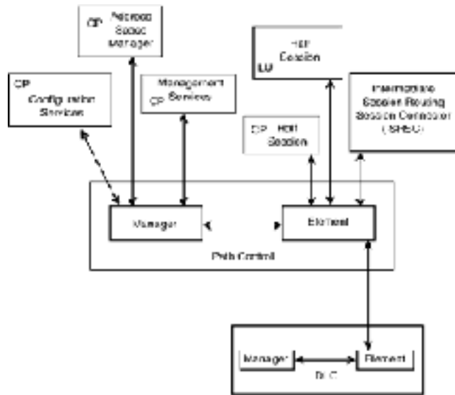
Figure 6-15 Relationship between PC, CP, and session establishment.
