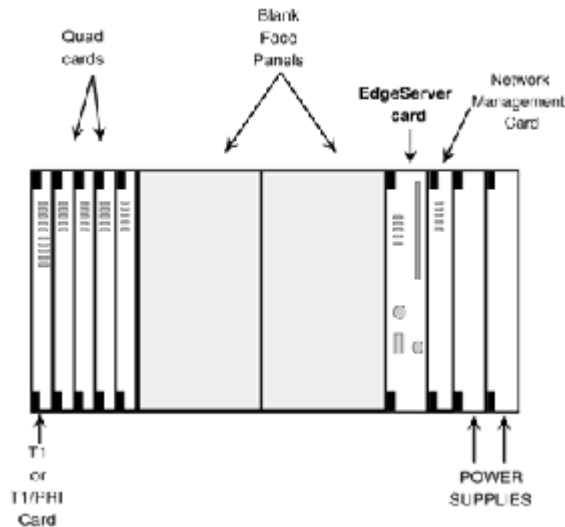
Figure 18-21 Network hub.
