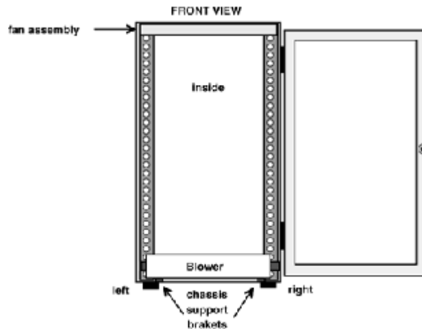
Figure 17-2 Great Lakes cabinet front view.
