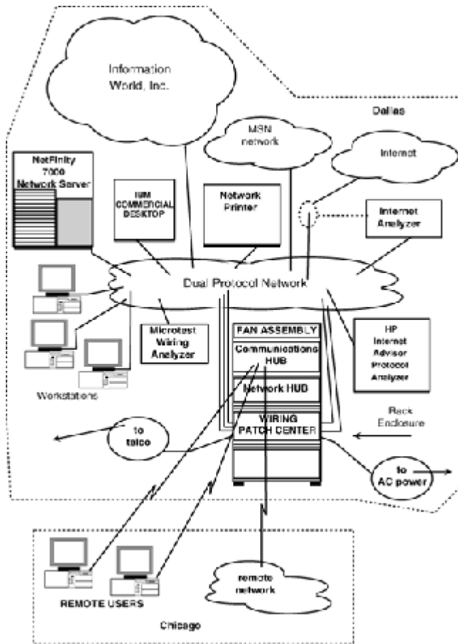
Figure 18-19 Data-communications hub.
