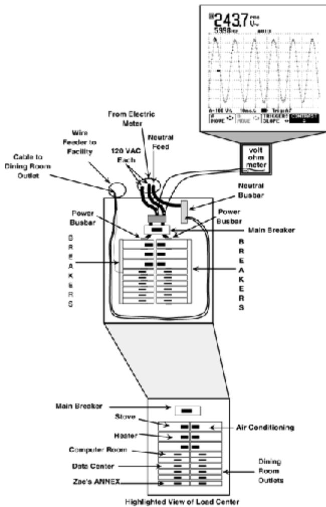
Figure 18-31 Highlighted view of a different perspective of the electrical infrastructure.
