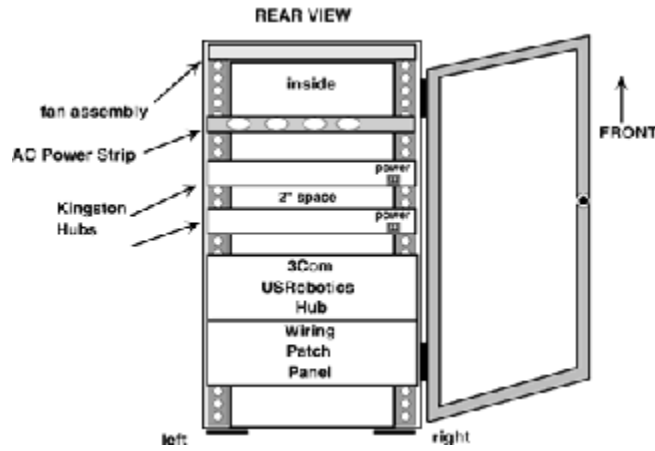
Figure 18-26 Kingston hubs (rear view).
