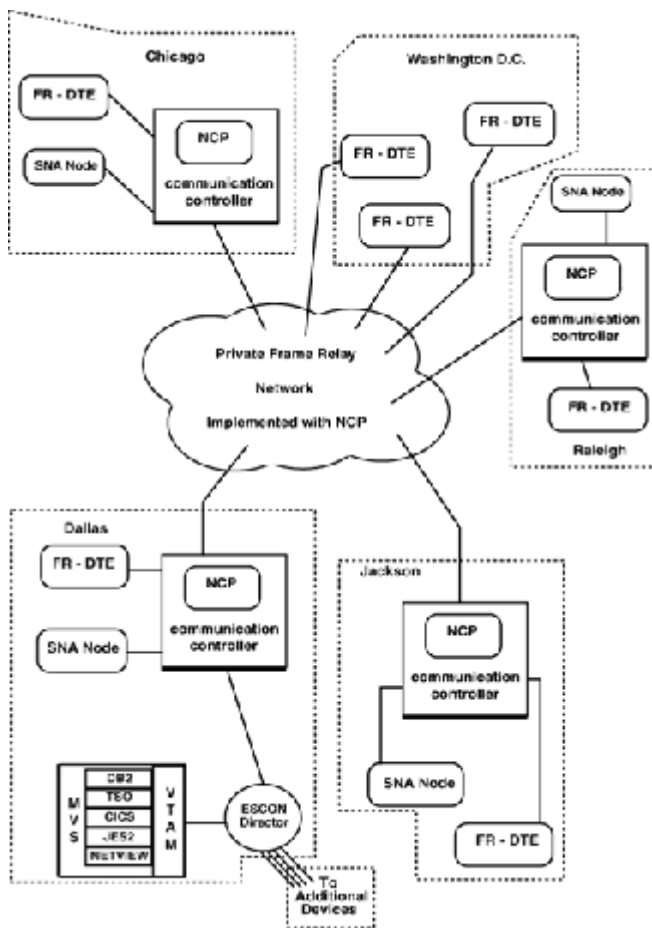
Figure 23-3 Private SNA—frame-relay network.
