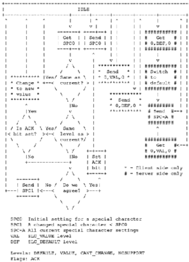
Figure 13.1 State diagram for SLC.
