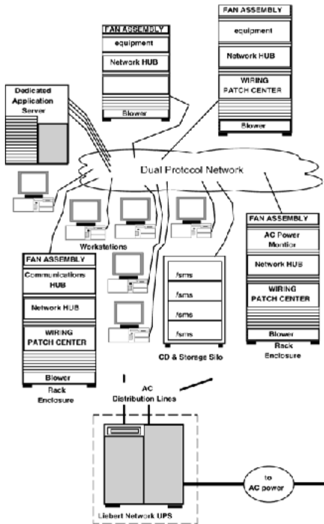
Figure 18-16 Conceptual view of network with cabinets.
