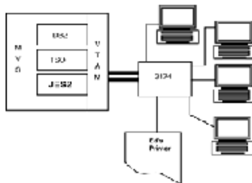
Figure 4-5 The JES2.
