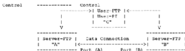
Figure 15-2 Server-server interaction.
