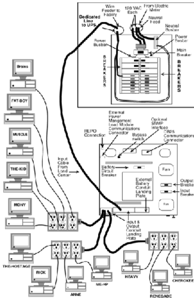
Figure 18-30 Conceptual view of the electrical infrastructure.
