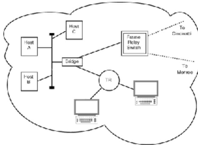
Figure 23-11 Focused view of FRAD equipment.
