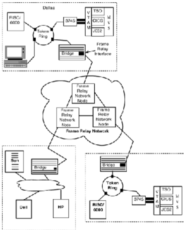
Figure 23-1 Conceptual view of frame relay.
