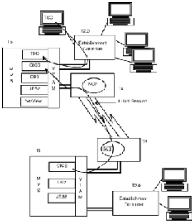
Figure 5-6 Conceptual view of a typical SNA network.
