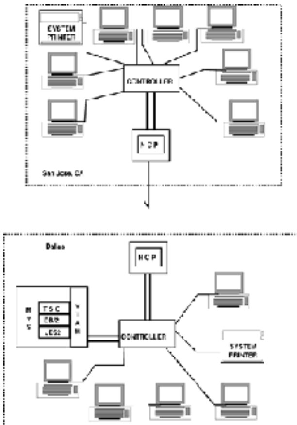
Figure 5-15 SNA blueprint 3.
