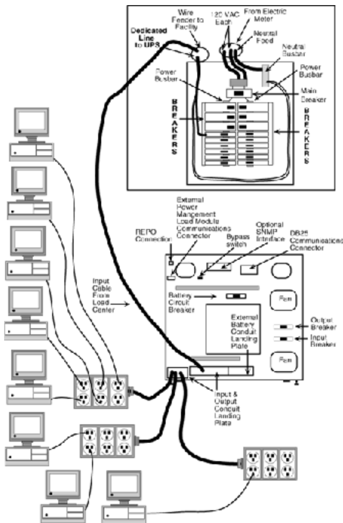
Figure 16-14 Conceptual view of ac supply.
