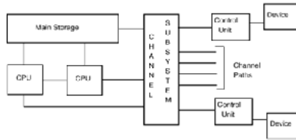
Figure 1-9 ESA/370 architecture.
