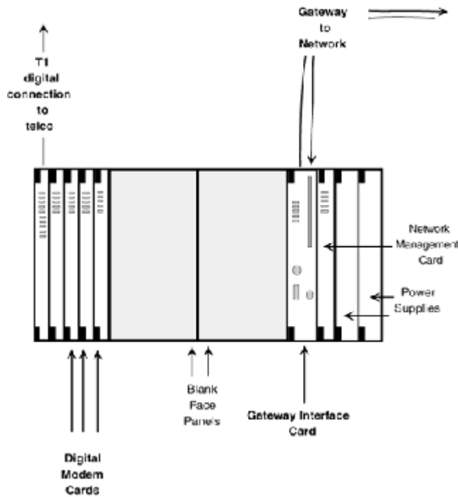
Figure 18-24 Network hub digital functionality.
