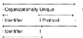
Figure 22-2 SNAP header.
