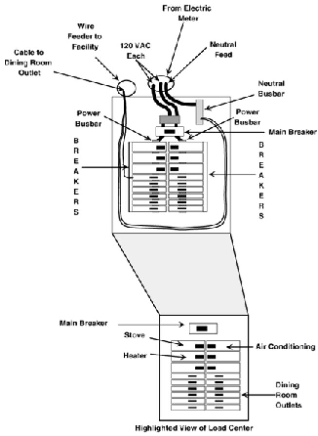
Figure 16-7 Detailed view inside load center.
