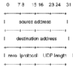
Figure 12-1 UDP pseudoheader.
