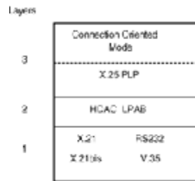
Figure 24-4 X.25 layers.
