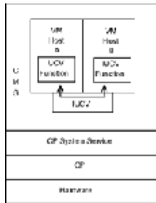
Figure 3-3 IUCV communications.
