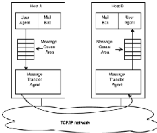
Figure 8-6 SMTP components.
