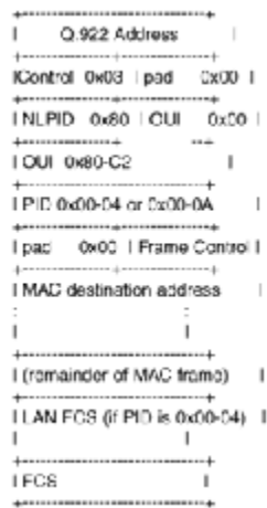
Figure 22-9 Format of bridged FDDI frame.
