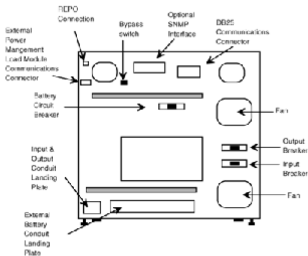
Figure 16-13 Liebert UPS rear view.
