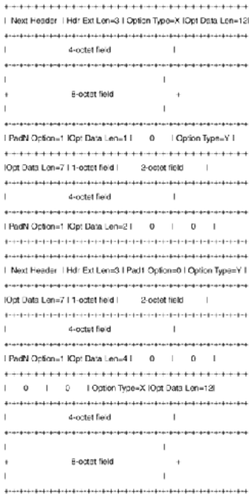
Figure 10-19 Hop-by-hop head for both options X and Y.
