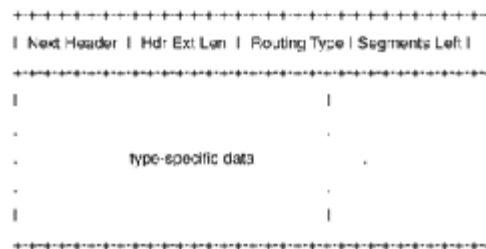
Figure 10-7 IPv6 routing header.
