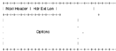
Figure 10-14 IPv6 TCP and UDP “pseudoheader.”
