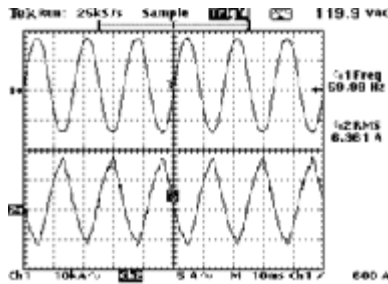
Figure 18-38 Amperage and voltage readings with drum heating.
