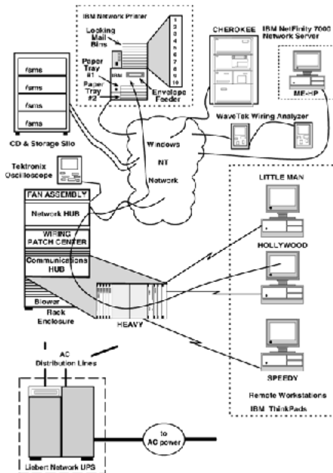
Figure 18-35 Remote users using the network printer.
