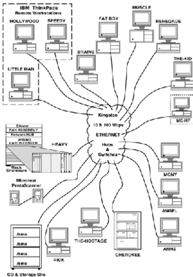
Figure 17-4 Logical view of Kingston hub and switch implementation.
