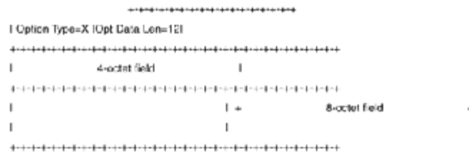
Figure 10-15 Option X with two data fields.
