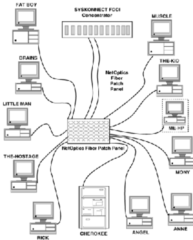
Figure 17-13 SysKonnnect Concentrator.
