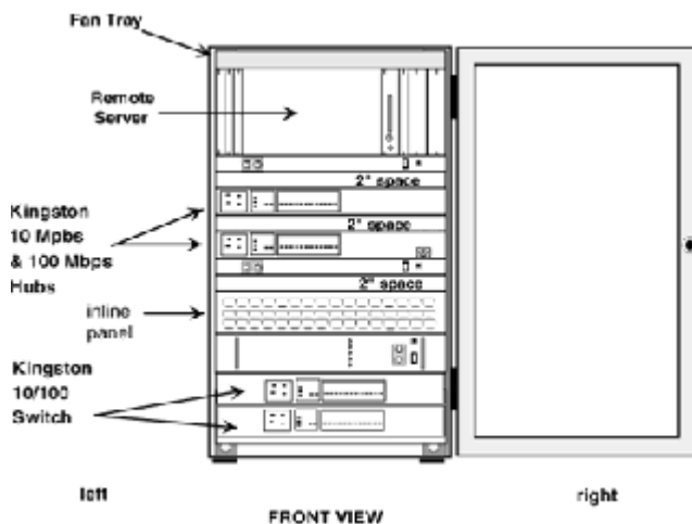
Figure 17-3 Kingston hubs and switches.
