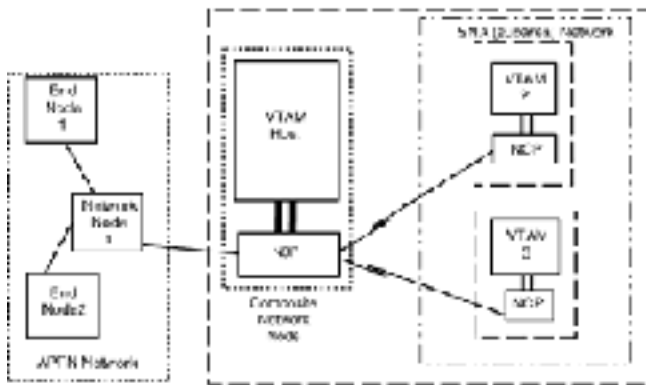
Figure 6-25 A mixed APPN-SNA network.
