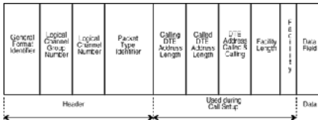
Figure 24-8 Example of an X.25 call setup packet.
